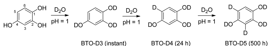
Figure 1. (a) Decomposition of BTO (TCI) in D 2 O (0.125 M) as a function of time under different conditions (acidic: pH 1, basic: pH 10) monitored by 1 H NMR via the signal of the 5-Ar-H compared with an internal standard. (For the illustration, lines are added, obtained through fitting a second-order exponential decay.) (b) Series of 1 H NMR spectra of BTO in acidic (H 2 SO 4 ) D 2 O. Relative decrease in different signal integrals compared with integrals at t 0 for different aromatic protons of (c) BTO and (d) 1. (e) Repeat of spectra series of BTO (Aldrich) in acid (H 2 SO 4 ) and D 2 O on a short time scale. (f) Relative decrease in different signal integrals compared with integrals at t 0 for different aromatic protons of BTO on a shorter time scale.
