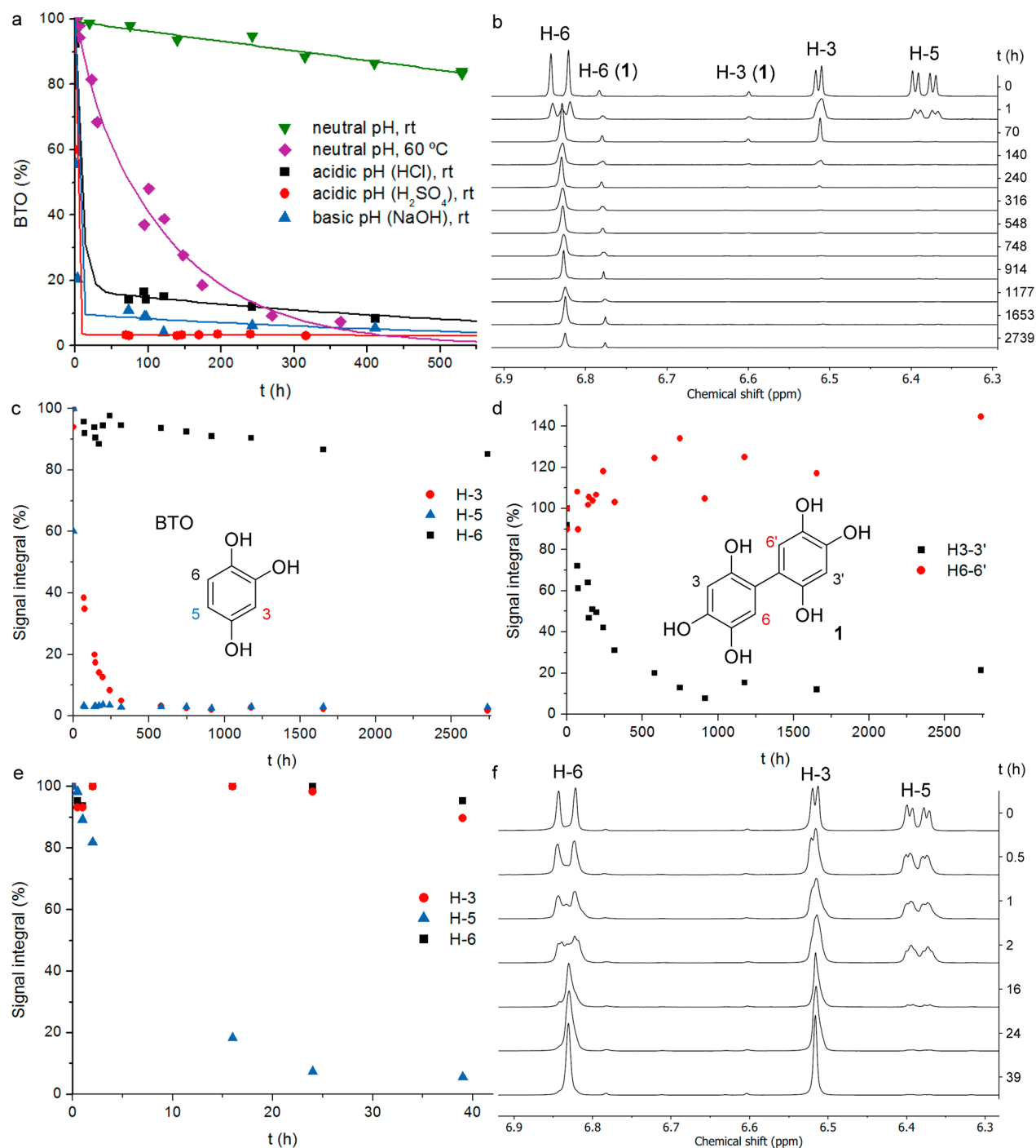
Figure 1. (a) Decomposition of BTO (TCI) in D 2 O (0.125 M) as a function of time under different conditions (acidic: pH 1, basic: pH 10) monitored by 1 H NMR via the signal of the 5-Ar-H compared with an internal standard. (For the illustration, lines are added, obtained through fitting a second-order exponential decay.) (b) Series of 1 H NMR spectra of BTO in acidic (H 2 SO 4 ) D 2 O. Relative decrease in different signal integrals compared with integrals at t 0 for different aromatic protons of (c) BTO and (d) 1. (e) Repeat of spectra series of BTO (Aldrich) in acid (H 2 SO 4 ) and D 2 O on a short time scale. (f) Relative decrease in different signal integrals compared with integrals at t 0 for different aromatic protons of BTO on a shorter time scale.
