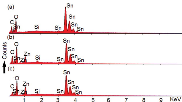
Fig. 3 Energy-dispersive X-ray spectra of (a) undoped, (b) Sn 0.96 Zn 0.04 O 2 and (c) Sn 0.90 Zn 0.10 O 2 nanoparticles.
