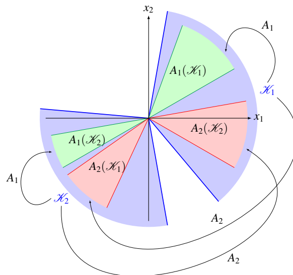
Figure 1: If A_1 and A_2 are linear operators that map the cones \mathcal{K}_1 and \mathcal{K}_2 as shown on the figure above, then the switching linear system defined by \{A_1, A_2\} is path-complete positive w.r.t. the set of cones \{\mathcal{K}_1, \mathcal{K}_2\} .
