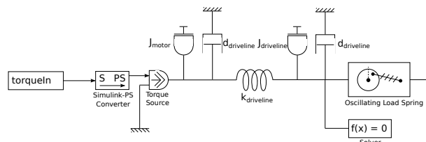
Figure 1: SimScape model
