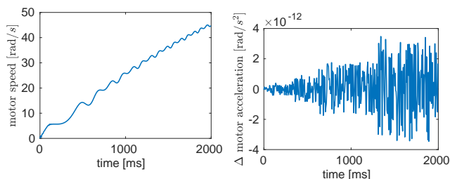
Figure 2: SimScape simulation
