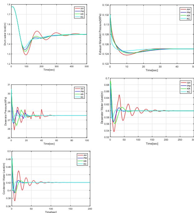
Figure 1: System outputs with different PID controllers
