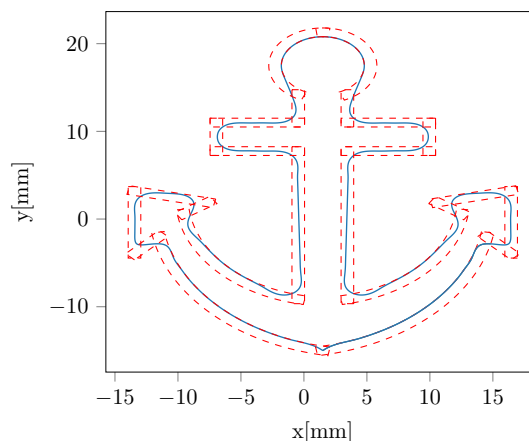
Figure 1: Anchor-shaped workpiece - machine tool trajectories
