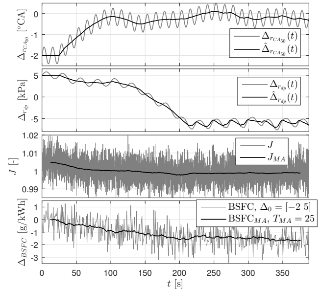
Figure 3: ES inputs \Delta_{r_{CA_{50}}} , \Delta_{r_{dp}} , cost J and BSFC saving \Delta_{BSFC} , and their moving averages J_{MA} , \Delta_{BSFC_{MA}} .
