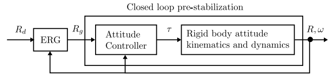
Figure 2: Control scheme
