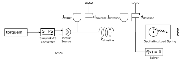
Figure 1: SimScape model
