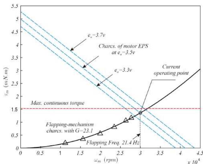
Figure 2: Torque versus rotation speed of the motor, for various voltages, and measured torque requirements of the mechanism for a gear ratio of G = 23.1 : 1 . The crossing of the two curves is the operating point of the mechanism.
