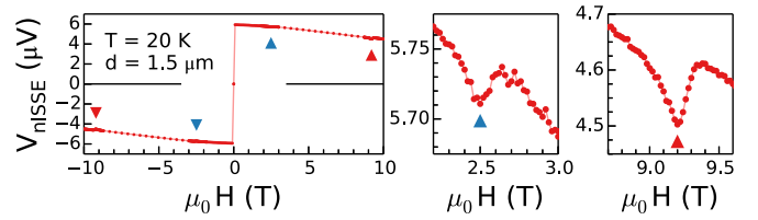
FIG. 8. nISSE measurements over an extended magnetic field range. In addition to the resonant suppression of V_{\text{nISSE}} at H_{TA} , a second resonance due to the hybridization of magnons with phonons in the longitudinal acoustic mode can be seen in the data at higher magnetic field amplitude. The smaller panels show a close-up of the data around H = H_{TA} and H = H_{LA} . Data obtained from sample S1.
