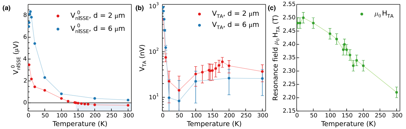
FIG. 5. (a) Temperature dependence of the low-field V_{\text{nlsSE}}^0 , for d = 2 and 6 \mu\text{m} . For 2 \mu\text{m} , the signal changes sign around T = 143 K. The blue shading in the graph indicates the regime in which the sign agrees with that of the hiSSE. (b) Temperature dependence of the magnon-polaron resonance V_{\text{TA}} . Here, no sign change but a minimum around T = 50 K is observed, which is absent in (a). (c) Temperature dependence of the resonance field H_{\text{TA}} . The maximum around T = 25 K is likely an artifact resulting from our measurement uncertainty, since it falls within the error bars and no such maximum was observed for the hiSSE measurements [9]. Error bars in (b) and (c) reflect the peak-to-peak noise in the data used to extract V_{\text{TA}} and the step size in the magnetic field scans ( \mu_0 \Delta H = 20 mT), respectively.
