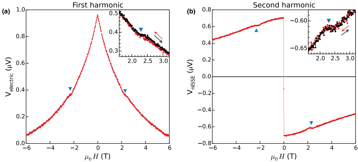
FIG. 3. (a) Nonlocal voltage generated by magnons that are excited electrically (first harmonic response to an oscillating current in the injector contact). An anomaly is observed at |H| = H_{TA} (the field that satisfies the touching condition for magnons and transverse acoustic phonons). The inset shows a second set of data from the same sample, taken with a higher magnetic field resolution ( \mu_0 \Delta H = 15 mT), sweeping the magnetic field both in the forward (black) and backward (red) directions. (b) nISSE voltage (second harmonic response) for the same device. V_{nISSE} is suppressed at |H| = H_{TA} . The inset shows the corresponding second harmonic data of the high resolution field sweep. The results were obtained on sample G1 (thickness 210 nm) with d = 3.5 \mu\text{m} and I = 150 \mu\text{A}_{\text{rms}} , at room temperature. A constant background voltage V_{bg} = 575 nV was subtracted from the data in Fig. (a).
