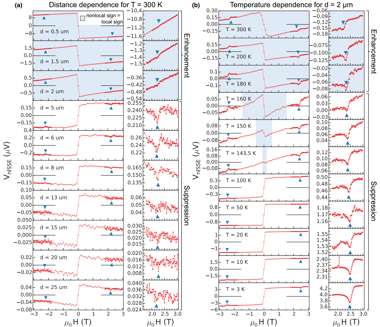
FIG. 4. (a) V_{\text{nISSE}} vs H for various injector-detector separations at T = 300\text{ K} . (b) V_{\text{nISSE}} vs H for different temperatures and d = 2\ \mu\text{m} . The data in (a) and (b) are from sample S1 and S2, respectively, and is the average of a forward and backward magnetic field sweep. (The voltage shown is given by V_{H+} = [V_{\text{backward}}(H) - V_{\text{backward}}(-H)]/2 and V_{H-} = [V_{\text{forward}}(H) - V_{\text{forward}}(-H)]/2 , where V_{H+} is the voltage at positive magnetic field values and V_{H-} that at negative magnetic field values.) The magnon-polaron resonance is indicated by the blue arrows. The blue shading in the graphs indicates the region in which the sign of the nISSE signal agrees with that of the hiSSE. The right column in both (a) and (b) shows close-ups of the data around the positive resonance field (blue triangles). The data in the close-ups has been antisymmetrized with respect to H , i.e., V = [V(+H) - V(-H)]/2 . (a) shows that when the contacts are close ( d \leq 2\ \mu\text{m} ), the magnon-polaron resonance enhances V_{\text{nISSE}} , while for long distances V_{\text{nISSE}} is suppressed at the resonance magnetic field. For very large distances ( d \geq 20\ \mu\text{m} ), the resonance cannot be observed anymore. Similarly in (b), for temperatures T \geq 180\text{ K} , the magnon-polaron resonance enhances the nISSE signal, while for lower temperatures the nISSE signal is suppressed. The excitation current I = 100\ \mu\text{A}_{\text{rms}} for all measurements.
