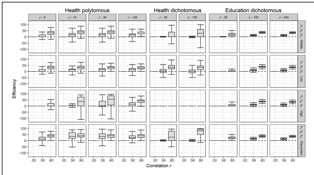
Figure 6. Relative efficiency gain associated with MCAT. Note. Positive and negative values indicate gain and loss percentages in efficiency on the UCAT test length scale, respectively. MCAT = multidimensional CAT; UCAT = unidimensional CAT.
