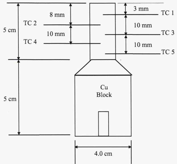
Fig. 3 Copper block schematic with TC locations (not to scale)
