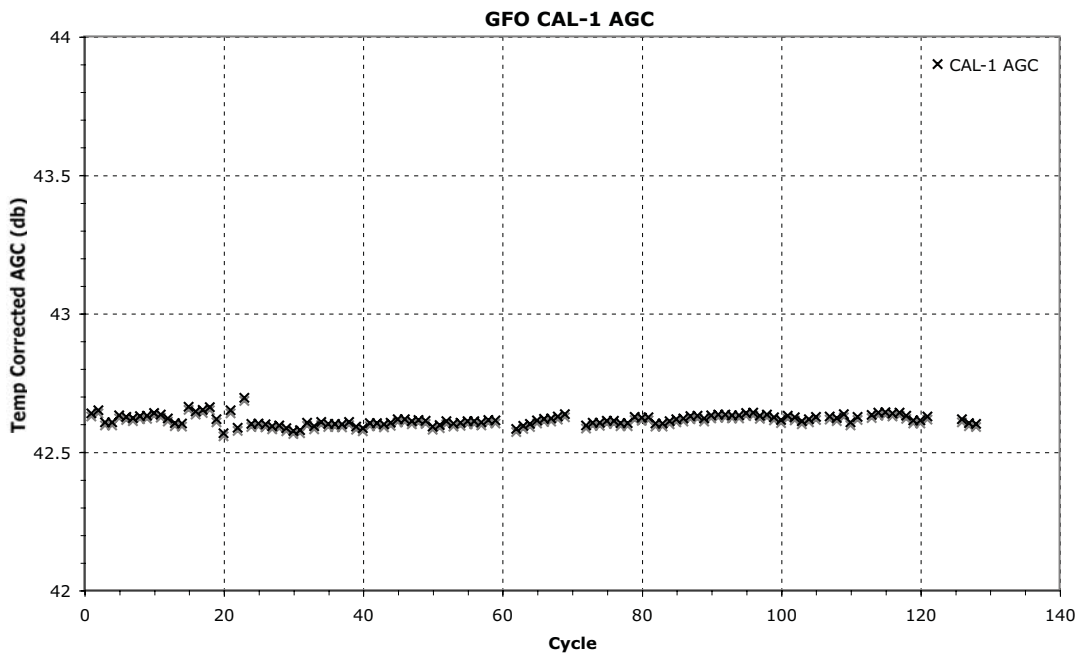
Figure 2-2 CAL-1 AGC for the First 130 GFO Cycles
