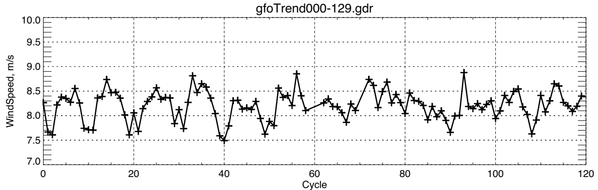
Figure 2-10 GFO Cycle-Averages Windspeed in Meters Per Second
