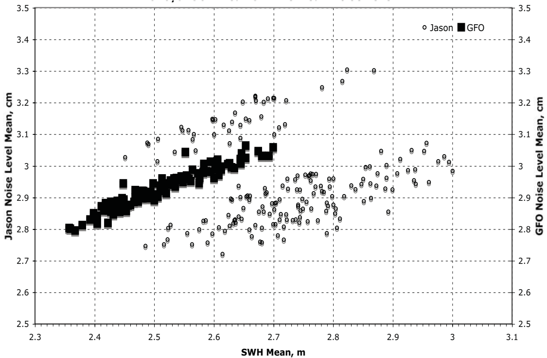
Figure 3-2 GFO/JASON Mean SWH vs. Mean Noise Level
