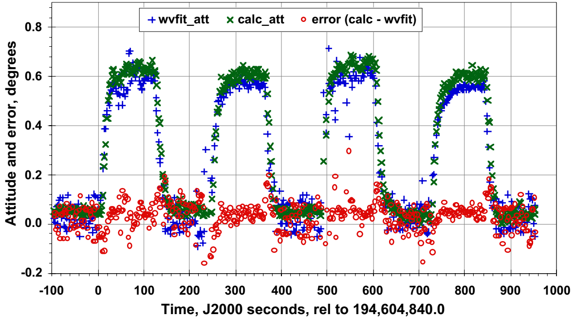
Figure 4-6 Waveform Fit and Calculated Attitudes in 2006/03/02 ABCAL from WFF Boresight Vector Solution
