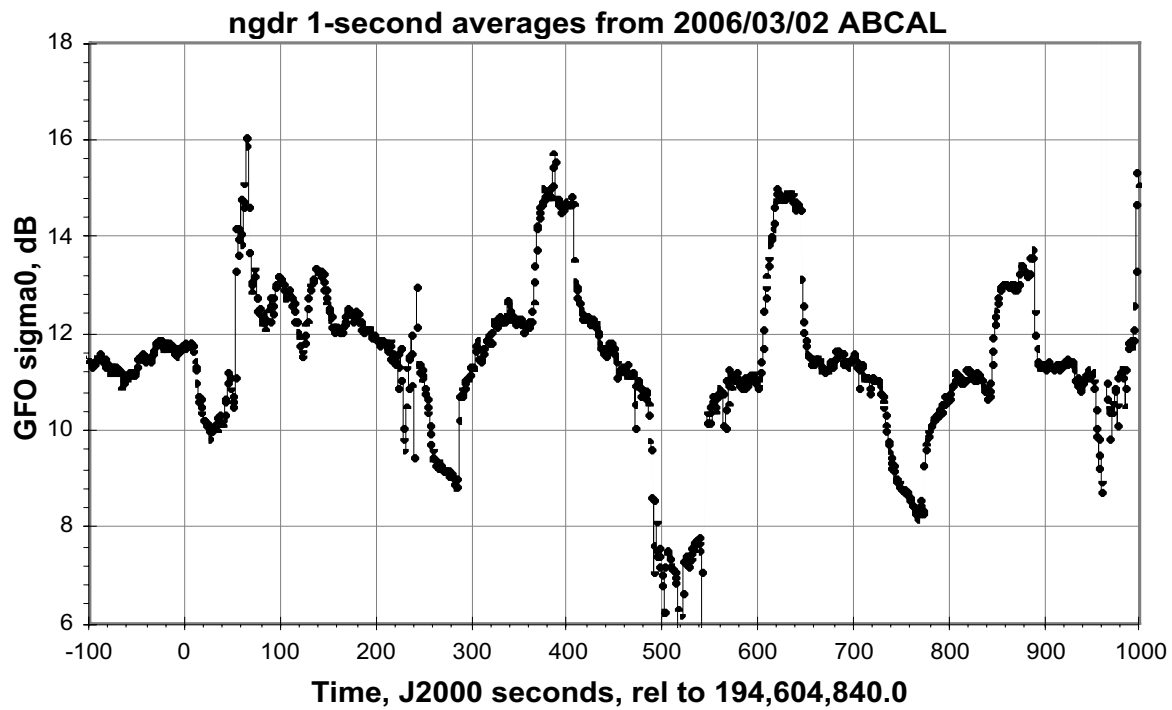
Figure 4-5 GFO NGDR Sigma0 Estimates
