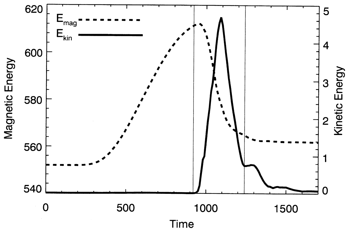
Fig. 5. Evolution of the kinetic (solid line) and the magnetic (dashed line) energies during the simulation. The two vertical lines at t = 920 and t = 1240 separate the three evolutionary phases.
