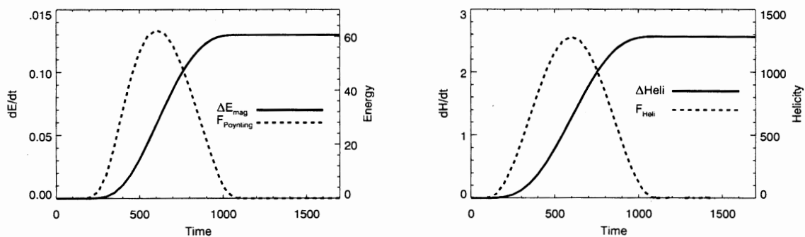
Fig. 6. Injection of energy and helicity through the bottom (photospheric) boundary ( z = 0 ). Left: Poynting flux (dashed curve) and total magnetic energy injection (solid curve) estimated by integrating the Poynting flux. Right: Magnetic helicity flux (dashed curve) and total helicity (solid curve) estimated by integrating this flux.
