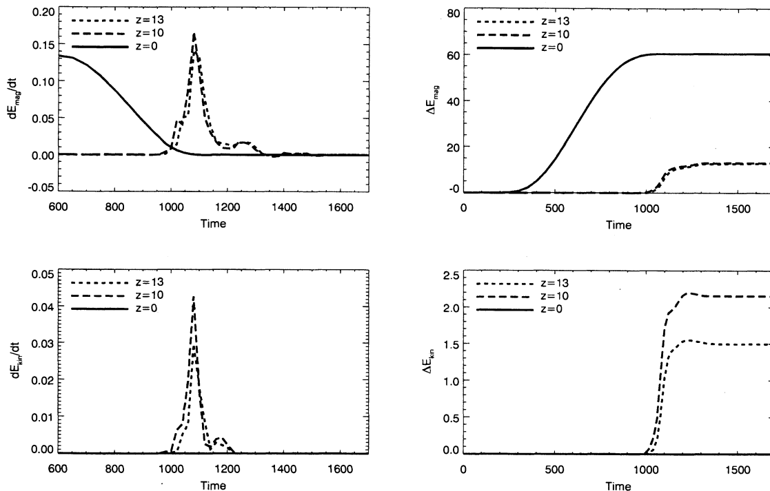
Fig. 10. — Flux ( left column ) and time integrated variations ( right column ) of the magnetic energy ( top row ) and kinetic energy ( bottom row ) through horizontal ( xy ) planes at z = 0, 10, \text{ and } 13 .
