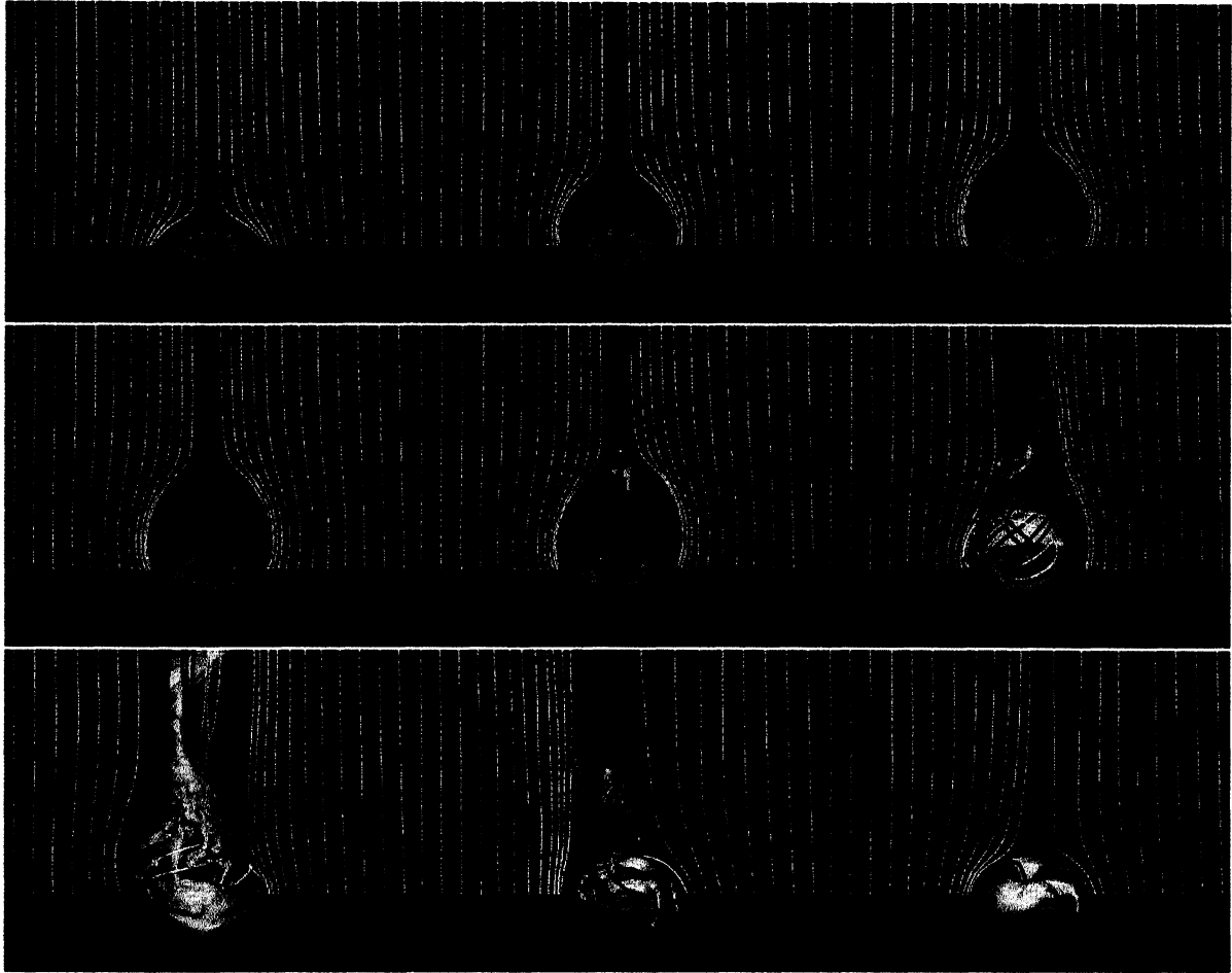
Fig. 4. Evolution of the magnetic configuration. The 2D horizontal plane displays the distribution of |\mathbf{B}| at the bottom boundary (as in Fig. 1). The field lines are plotted starting from fixed position at the bottom boundary along the y axis. The white ones initially belong to the open connectivity domain whereas the blue ones are in the closed connectivity domain. The yellow isocontours correspond to mass density, \rho = 1.25 .
