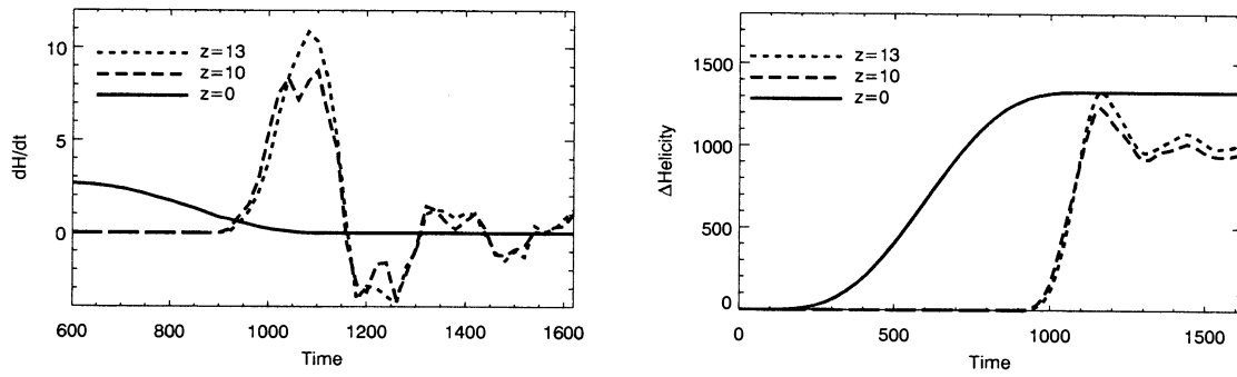
Fig. 11. Flux ( left ) and time integrated variations ( right ) of the magnetic helicity through horizontal ( xy ) planes at at z = 0, 10 , and 13 .
