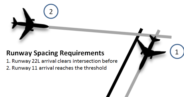
Figure 3. Requirements for adequate spacing at the runway for arrivals to runways 22L and 11
