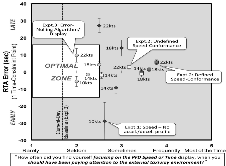
Figure 7. Mean ratings for the attentional allocation question (from Fig. 6) by mean RTA errors for the Commanded Speeds tested in Experiments 1, 2, and 3. (Dashed line represents “current-day baseline” condition rating). Error bars = +/- 1 SE.
