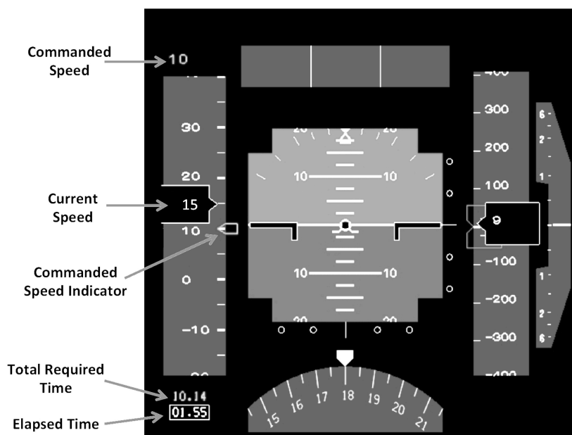
Figure 4. Error-Nulling Algorithm/Display. Speed tape (left side) shows Commanded Speed = 10 kts; Current Speed = 15 kts. Elapsed taxi time = 1:55 min/sec; Total required taxi time = 10:14 min/sec.). Commanded Speed is dynamically calculated and updated by error-nulling algorithm.
