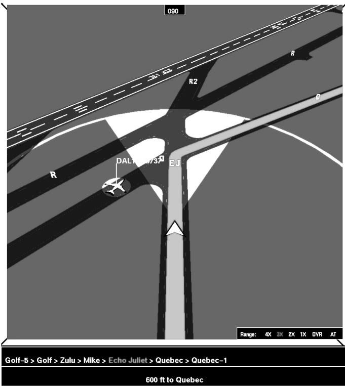
Figure 1. Airport Moving Map (AMM) showing route and ownship position (chevron).
