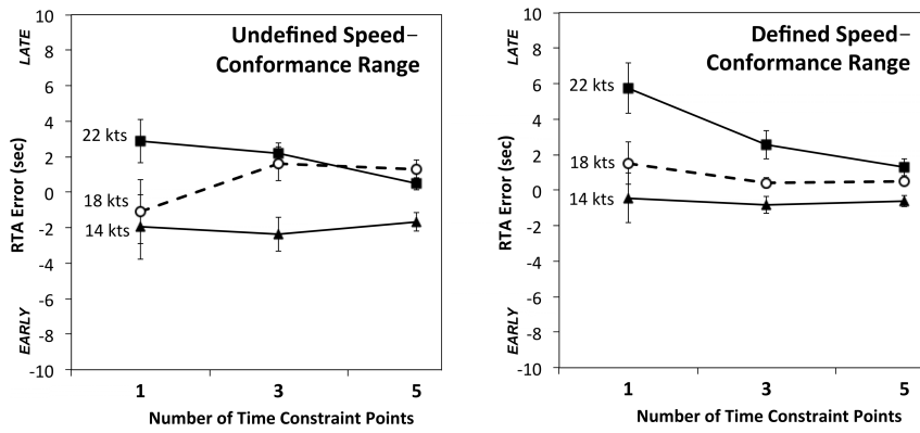
Figure 3. Experiment 2: Mean required time of arrival (RTA) error as a function of Commanded Speed and Number of Time Constraint Points for the Undefined (left panel) and Defined (right panel) Speed-Conformance conditions. Error bars = +/- 1 SE.
