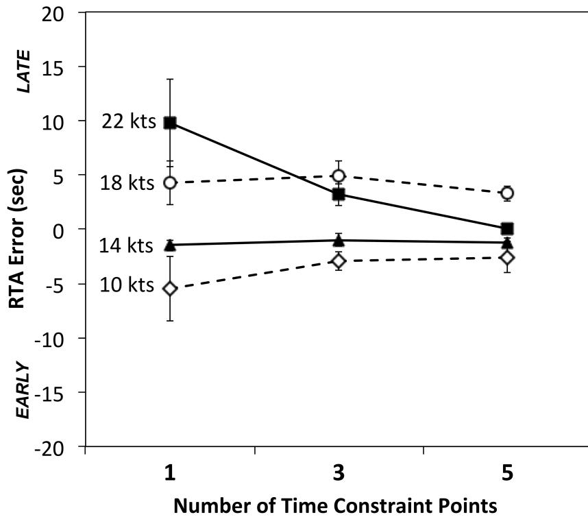
Figure 5. Experiment 3: Mean required time of arrival (RTA) error as a function of Commanded Speed and Number of Time Constraint Points. Error bars = +/- 1 SE.
