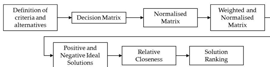
Figure 1. TOPSIS methodology.
