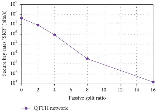
FIGURE 7: Performance comparison of QTTH network with diverse passive split ratios as a function of achieved secure key rates.
