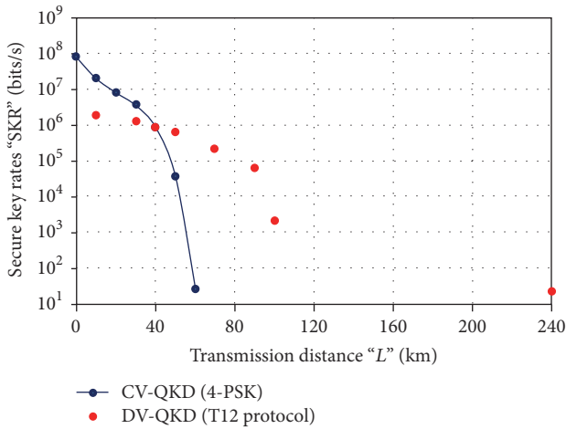
FIGURE 5: Performance comparison of CV-QKD versus DV-QKD for access and metro networks.
