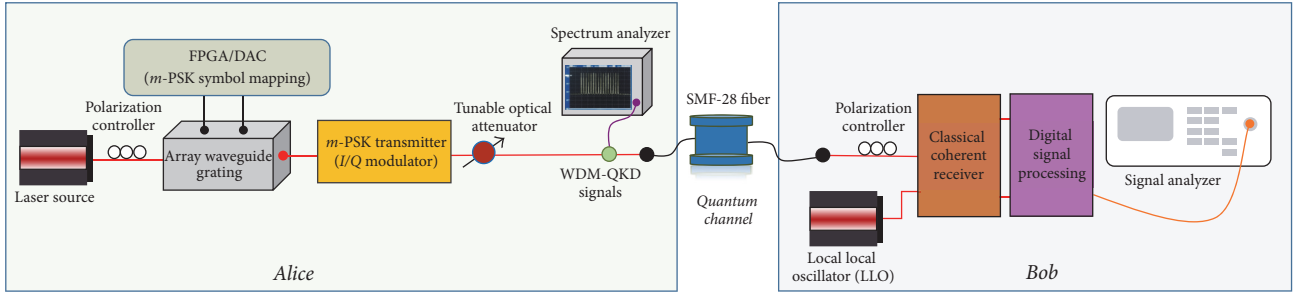
FIGURE 1: Schematic of the m -PSK based quantum transmitter (Alice) and quantum receiver (Bob) for QTT applications.
