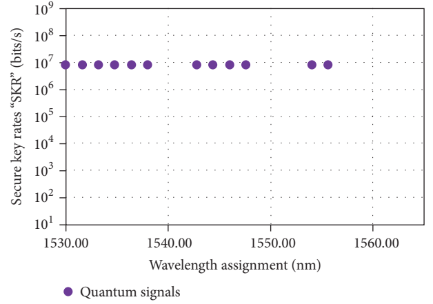
FIGURE 8: Optimum system performance and wavelength assignment for hybrid classical-quantum traffic in an access network.
