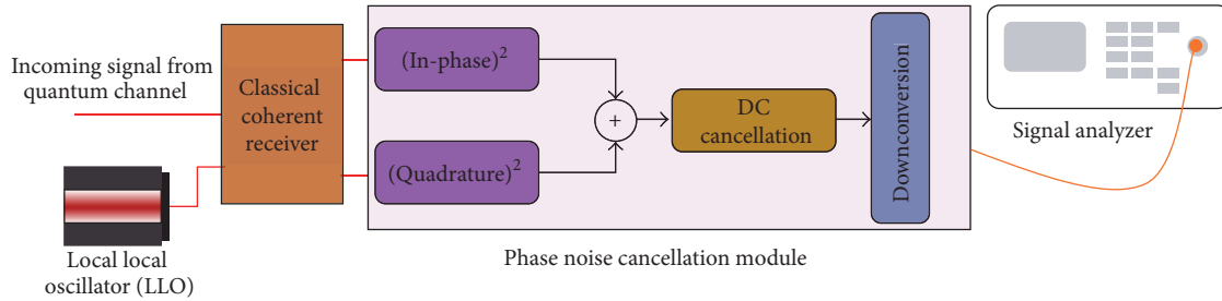
FIGURE 2: Schematic of the digital signal processing (phase noise cancellation) module for quantum receiver (Bob).
