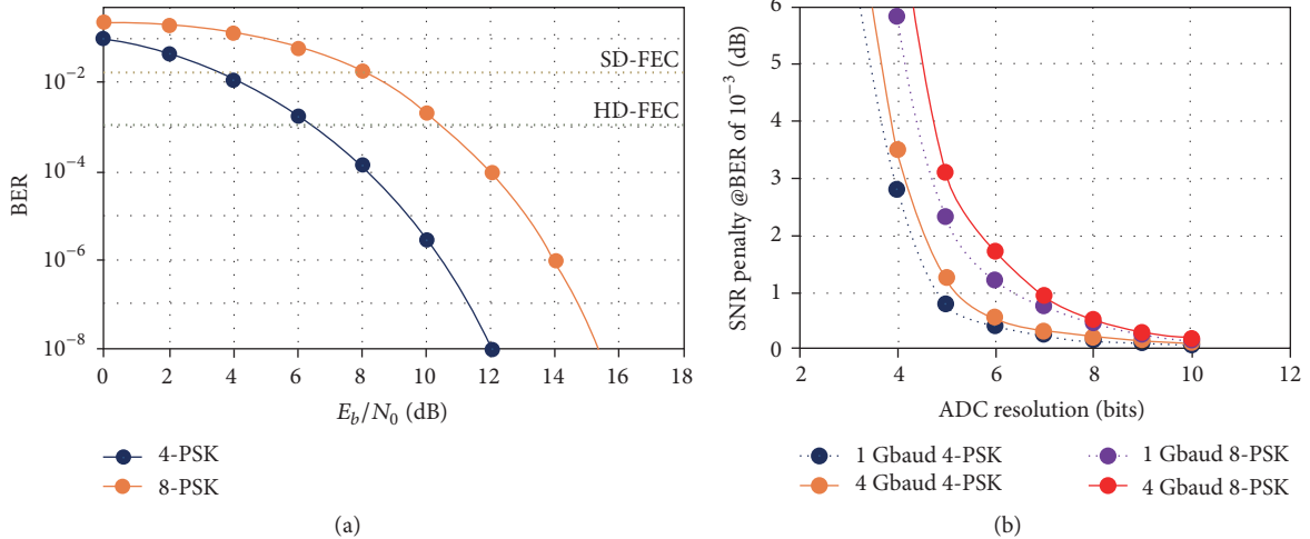
FIGURE 3: Performance comparison of classical data transmissions: (a) averaged SNR with respect to m -PSK signals at different FEC levels and (b) SNR penalty with respect to ADC resolution for different baud rates for m -PSK signals.
