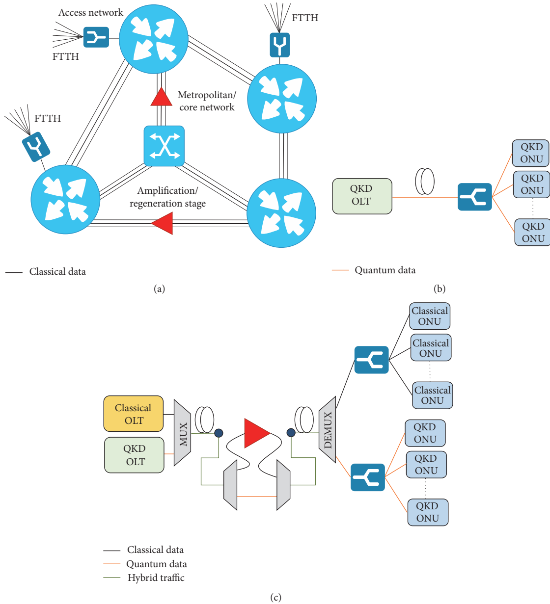
FIGURE 6: (a) Deployment of FTTH network with classical optical components, (b) downstream and upstream quantum access network, and (c) hybrid classical-quantum traffic in access networks.
