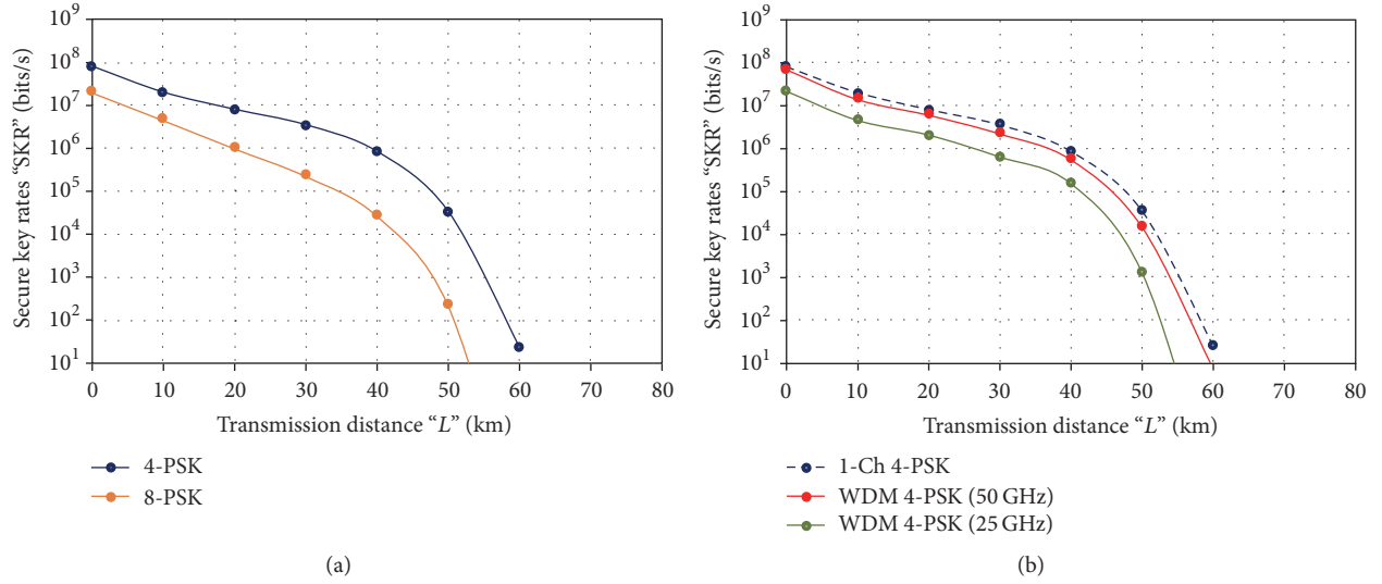
FIGURE 4: Calculated QKD secure key rates as a function of transmission distance for (a) 4-PSK and 8-PSK modulation and (b) single-channel (1-Ch) 4-PSK modulation and 12-channel WDM 4-PSK modulation with 25 and 50 GHz channel spacing. Simulations are performed by assuming 60% detector efficiency and 95% reconciliation efficiency.
