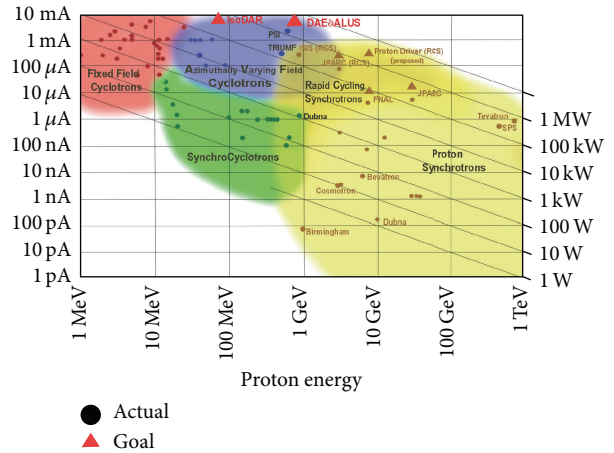
FIGURE 5: Proton energy versus current for various existing machines. The type of accelerator is indicated. Various types of cyclotrons are noted, where FF is the fixed field or classical cyclotron; FM is the frequency modulation (synchro-) cyclotron; and AVF is the azimuthal varying field cyclotron. This plot is taken from [18].
