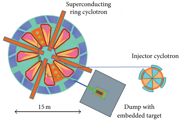
FIGURE 6: A DAEδALUS module.
