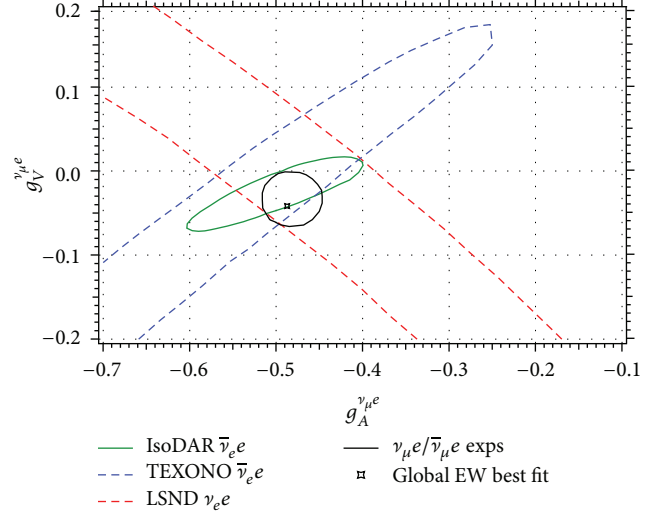
FIGURE 9: IsoDAR’s sensitivity to g_V and g_A along with allowed regions from other neutrino scattering experiments and the electroweak global best fit point taken from [16]. The IsoDAR, LSND, and TEXONO contours are all at 1\sigma and are all plotted in terms of g_{V,A}^{\nu_\mu e} = g_{V,A}^{\nu_e e} - 1 to compare with \nu_\mu scattering data. The \nu_\mu e/\bar{\nu}_\mu e contour is at 90% C.L.
