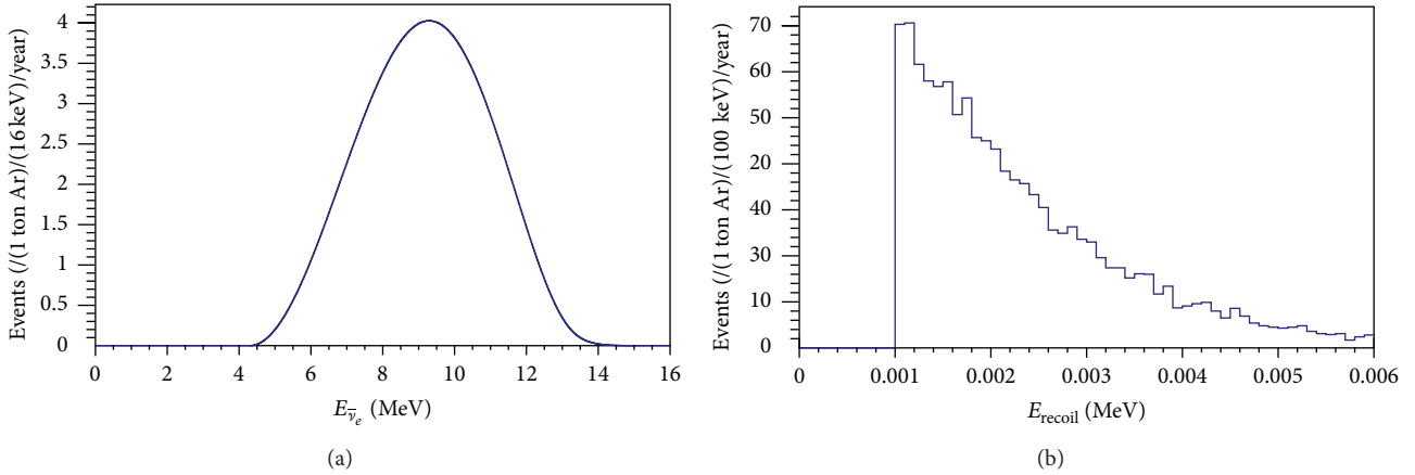
FIGURE 11: (a) Coherent event rate in terms of antineutrino energy with a 1000 kg argon detector at a 10 m average baseline from the IsoDAR source. (b) The event rate in terms of nuclear recoil energy.
