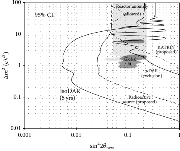
FIGURE 8: Sensitivity of IsoDAR in a nominal 5-year run, in comparison with other experiments. The existing \mu DAR [19] exclusion curve and Reactor + Gallium [20] allowed region are also shown. With respect to future experiments, the expected sensitivities from a propose PetaBequerel source experiment [21] and from KATRIN [22], now under construction, are also indicated. Reprinted from [23].
