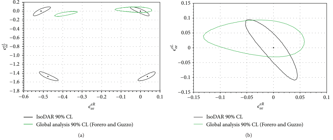
FIGURE 10: (a) IsoDAR's sensitivity to \epsilon_{ee}^{eL} and \epsilon_{ee}^{eR} . The current global allowed region, based on [24], is also shown. (b) A zoomed-in version of the top plot, emphasizing the region near \epsilon_{ee}^{eL} and \epsilon_{ee}^{eR} \sim 0 , is shown.
