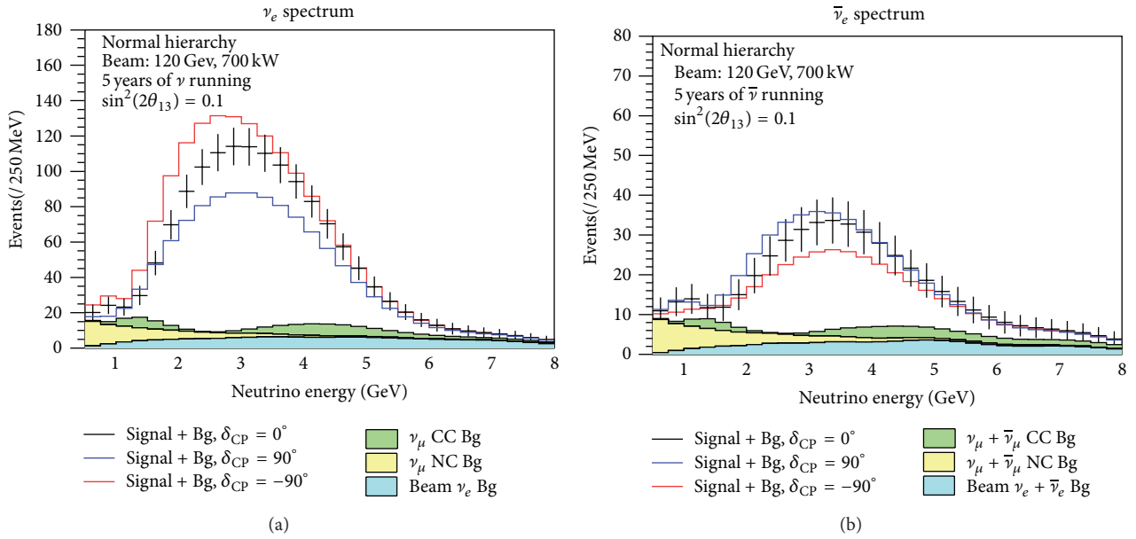
FIGURE 12: Estimated events for the LBNE experiment running for 5 years of neutrino and 5 years of antineutrino with 700 kW of 120 GeV protons on target and with the assumption that \sin^2 2\theta = 0.1 . Backgrounds and changes with \delta_{CP} are also shown. These plots are from [25].
