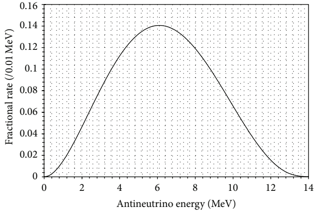
FIGURE 2: The {}^8\text{Li} isotope DAR anti-electron-neutrino flux.
