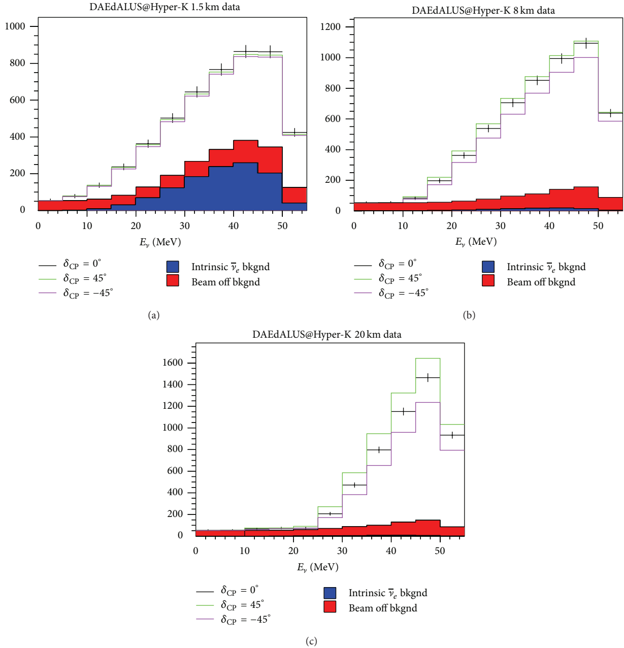
FIGURE 14: The event energy distributions for signal and background of the DAEδALUS@Hyper-K running scenario with \sin^2 2\theta_{13} = 0.10 . Black, green, and violet histograms show signals for \delta_{CP} = 0^\circ , 45^\circ and -45^\circ . The blue histogram shows the intrinsic \bar{\nu}_e beam-on background. The red histogram shows the beam-off backgrounds. (a) and (b) show events from the near (1.5 km) and middle (8 km) accelerators. (c) shows events from the far (20 km) accelerator.
