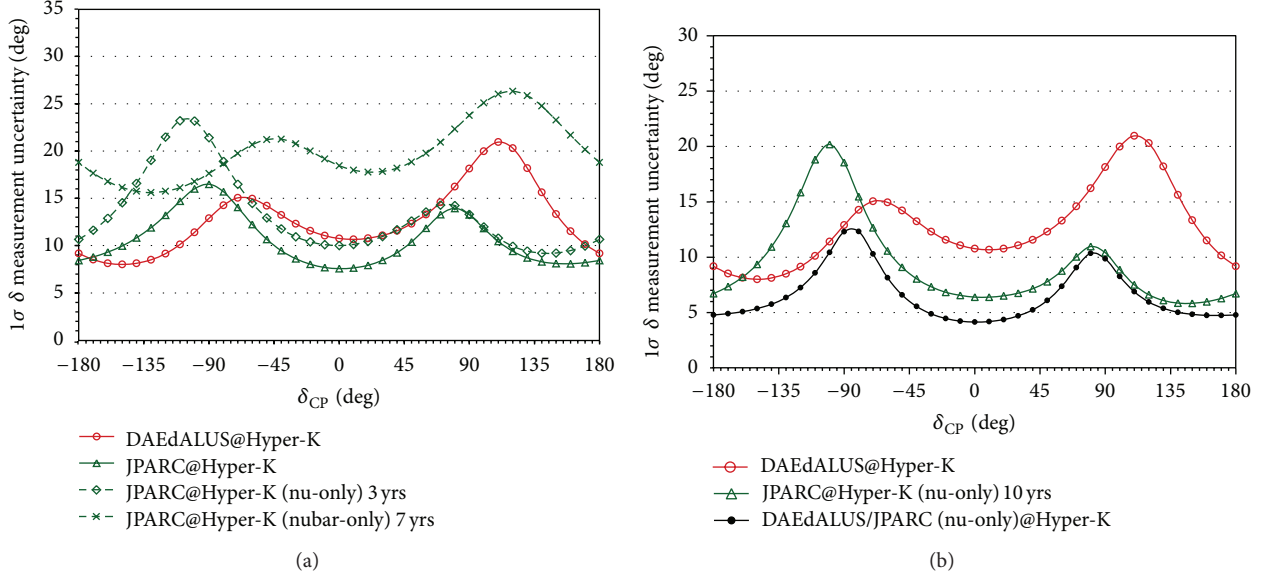
FIGURE 15: (a) 1\sigma measurement sensitivities for the nominal JPARC@Hyper-K run (solid green with triangles) compared to DAE \delta ALUS@Hyper-K (solid red) assuming the normal mass hierarchy. Dashed green curves show contributions of neutrino and antineutrino running to the total sensitivity of JPARC@Hyper-K. (b) DAE \delta ALUS/JPARC(nu only)@Hyper-K combined measurement sensitivity assuming the normal mass hierarchy. The contribution to the combined measurement from DAE \delta ALUS antineutrinos is indicated in red and the contribution from JPARC neutrinos is indicated in green.
