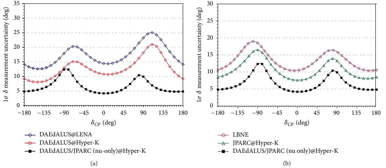
FIGURE 16: (a) The sensitivity of the CP violation search in various configurations assuming the normal mass hierarchy: dark blue:DAE \delta ALUS@LENA, red:DAE \delta ALUS@Hyper-K, and black:DAE \delta ALUS/JPARC(nu-only)@Hyper-K. (b) pink:LBNE; green: JPARC@Hyper-K [26], and black:DAE \delta ALUS/JPARC(nu-only)@Hyper-K (same as above). See Table 5 for the description of each configuration.
