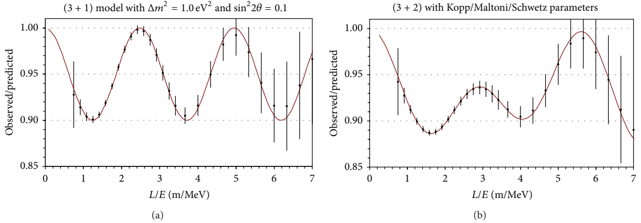
FIGURE 7: Example data sets for 5 years of running for 3 + 1 (a) and 3 + 2 (b) oscillation scenarios.
