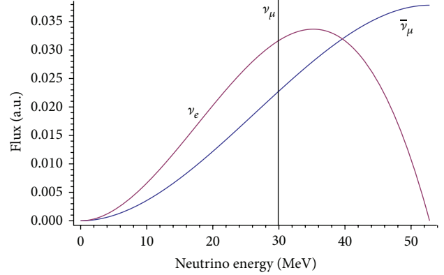
FIGURE 3: Neutrino flux distribution from a pion/muon DAR source, from [17].
