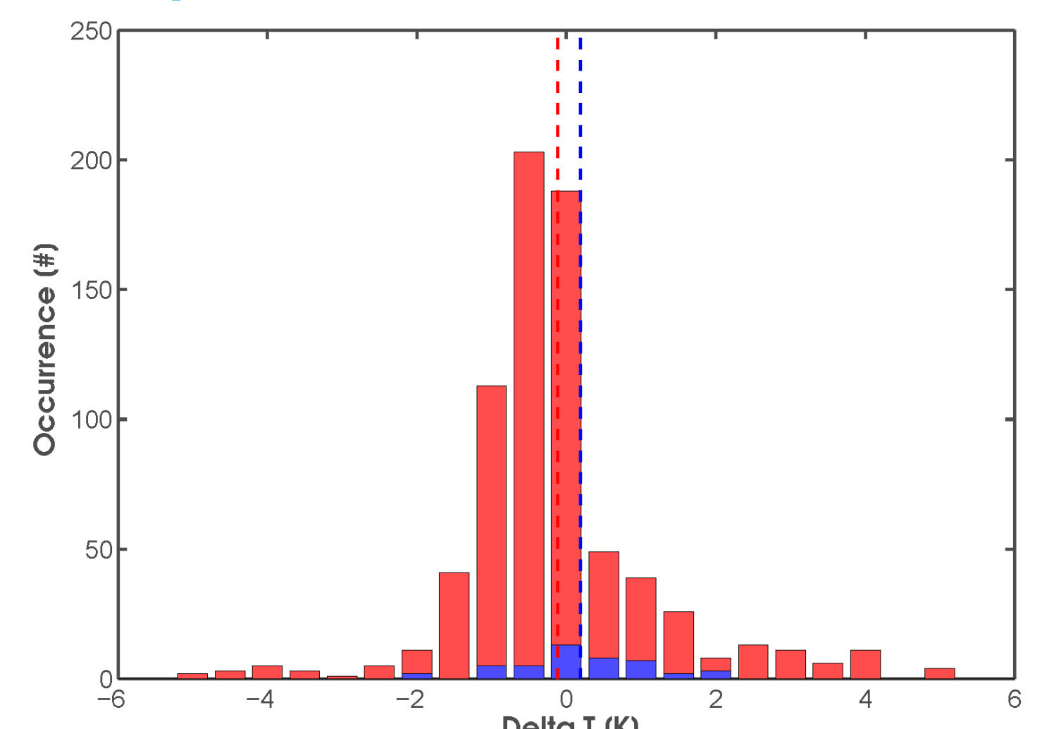
Fig 6: Dropsonde minus aircraft for measurements in cloud free air (red) and inside clouds (blue). Mean values agree within \pm 0.1 \text{ K} in cloud free and cloudy air.
