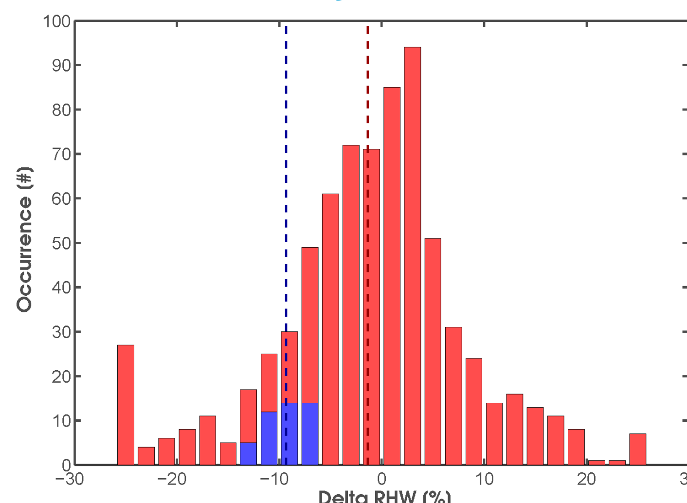
Fig 4: Dropsonde minus aircraft for measurements in cloud free air (red) and dropsonde compared to 100 % inside clouds (blue). Mean values agree within 2 % RH in cloud free air. Inside clouds, the mean bias is almost -10\% .
