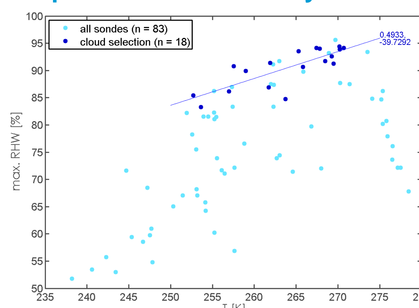
Fig 5: Maximum dropsonde humidity per profile within and out of clouds.
