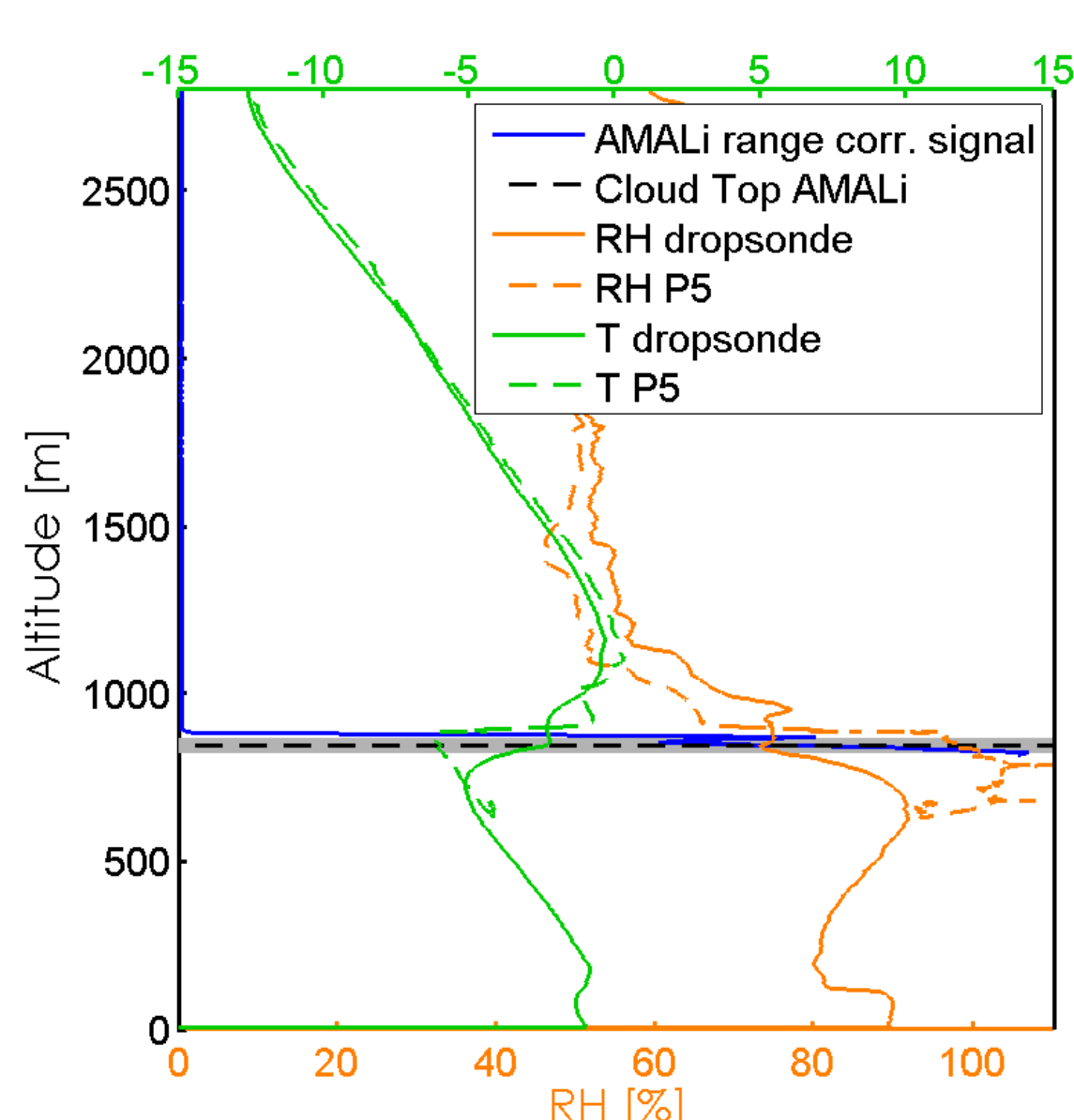
Fig 3: Example of profiles measured by dropsonde and Polar 5 aircraft. The top of a stratus cloud at 850 m can be seen in temperatures and humidities and by the AMALi lidar backscatter. Aircraft humidity shows a vertical extent of the cloud of about 250 m.
