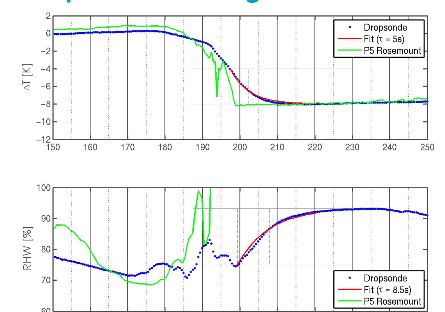
Fig 7: Example for dropsonde time constant estimation at cloud top transitions.
