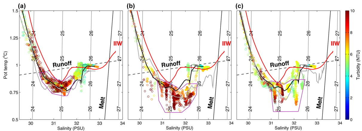
Figure 6. Turbidity of glacially modified waters. \theta ( ^{\circ}\text{C} ) and S (PSU) profiles from the regions along R4 and R5 outlined in blue (GMW1 region) (a), gold (GMW2 region) (b), and white (the region between GMW1 and GMW2) (c) in Fig. 3, with turbidity plotted as the color of the point. CTD1 (a), CTD2 (b), and CTD3 (c) are plotted in grey. The GMW region in \theta/S space is outlined in purple. The average of all R4 and R5 measurements and the ambient fjord waters are plotted in black and red, respectively. Black square along ambient fjord water profile shows \theta/S properties at sill depth (70 m).
