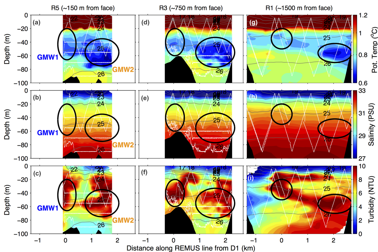
Figure 4. Select REMUS across-fjord sections. \theta ( ^{\circ}\text{C} ), S (PSU), and turbidity (NTU) sections along REMUS lines (a)–(c) R5, (d)–(f) R3, and (g)–(i) R1 from 0 to 100 m depth. Sections are oriented looking away from the terminus, with the southwestern end of the section on the left. Across-fjord transect distance is plotted as horizontal distance along section, with 0 km located at the intersection of the REMUS section with an along-fjord line running from D1 to the southwestern LBL transponder along R1 (Fig. 3). GMW1 and GMW2 regions identified by black ellipses, and labeled in blue and gold, respectively in (a)–(c). Isopycnals plotted in grey, REMUS mission tracks shown in white (Table 1), and bathymetry shown in black (Fig. 3).
