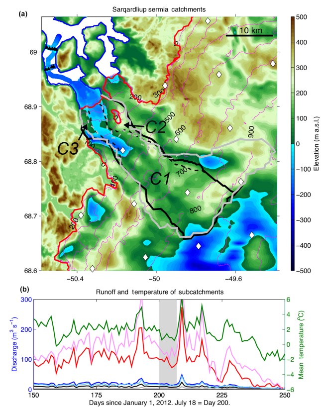
Figure 7. Saqqarliup sermia catchments and discharge. (a) Estimated Saqqarliup sermia catchment (thick black line) and subcatchments C1, C2, and C3 (dashed black line) from the MBM2014 analysis over Morlighem et al. (2014) bedrock elevation map (filled contours) and ice sheet surface (magenta contours). BBM2013 catchment and subcatchment outlines in thick solid and dashed grey lines, respectively. Ice sheet margin and coastlines shown in red and blue, respectively. RACMO2.3 11 km resolution grid points shown with white diamonds. Sarqardleq Fjord bathymetry and outer Sarqardleq Fjord CTD positions (black triangles) and depth measurements also shown. (b) Daily C1, C2, and C3 subcatchment MBM2014 RACMO2.3 discharge estimates (red, blue, and black lines, respectively) and daily average RACMO2.3 temperature (green line) across the Saqqarliup sermia subcatchment C1 for DOY 150–250, 2012. Daily C1, C2, and C3 subcatchment BBM2013 RACMO2.3 discharge estimates in pink, cyan, and grey lines, respectively. Dates of REMUS and CTD sampling from DOY 200–207 marked by grey bar.
