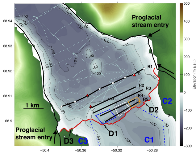
Figure 3. July 2012 Survey of Sarqardleq Fjord. Sarqardleq Fjord bathymetry (10 m colored contours below sea level within fjord) and Morlighem et al. (2014) bedrock elevation map (10 m colored contours above and below sea level outside of fjord) are shown. The Saqqarliup sermia front position and coastline from a 19 June 2012 Landsat image are mapped in red and black lines, respectively. Depth measurements collected during July 2012 field operations used to create the Sarqardleq Fjord bathymetry are plotted as grey dots over the contoured bathymetry. REMUS transects R1–R5 are shown in black, with LBL transponders mapped with red triangles. Subglacial subcatchments C1, C2, and C3 dividing lines from MBM2014 analysis are mapped in dashed blue line, with the location of D1, D2, and D3 subglacial discharge channels along the submerged terminus shown with thin black arrows. CTD casts are shown with diamonds: white diamonds are CTD casts along R1 used in REMUS cross-calibration, and the blue, gold, and grey diamonds are CTD casts 1, 2, and 3 that were taken along R5 within GMW1, GMW2, and the region between GMW1 and GMW2 (outlined in blue, gold, and white, respectively). Three proglacial stream entries to Sarqardleq Fjord are shown along the northeast and southwest fjord coastlines with thick black arrows.
