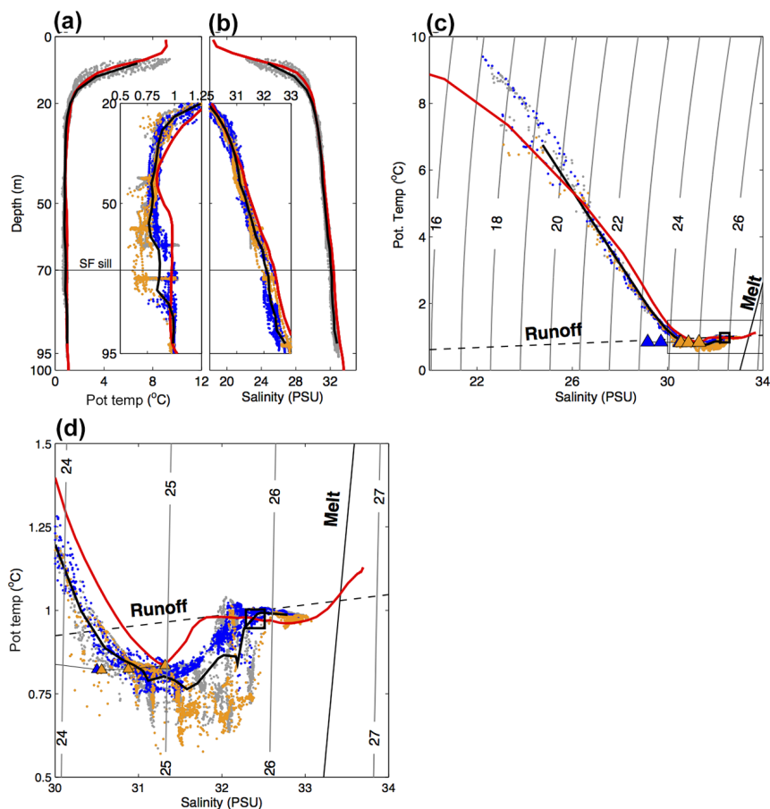
Figure 5. Glacially modified water in Sarqardleq Fjord. \theta ( ^{\circ}\text{C} ) (a) and S (b) profiles for R4 and R5 measurements over the full water-column depth (grey), with the average of R4 and R5 measurements and the ambient fjord waters in black and red, respectively. (a) and (b) insets show same data from 20–95 m depth over a finer \theta or S range, with measurements taken within the GMW1 and GMW2 regions along R4 and R5 (Fig. 3) shown in blue and gold, respectively. \theta/S plots of R4 and R5 measurements (c) (colors same as in a and b), with melt and runoff mixing lines. Intersection for melt and runoff mixing lines set to CTD2 properties at grounding line depth (Fig. 6b). Black square along ambient fjord water profile shows \theta/S properties at sill depth (70 m). \theta/S results for the Jenkins (2011) plume modeling (Table 4) of D1 (blue triangles) and D2 (gold triangles) shown. (d) Same data as in (c) over finer \theta/S range indicated by thin black box in (c).
