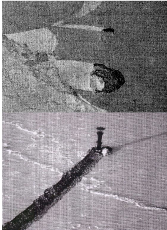
Fig 2 Top: Lanes downstream of obstacles in the Elysium frozen sea. Bottom: Similar lane downstream of a lighthouse, Baltic Sea, with ice pressure ridges.
