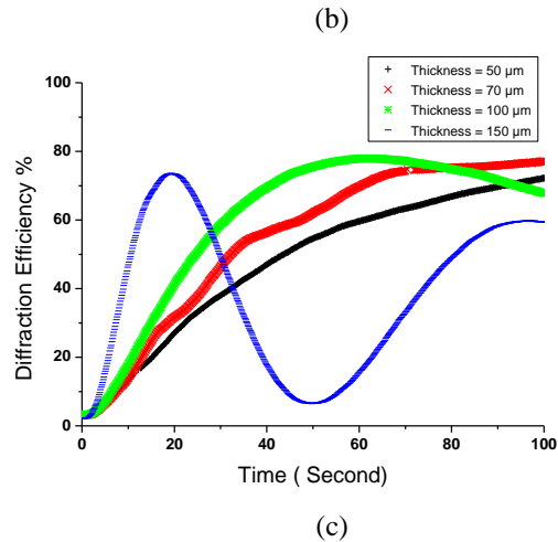
Figure 5 Real time measurements of the diffraction efficiency of gratings recorded in polymer layers of various thickness; recording intensity is 1\text{mW/cm}^2 and the spatial frequency is a) 100\text{ l/mm} , b) 200\text{ l/mm} , c) 300\text{ l/mm} .
