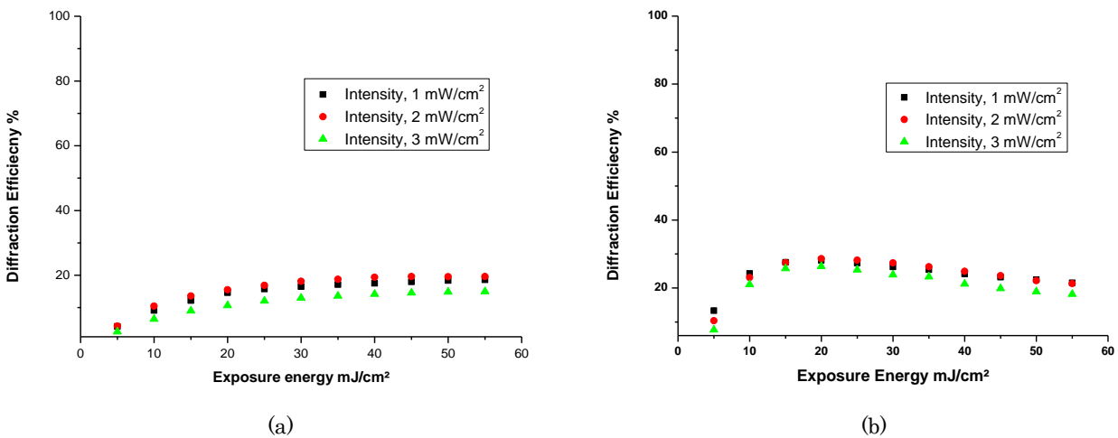
Figure 6 Measured diffraction efficiency vs. Exposure energy for transmission gratings with intensity from 1\text{--}3\text{ mW/cm}^2 at spatial frequency of 100\text{ l/mm} investigated for sample thicknesses of a) 50\mu\text{m} , b) 75\mu\text{m} .
