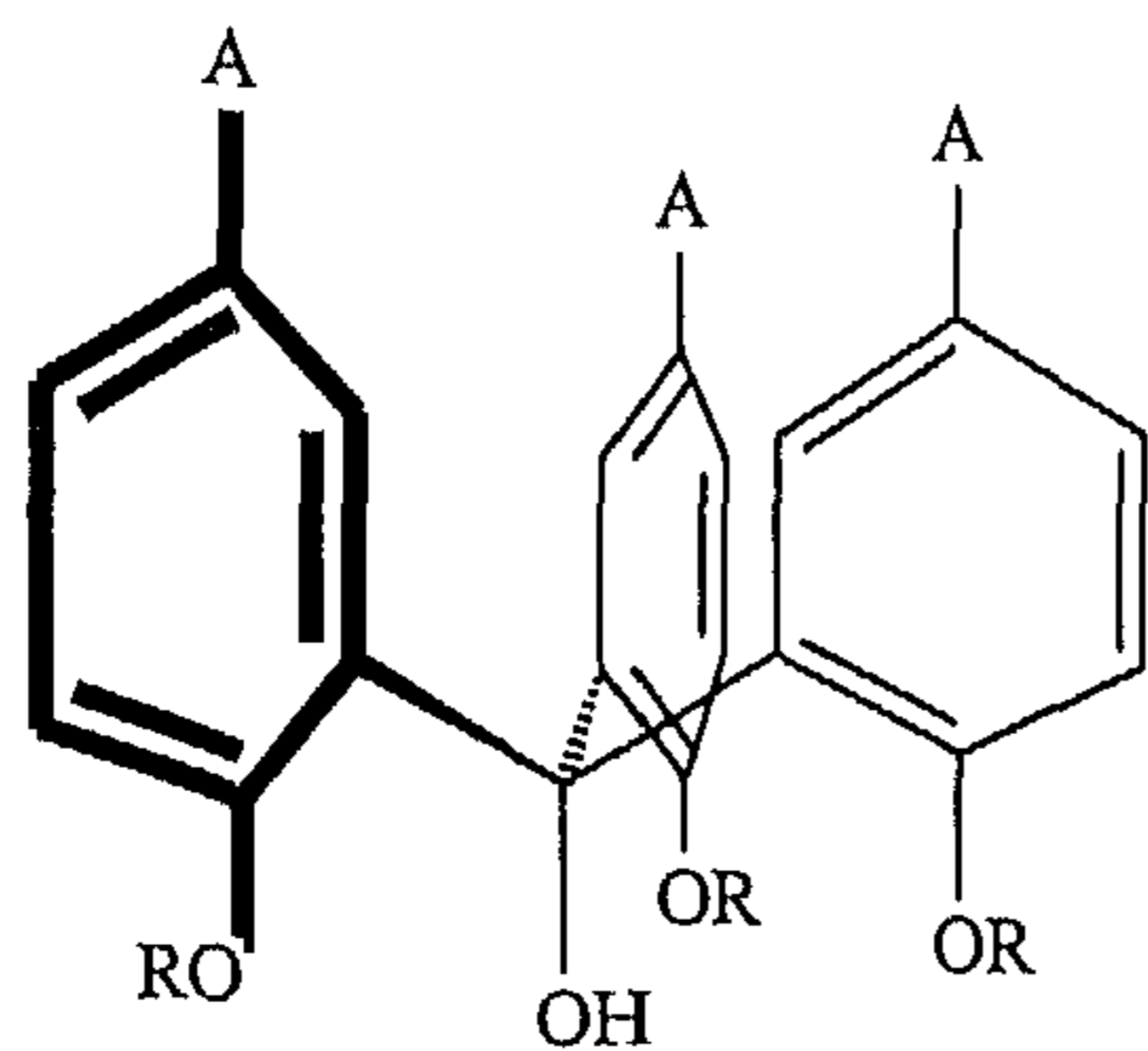
Figure 1. A 2,5-D- \pi -A-substituted triphenylcarbinol.
