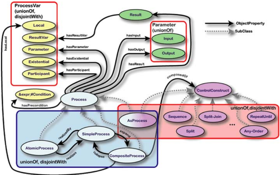
Figure 3 Top-level structure of the OWL-S process model.
