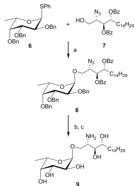
Scheme 2. (a) NIS/TfOH, \text{CH}_2\text{Cl}_2 , -78 °C to -20 °C, 68%; (b) NaOMe/MeOH, 92%; (c) \text{H}_2 , Pd, 76%.
