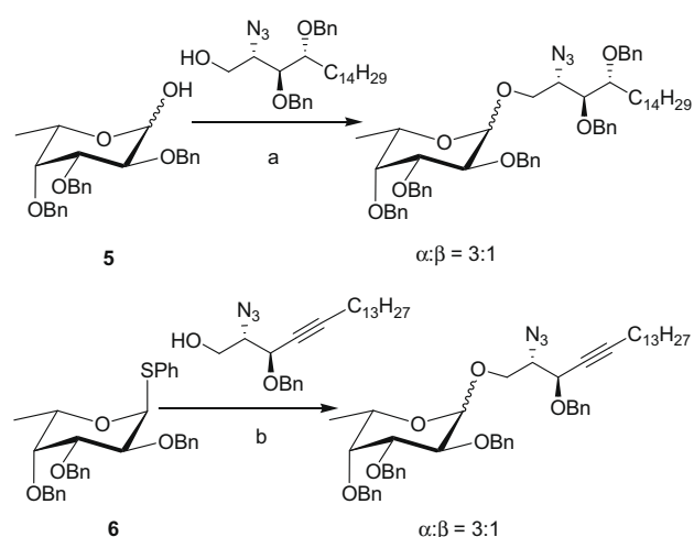
Scheme 1. (a) \text{Me}_2\text{S} , 2-Cl-pyridine, \text{Tf}_2\text{O} , \text{CH}_2\text{Cl}_2 ; (b) dimethyl(methylthio)sulfonium triflate (DMTST), \text{CH}_2\text{Cl}_2 , 0 °C-rt.
