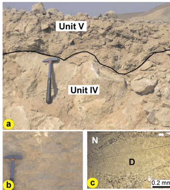
Figure 9. (a) Outcrop exposure showing the contact between Unit IV and Unit V (Loc. 1). The contact is irregular with clear lithologic change across it. The lower part of Unit V consists of interbeds of Unit IV and Unit V lithofacies (Salad Hersi et al. , 2008). (b) Close-up view of Unit V showing prolific larger foraminifera tests (Nummulites, Asselinas and Discocyclusinas) commonly dispersed throughout the unit (hammer in both a and b is 33 cm long). (c) a thin section photomicrograph showing larger Discocyclusina (D) and Nummulites (N) tests.
