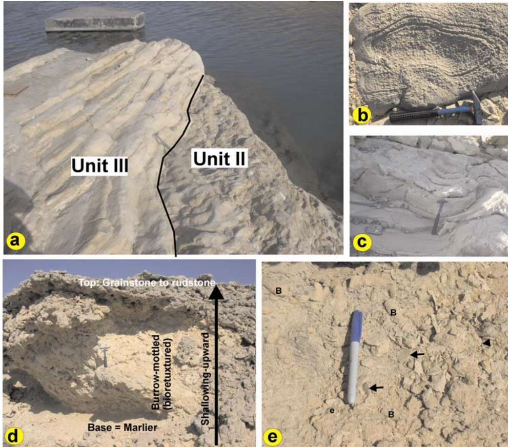
Figure 8. (a) Field view of the sharp contact separating Unit II from Unit III (Loc. 3). (b) Hummocky cross stratification that commonly occurs within Unit III (Loc. 3). Hammer (in all pictures) is 33 cm. Photos d & e are from Unit IV and show textural appearance of the unit. The unit is the thickest among all units of the formation and is characterized by rhythmically stacked cycles. (d) Single cycle defined by a basal, recessive, muddy / marly rudstone to flauostone lithofacies followed by highly burrowed (bio-ret textured) packstone grading into more resistant, cleaner bioclastic packstone / grainstone / rudstone lithofacies. (e) Close-up view of the basal burrowed facies with significant amount of larger foraminifera (arrows) including Nummulites and fusiform Alveolina .
