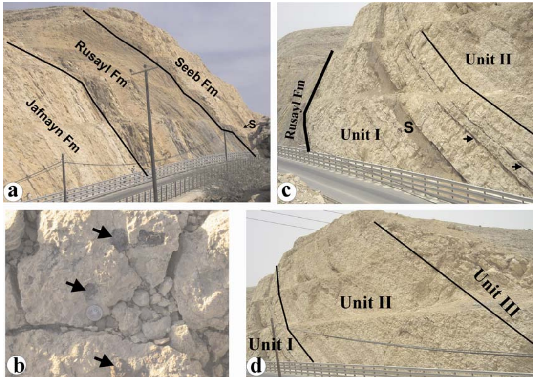
Figure 5. Outcrop exposures showing (a) the Jafnayn – Rusayl – Seeb sequence with formational boundaries demarcated with thick black lines (Loc. 2); (b) a hardground surface with ferruginous nodules (arrows) replacing bioclasts. This surface most likely indicates the top of the Seeb Formation (~ 250m northwest of Loc. 1, close to SQU); (c) Unit I of the Seeb Fm. Exposed in Loc. 2. Note the Rusayl-like layers (S & arrow heads) with the unit; (d) Unit II of the Seeb Fm. also exposed in Loc. 2. The upper contact with Unit III is also exposed here.
