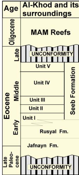
Figure 2. Stratigraphic chart showing the various late Paleocene to Oligocene lithostratigraphic units in the study area. Note the interfingering nature of the Rusayl – Seeb contact. The Seeb Formation is divided into five informal units (I to V) and it is unconformably overlain by the MAM (Muaskar Al Murtafa’ reefs).
