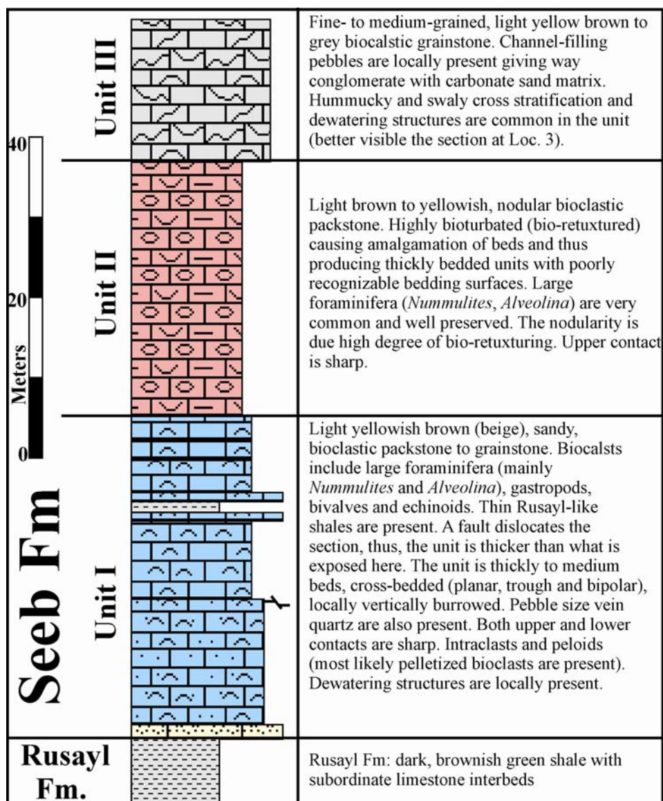
Figure 4. Stratigraphic log of Section 2 (Al-Khoud Road-cut) showing the Rusayl – Seeb contact and descriptions of the lower three units that are exposed along the section. Note the fault that lies within Unit I. The upper contact of Unit III is not exposed.
