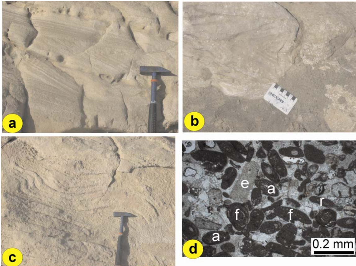
Figure 6: Sedimentary structures and microfacies attributes of Unit I. (a) Tabular x-bedding; (b) bidirectional, tabular x-bedding (herringbone x-bedding); (c) deformation of the layers due to dewatering (hammer = 33 cm, pencil ~ 10 cm), and the bars on the card in c are in cm); (d) thin section photomicrograph showing bioclastic grainstone (f = foraminifera, e = echinoid, a = Alveolina, r = red algae).
