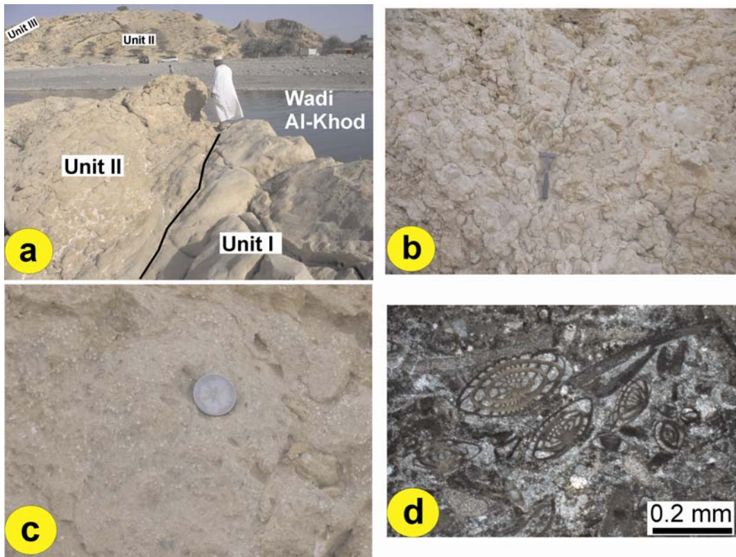
Figure 7. (a) Outcrop exposure showing the sharp contact between Unit I and Unit II (Loc. 3). (b) A view highlighting the nodular texture of Unit II (hammer = 33 cm). (c) Close-up view of Unit II showing scattered larger foraminifera tests in the unit (coin is ~1.5 cm in diameter). (d) Thin section photomicrograph of Unit II showing a grainstone lithofacies rich in Nummulites and other fossil fragments.
