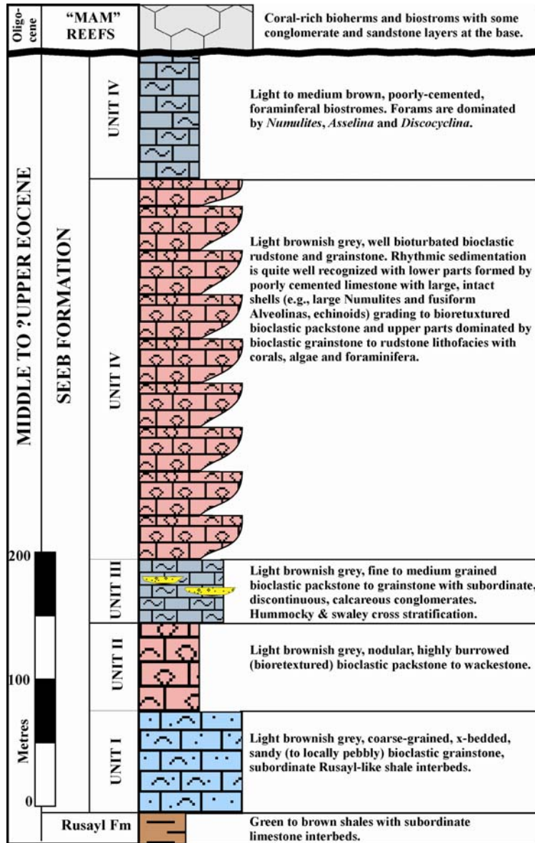
Figure 3. Hypothetical stratigraphic log for the Seeb Formation with lithologic descriptions of the five units that constitute the formation. The cycles shown for Unit IV are not to their actual scale.
