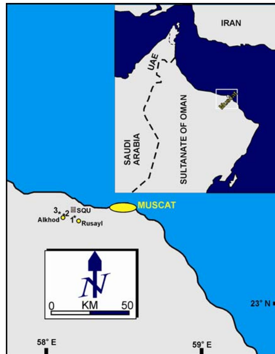
Figure 1. Location of the studied area and sections (1, 2 and 3). Section 1 lies along the SQU-Waha Al Ma'rifah Institute, Section 2 is the Al-Khoud road-cut and Section 3 is the along Wadi Al-Khoud, north of Al-Khoud village.
