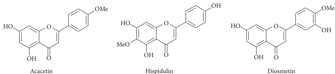
FIGURE 8: Chemical structure of acacetin (1), hispidulin (2), and diosmetin (3).
