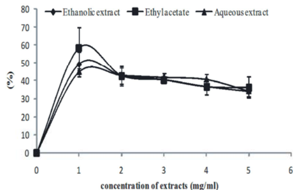
Fig. 1: Ferric reducing antioxidant properties of ethanolic, ethyl acetate and aqueous extracts of Ocimum gratissimum .
