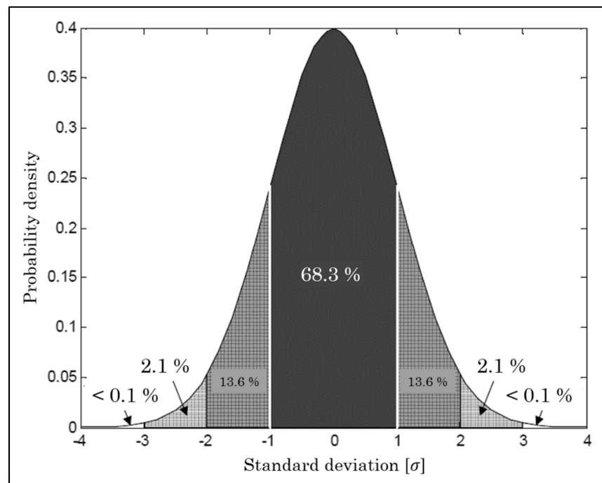
Figure-A IV-1 Centered normal distribution
