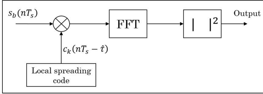
Figure 3.15 Block diagram of the parallel frequency search acquisition
