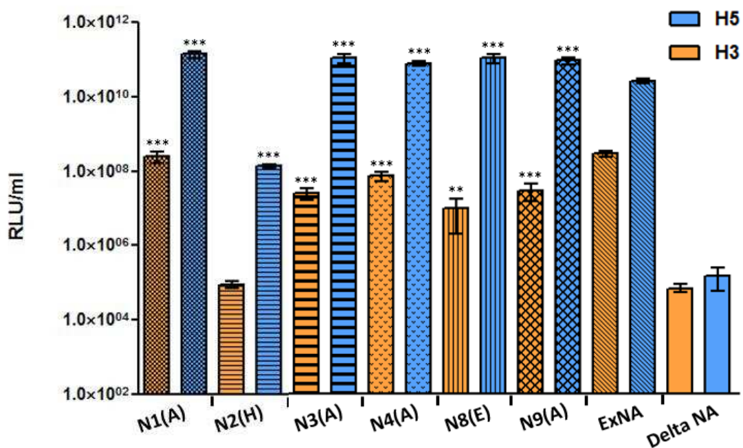
Figure 52. A/equine/Richmond/1/2007 H3 (orange) and A/Vietnam/1194/2004 H5 (blue) mean PV titres generated by co-transfection with different NA plasmids (Table 22 contains NA strains). Species origin of NA denoted by; A – avian, C – canine, E – equine, and H – human. An exogenous source of NA (ExNA) was added 24hours post transfection as a positive control and Delta (without) NA was generated as a negative control. PV titres reported in relative luminescent units (RLU/ml), +/- SEM of eight replicates. Statistically significant differences (Mann-Whitney test) between mean RLU/ml of each HA/NA combination PV and the Delta NA control are indicated by ** = p < 0.01 ; *** = p < 0.001 .
