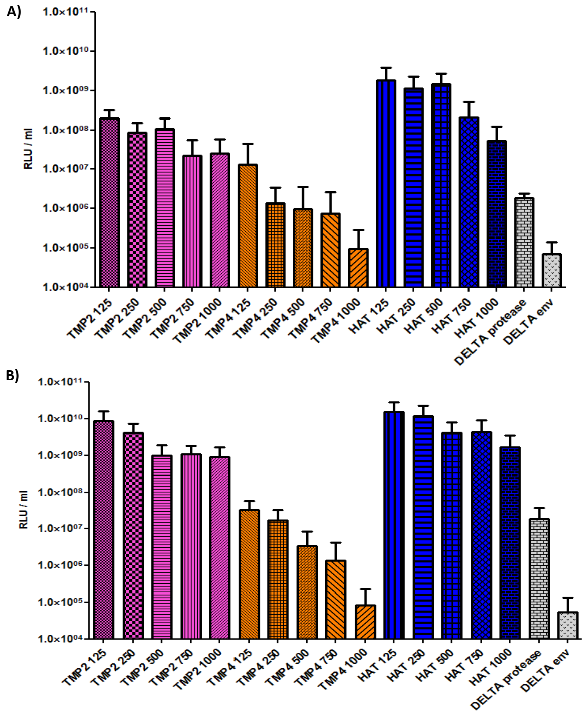
Figure 16. PV titres obtained with A) A/equine/Richmond/1/2007 H3 and B) A/equine/Newmarket/1979 H3 in combination with selected protease-expressing plasmids. TMPRSS2 (TMP2), TMPRSS4 (TMP4) and HAT proteases were trialed, each number denotes the quantity of protease plasmid used (ng). PV titres reported in relative luminescent units (RLU/ml) and error bars represent +SEM from 8 replicates.
