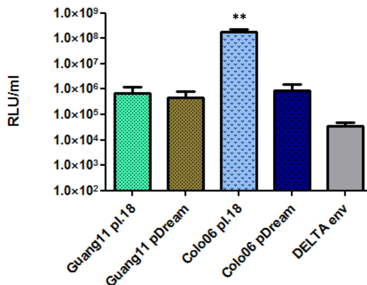
Figure 42. Attempted generation of H3-only PVs derived from A/canine/Colorado/30604/2006 H3N8 (Colo06) and A/canine/Guangdong/3/2011 H3N2 (Guang11) strains using different HA-encoding plasmid vectors; pDream and pl.18. Mean PV titres are reported in relative luminescent units (RLU/ml) based on eight replicates with error bars indicating +SEM. ** Indicates a significant difference ( p < 0.05 ) determined by an unpaired T-test.
