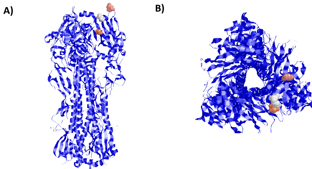
Figure 33. Trimeric HA structure of A/Newmarket/2/93 (PDB: 4UNW) highlighting amino acid residues at positions of 159 (pink), 189 (white) and 227 (orange), on one chain, from A) the side-view and B) top view of the protein. Protein figures edited using RasWin software (Version 2.7.5.2).
