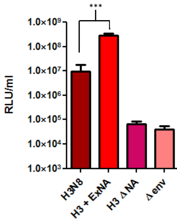
Figure 18. A/equine/Richmond/1/2007 H3 PV titres of preparations generated by co-transfection with an N8 encoding plasmid or using the standard technique of adding exogenous (Ex) NA (positive control). H3 \Delta NA (H3 without NA) and \Delta env (no HA or NA) were generated as negative controls. Average PV titres reported in relative luminescent units (RLU/ml), with error bars indicating +SEM, based on 8 replicates. The statistically significant difference between H3+ExNA and H3+N8 encoding plasmid is indicated by *** (Mann-Whitney test; p < 0.001 ).
