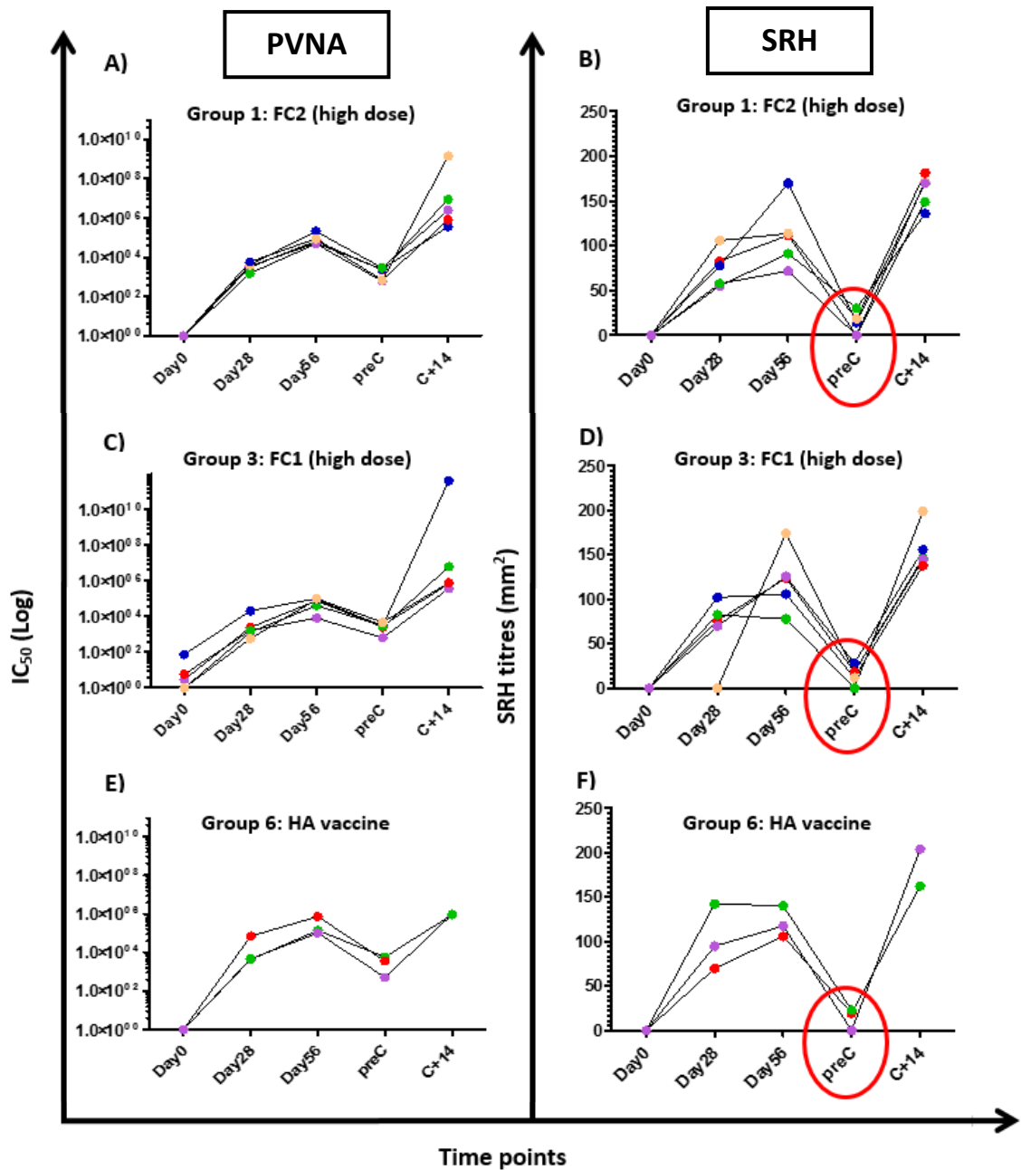
Figure 27. Neutralising antibody responses as measured by PVNA (A, C, E) compared to SRH (B, D, F). Responses were recorded at five different time points during the vaccine efficacy trial; Day 0, Day 28, Day 56, pre-Challenge (preC) and 14 days post challenge (C+14). Red circles highlight the point in time where SRH values are negative.
