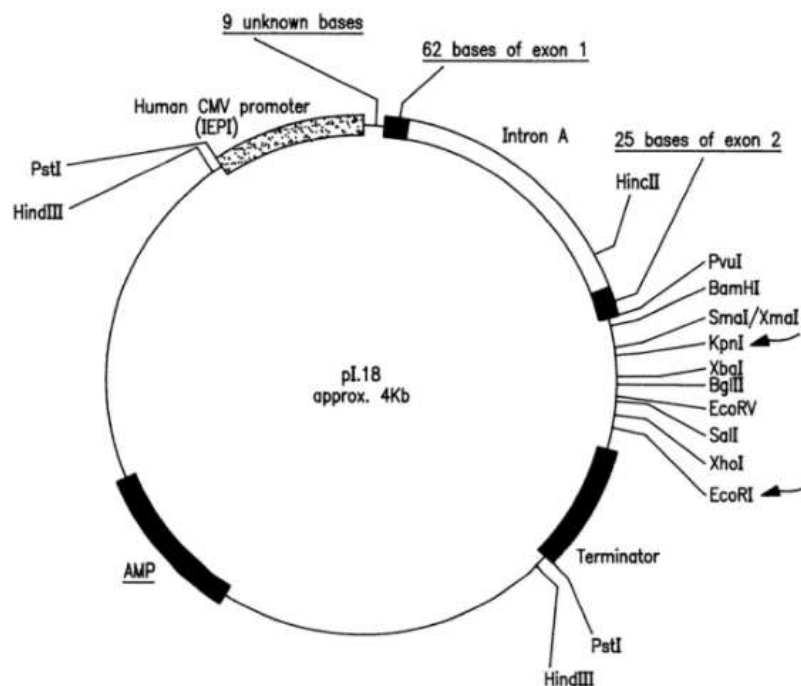
Figure 9. pI.18 mammalian expression plasmid with multiple cloning site. The plasmid was developed by I. Tarpey and N. Greenwood (US patent number US6187759 B1). The Human Cytomegalovirus (CMV) promoter facilitates expression of a gene cloned into the multiple cloning site and Intron A enhances expression. The plasmid harbours an ampicillin resistance gene (AMP) for clone selection.
