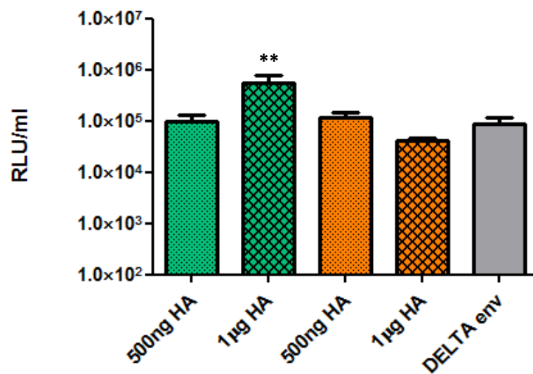
Figure 45. Testing A/canine/Guangdong/3/2011 H3-only PV production using different quantities of pl.18-HA encoding plasmid, in the presence of 250ng TMPRSS2 (green) or 250ng HAT (orange) protease plasmids. Mean PV titres are reported in relative luminescent units (RLU/ml) based on eight replicates with error bars indicating +SEM. ** Indicates a significant difference ( p < 0.05 ) determined by an unpaired T-test.
