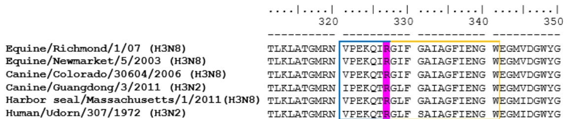
Figure 44. Alignment of H3 cleavage sites from different species; equine, canine, human and seal H3. Blue box indicates protease cleavage region with the arginine (R) cleavage site highlighted in pink. Yellow box indicates fusion peptide.
