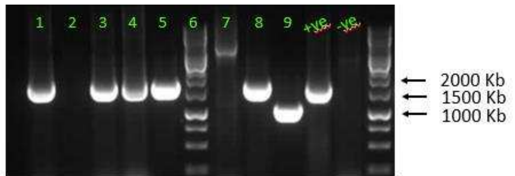
Figure 14. Colony PCR of A/equine/Newmarket/1979 HA insert in pl.18. Lanes 1, 3, 4, 5 and 8 were positive for the correct size insert at 1.7Kb. Lanes 2, 7 and 9 were negative for HA. Positive control (+ve) was A/equine/Sussex/1989 HA in pl.18 and negative control (-ve) was pl.18 cut with Bam HI and Xho I.
