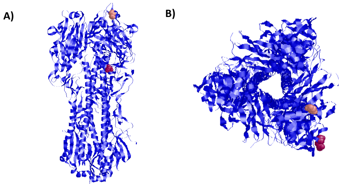
Figure 37. Trimeric HA structure of A/Newmarket/2/93 (PDB: 4UNW) highlighting amino acid residues at positions of 78 (pink) and 159 (brown), on one chain, from A) the side-view and B) top view of the protein. Protein figures edited using RasWin software (Version 2.7.5.2).
