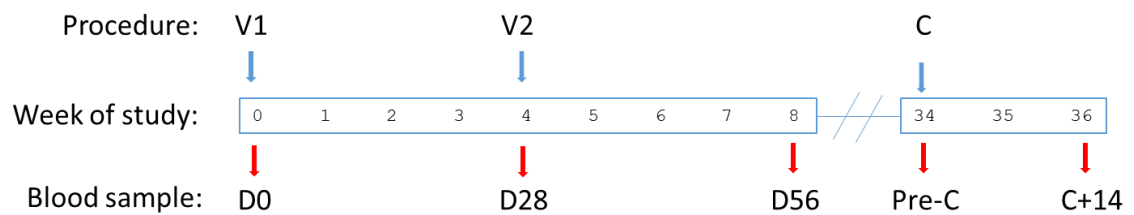
Figure 19. Timeline of study. V1, V2 = vaccination 1 and vaccination 2, C = challenge. Blood samples were collected at five time points; day 0 (D0), day 28 (D28), day 56 (D56), pre-challenge (Pre-C) and 14 days post challenge (C+14).
