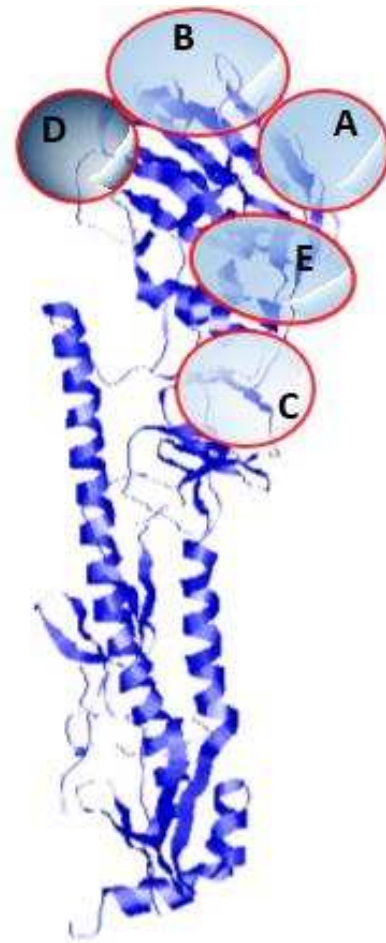
Figure 31. Illustration of a haemagglutinin monomer (PDB: 2VIU) with putative antigenic sites circled in red (A-E). Protein figure edited using RasWin software (Version 2.7.5.2) and Microsoft PowerPoint.
