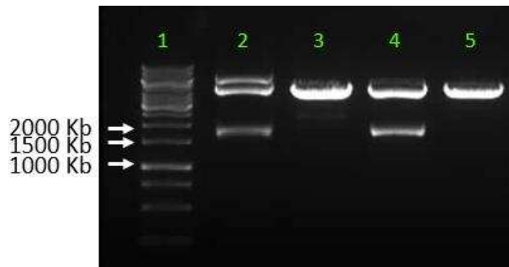
Figure 50. Plasmid digest of pl.18-HA A/harbor seal/Massachusetts/1/2011 H3 using restriction enzymes KpnI and Sall . Lanes 2 and 4 indicate positive clones. Negative control (lane 5) is pl.18 digested with KpnI and Sall .
