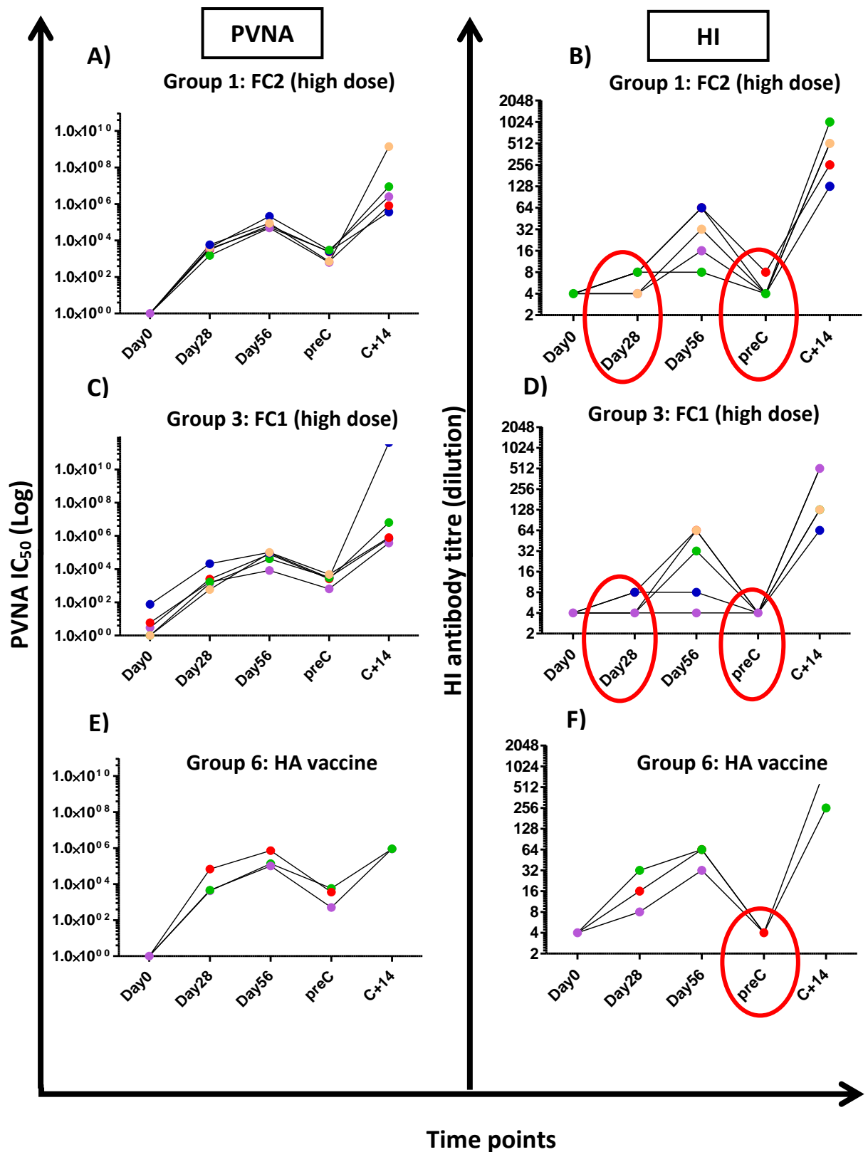
Figure 29. A-F. Neutralising antibody responses as measured by PVNA (IC 50 values) (A, C, E) compared to HI titres (dilution) (B, D, F). Responses were recorded at five different time points during the vaccine efficacy trial; Day 0, Day 28, Day 56, pre-Challenge (preC) and 14 days post challenge (C+14). Red circled data points indicate negative results from HI.
