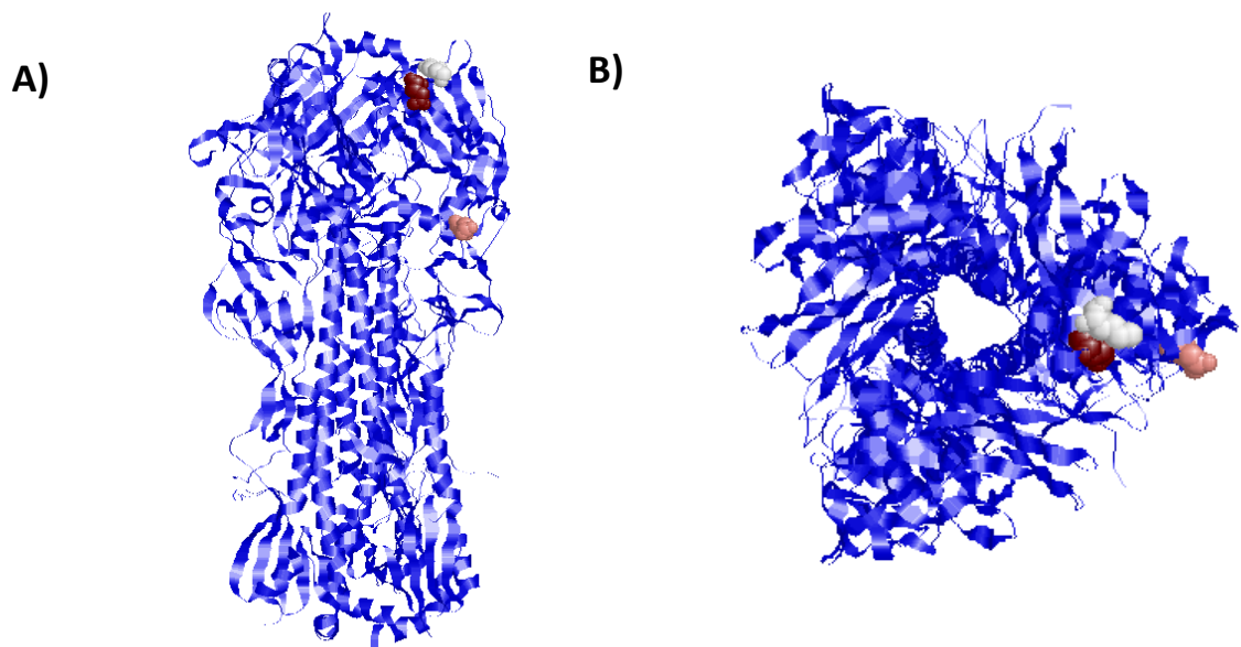
Figure 35. Trimeric HA structure of A/Newmarket/2/93 (PDB: 4UNW) highlighting amino acid residues at positions of 63 (pink), 190 (brown) and 193 (white), on one chain, from A) the side-view and B) top view of the protein. Protein figures edited using RasWin software (Version 2.7.5.2).
