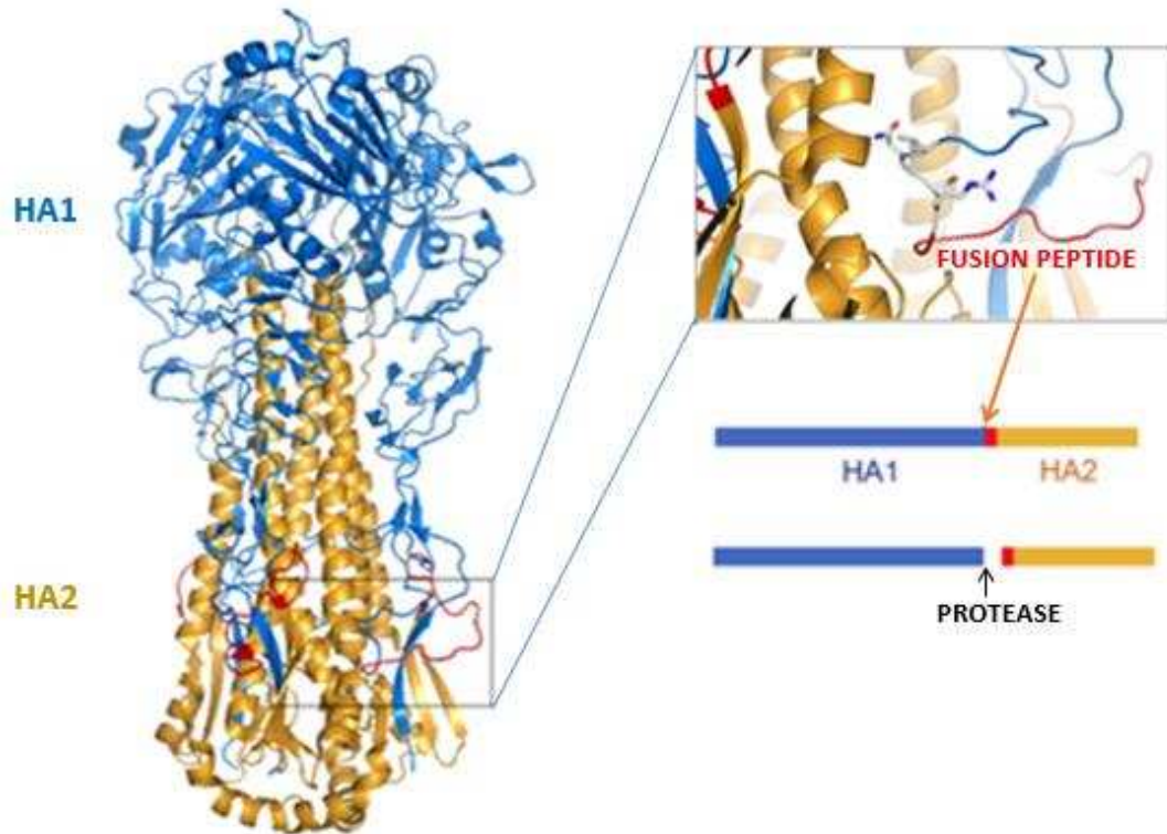
Figure 3. Cleavage of the influenza HA protein. Specific cellular proteases are responsible for cleaving the HA between HA1 and HA2 subunits and exposing the fusion peptide (modified from Hamilton et al., 2012).
