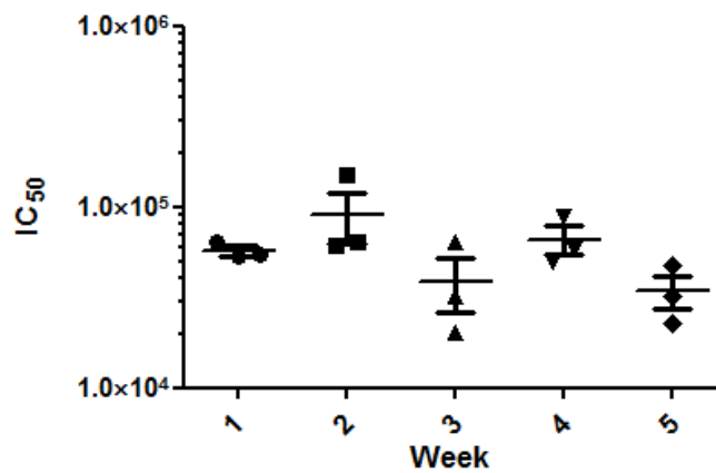
Figure 21. IC_{50} values calculated for an equine H3 positive control serum tested in triplicate against A/equine/Newmarket/1979 PV H3 PV at weekly intervals. Neat serum was added to the assay for a starting dilution of 1/40. Line with error bars represents mean with SEM.
