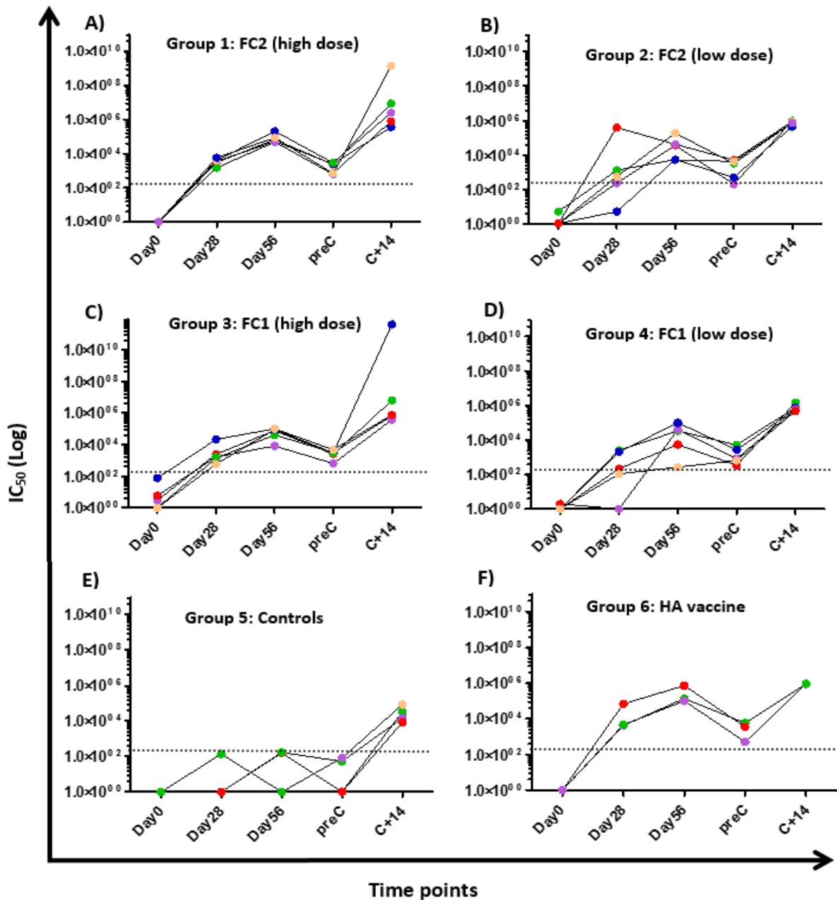
Figure 25. A-F. Neutralising antibody responses as measured by PVNA at five different time points during the vaccine efficacy trial; Day 0, Day 28, Day 56, pre-Challenge (preC) and 14 days post challenge (C+14). . Pony groups; A) FC2 (high dose), B) FC2 (low dose), C) FC1 (high dose), D) FC1 (low dose), E) controls and F) HA vaccine group. Antibody responses were recorded as IC 50 values (reciprocal value of the serum dilution at which 50% neutralisation of the PV was reached). The positive response threshold is indicated by the dotted line at a LogIC 50 of 2.20. Coloured data points represent different ponies.
