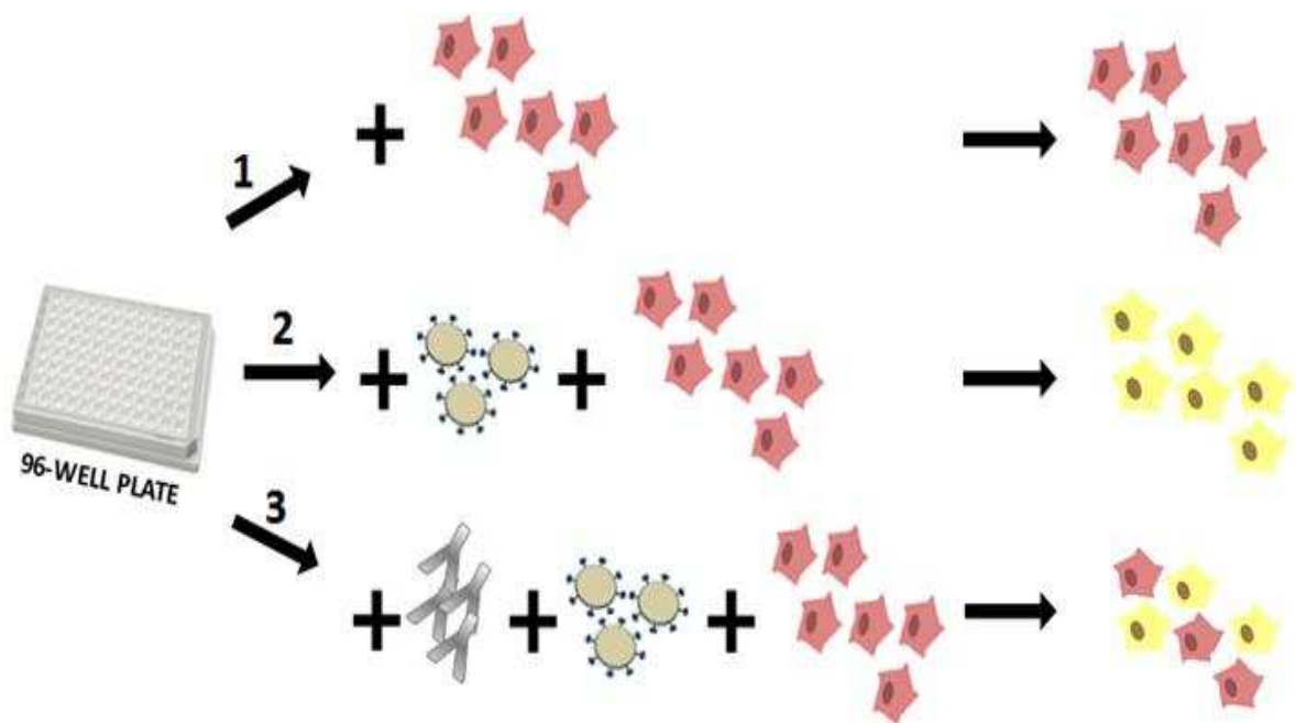
Figure 8. Principles of the pseudotype virus neutralisation assay using the luciferase reporter gene. 1 – Target cells alone do not luminesce. 2 – Virus added to target cells, the virus infects target cells and the reporter gene is integrated into the cell genome causing cells to luminesce. 3 – Upon addition of antisera containing antibodies directed against the HA, the influenza pseudotyped virus is prevented from transducing target cells thus infection is reduced and the luminescence measured, decreases (Kinsley et al. , 2016).
