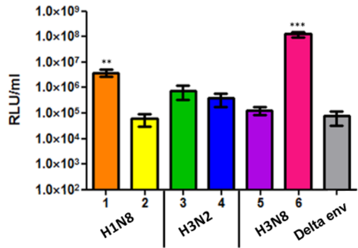
Figure 53. H1N8, H3N2 and H3N8 combination PVs. Mean PV titres generated by co-transfection with different HA and NA plasmids (Table 27 contains HA and NA strains for PVs 1-6). Delta envelope (env) was generated as a negative control. PV titres reported in relative luminescent units (RLU/ml), +/- SEM of eight replicates. Statistically significant differences (Mann-Whitney test) between mean RLU/ml of each HA/NA combination PV and the Delta env control are indicated by ** = p < 0.01 ; *** = p < 0.001 .
