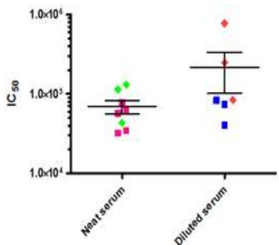
Figure 23. Comparison of IC_{50} values using different starting dilutions of serum; neat and diluted (pre-diluted 1/10).
