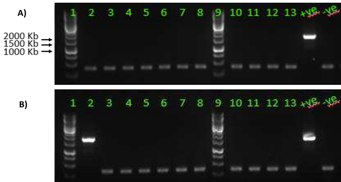
Figure 17. Colony PCR of pl.18-N8 equine (from A/equine/Richmond/1/2007 H3N8). Lanes 2-13 (A) are 1:1 molar ratio ligations, all negative for N8 gene. Lanes 2-13 (B) are 1:3 molar ratio ligations, with a positive clone in lane 2. Positive control (+ve) is A/chicken/Italy/1067/1999 N1 in pl.18 and negative control (-ve) was pl.18 digested with Bam HI/ Xho I.
