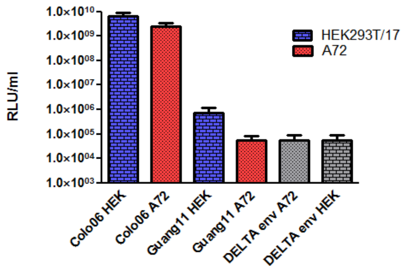
Figure 46. Titration of A/canine/Colorado/30604/2006 H3 PV (Colo06) and A/canine/Guangdong/3/2011 H3 PV (Guang11) using two different target cell lines; HEK293T/17 (HEK in blue) and A72 (red). Delta env negative control was also titrated on both cell lines. Mean PV titres are reported in relative luminescent units (RLU/ml) based on eight replicates with error bars indicating +SEM.
