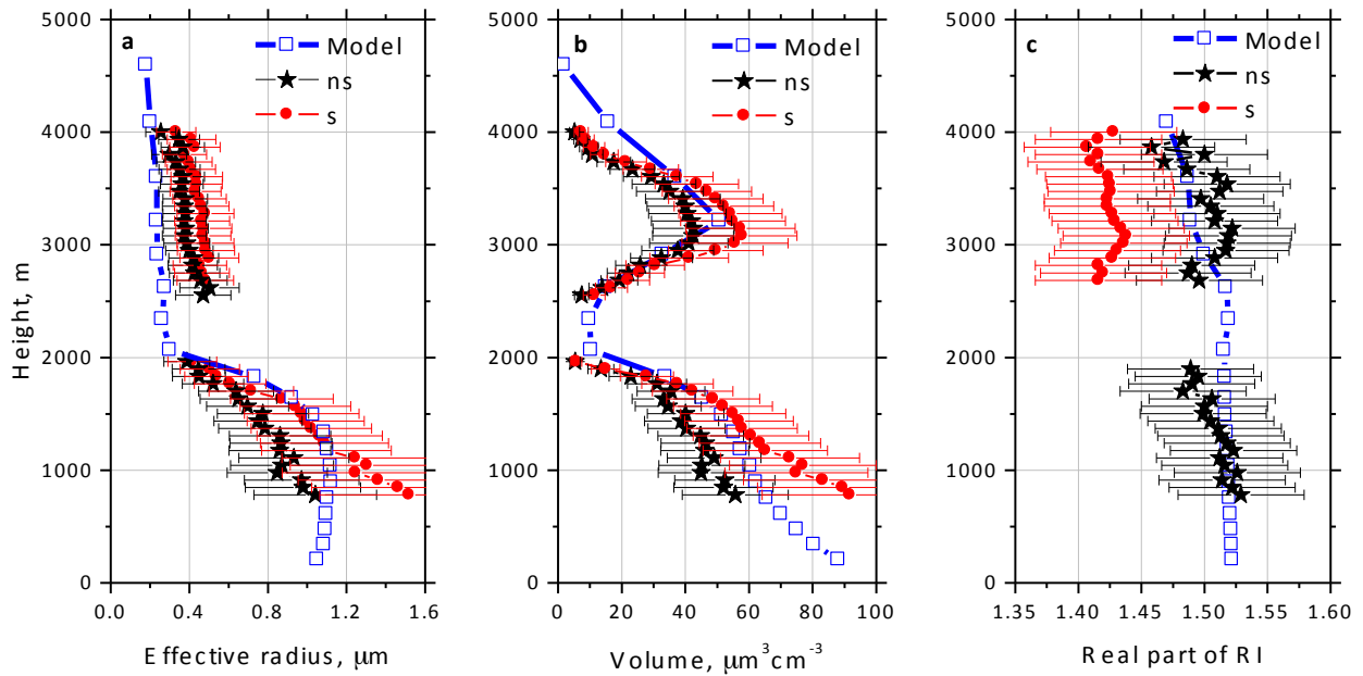
4 5 Fig.18. Profiles of (a) effective radius, (b) particle volume and (c) real part of the refractive index 6 on 24 December 2015 retrieved from 3\sigma+2\alpha lidar measurements shown in Fig.7a (solid 7 symbols) and provided by MERRA-2 for 21:00 UTC (open symbols). Inversion of lidar 8 measurements was performed in assumption of spherical particles (s) and using the model of 9 spheroids (ns).
