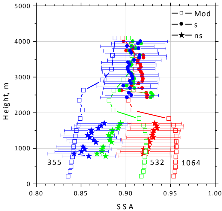
Fig.19. The single scattering albedo at 355 nm (blue), 532 nm (green) and 1064 nm (red) on 24 December 2015 retrieved from 3\sigma+2\alpha lidar measurements shown in Fig.7a (solid symbols) and provided by the MERRA-2 model for 21:00 UTC (line + open symbols). For inversion of lidar data the spheroids (ns) were used below 2000 m and spheres (s) above 2000 m.
