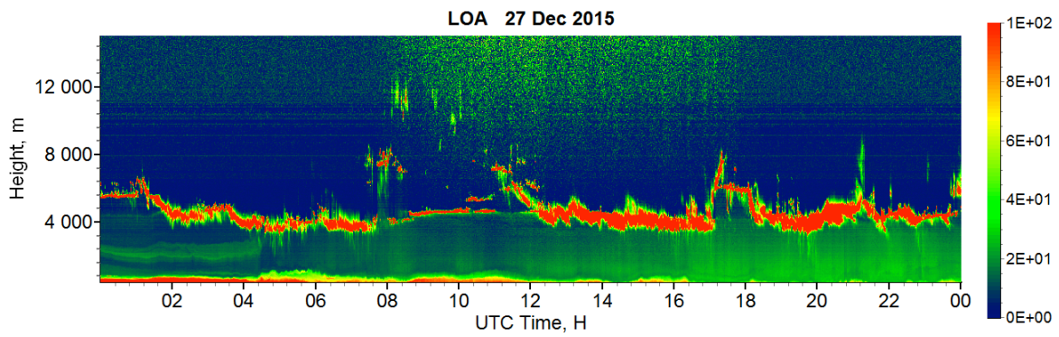
6 Fig.2. Range corrected lidar signal (in arbitrary units) of Cimel MPL for 24 - 27 December 2015.
