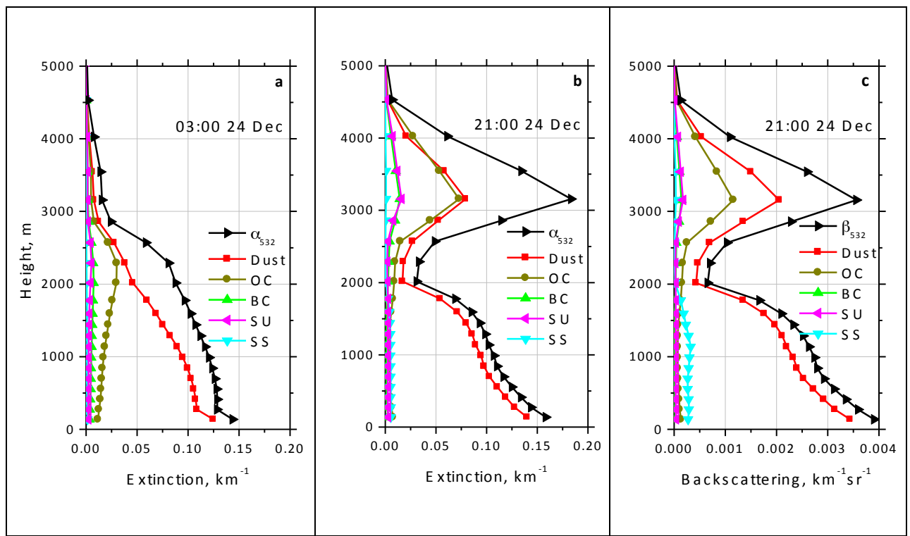
Fig.12. Vertical profiles of extinction coefficients at (a) 03:00 UTC, (b) 21:00 UTC and (c) backscattering coefficients at 21:00 UTC on 24 December 2015 from MERRA-2 model at 532 nm. Profiles are given for five aerosol components: dust, black carbon (BC), organic carbon (OC), sea salt (SS), sulfates (SU) together with total extinction \alpha_{532} and backscattering \beta_{532} .
