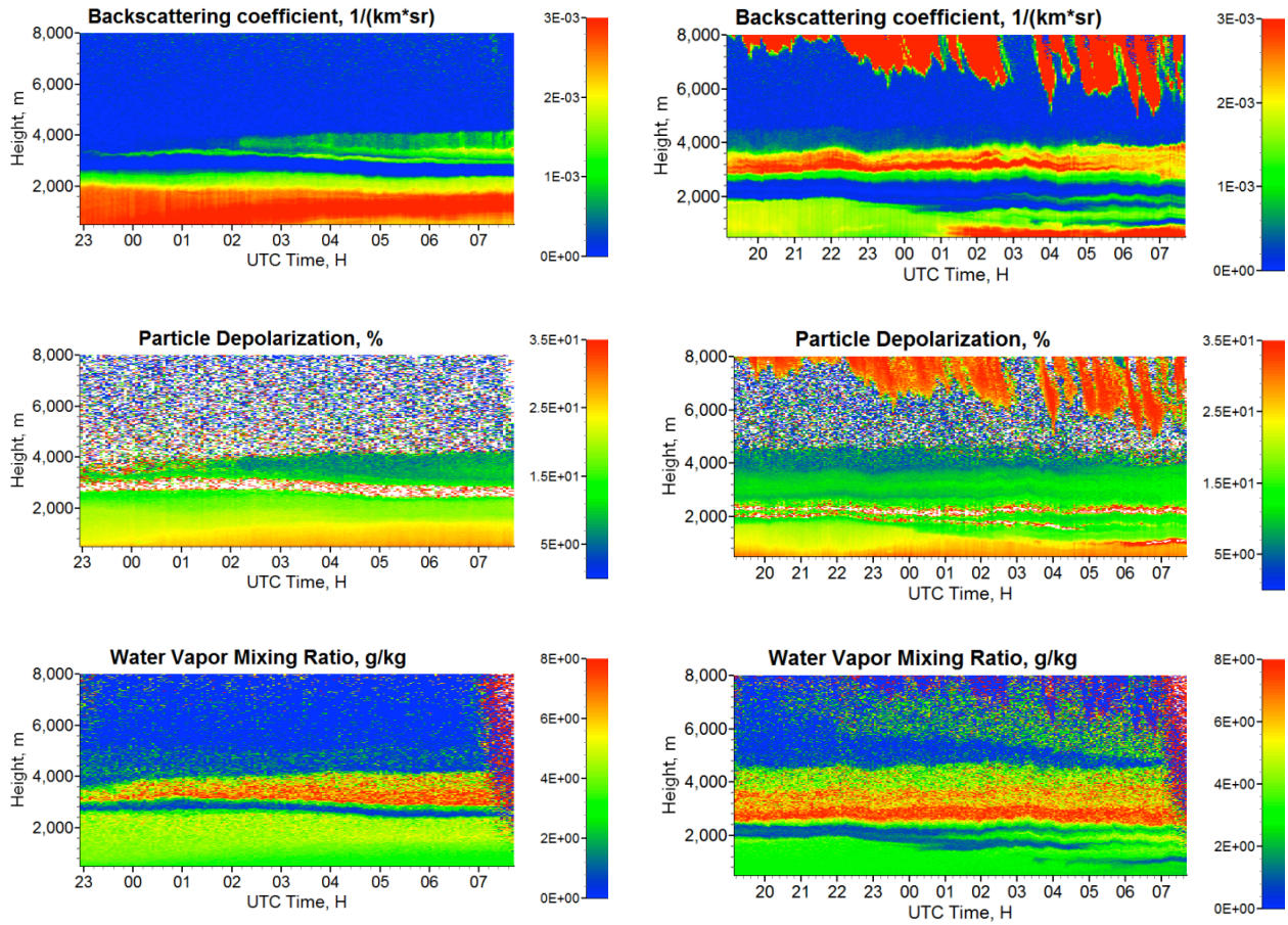
2 Fig.3 Height-temporal distributions of the backscattering coefficient and particle depolarization 3 ratio at 532 nm together with the water vapor mixing ratio derived from the Raman lidar 4 measurements on the nights 23-24 (left column) and 24-25 December 2015 (right column). 5
