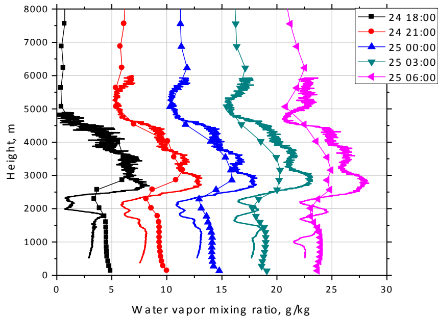
Fig.17. Water vapor mixing ratio derived from Raman lidar measurements (solid line) and obtained from the model (line + symbols) on the night 24-25 December 2015. Temporal intervals are the same as in Fig.13. The profiles are shifted relatively each other by 5 g/kg.
