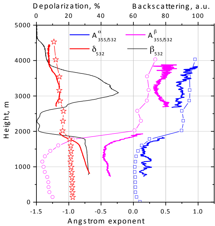
Fig.16. Extinction ( A_{355/532}^\alpha ) and backscattering ( A_{355/532}^\beta ) Ångström exponents together with the particle depolarization ratio \delta_{532} obtained from lidar measurements (line) and from MERRA-2 modeling (line + symbols). Lidar data are averaged over 19:00 – 23:00 UTC period while model data are given for 21:00 UTC.
