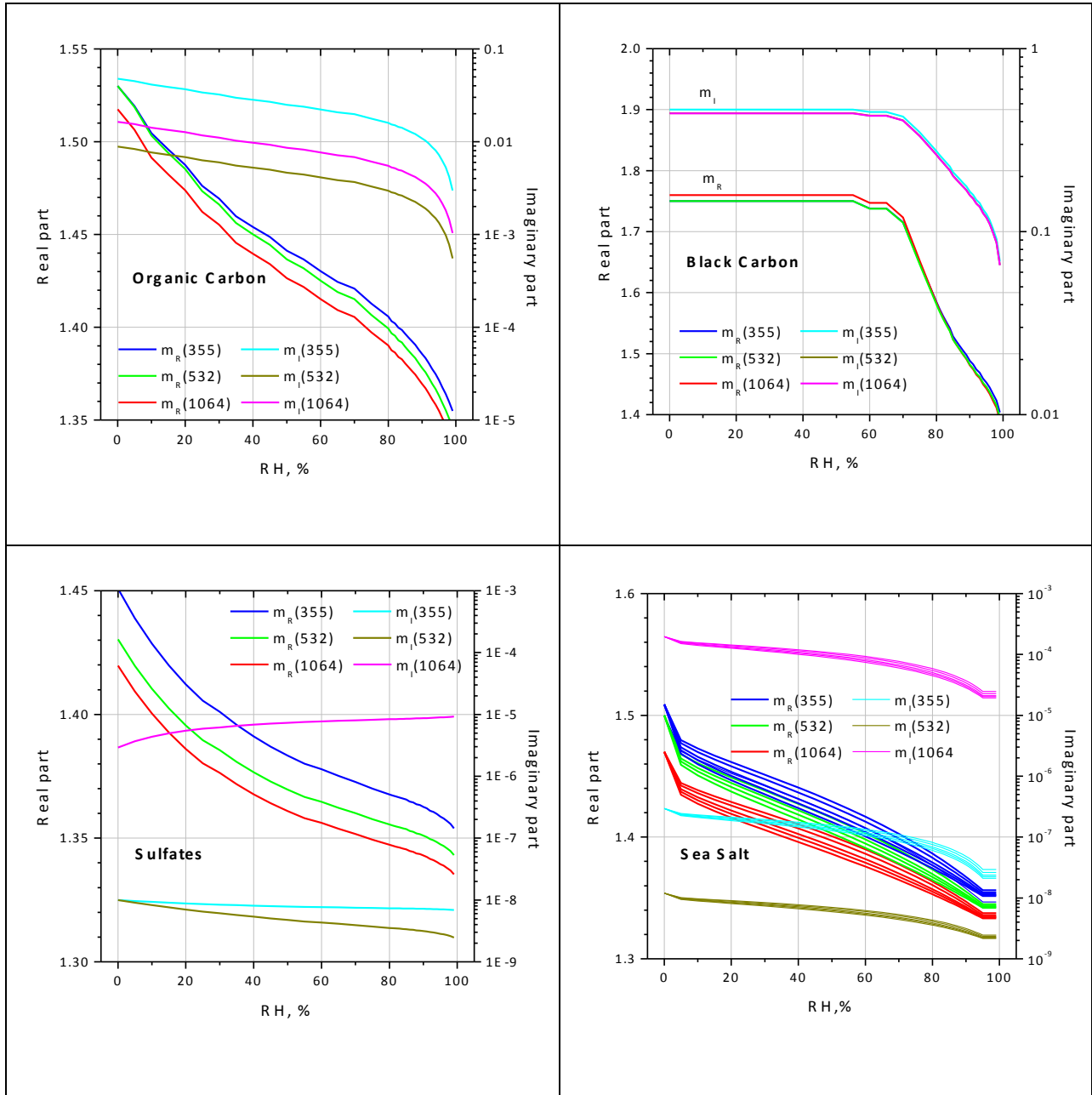
3 Fig.A2. Dependence of the real and imaginary part of the refractive index of organic carbon, 4 black carbon, sulfates and sea salt on relative humidity (RH) used in the MERRA-2 model. For 5 the sea salt the results are given for five size bins from Table 1. Both m_R and m_I decrease with 6 bin number increasing.
