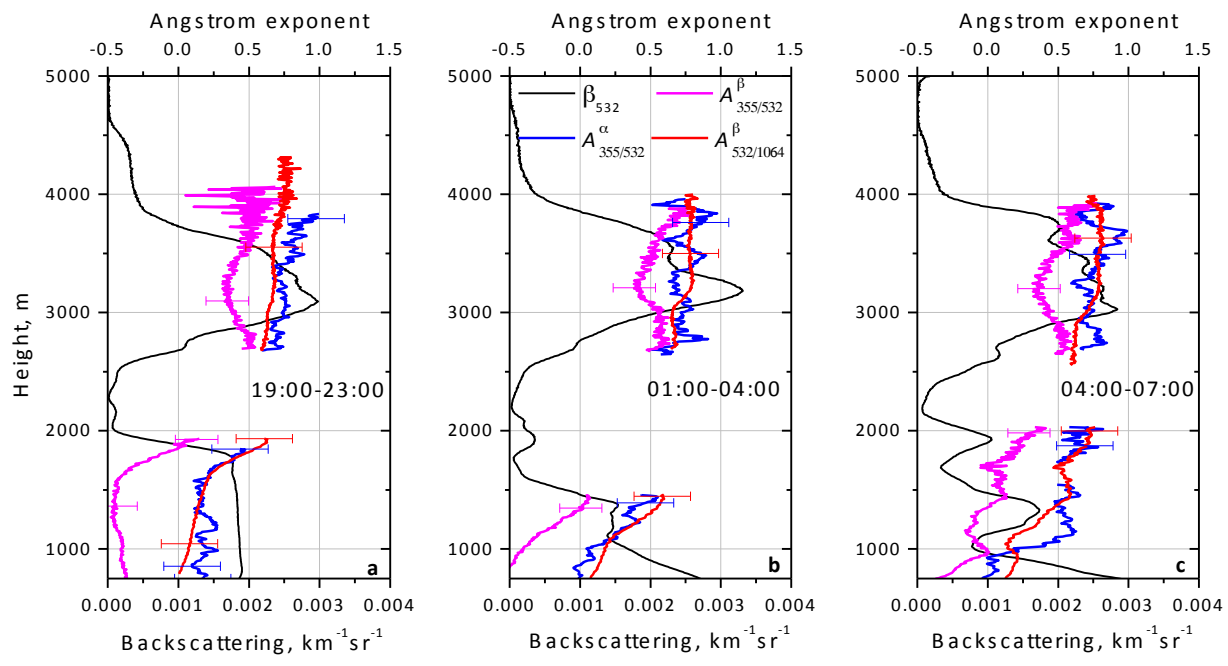
3 Fig.8 Extinction ( A_{355/532}^\alpha ) and backscattering ( A_{355/532}^\beta, A_{532/1064}^\beta ) Ångström exponents together 4 with backscattering coefficient \beta_{532} for the same three temporal intervals as in Fig.7. 5
