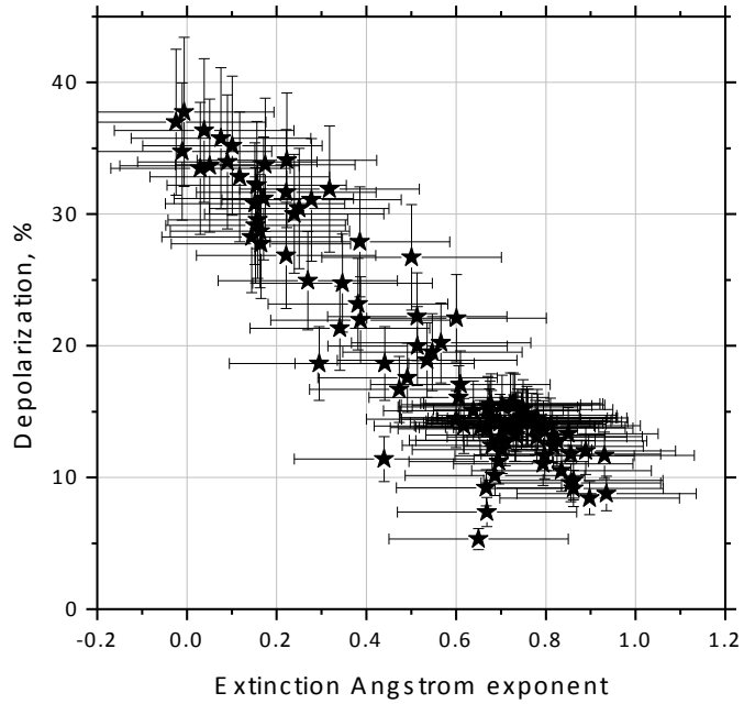
3 4 Fig.10. Particle depolarization ratio as a function of the extinction Ångström exponent derived 5 from data shown in Fig.7, 8. 6 7
