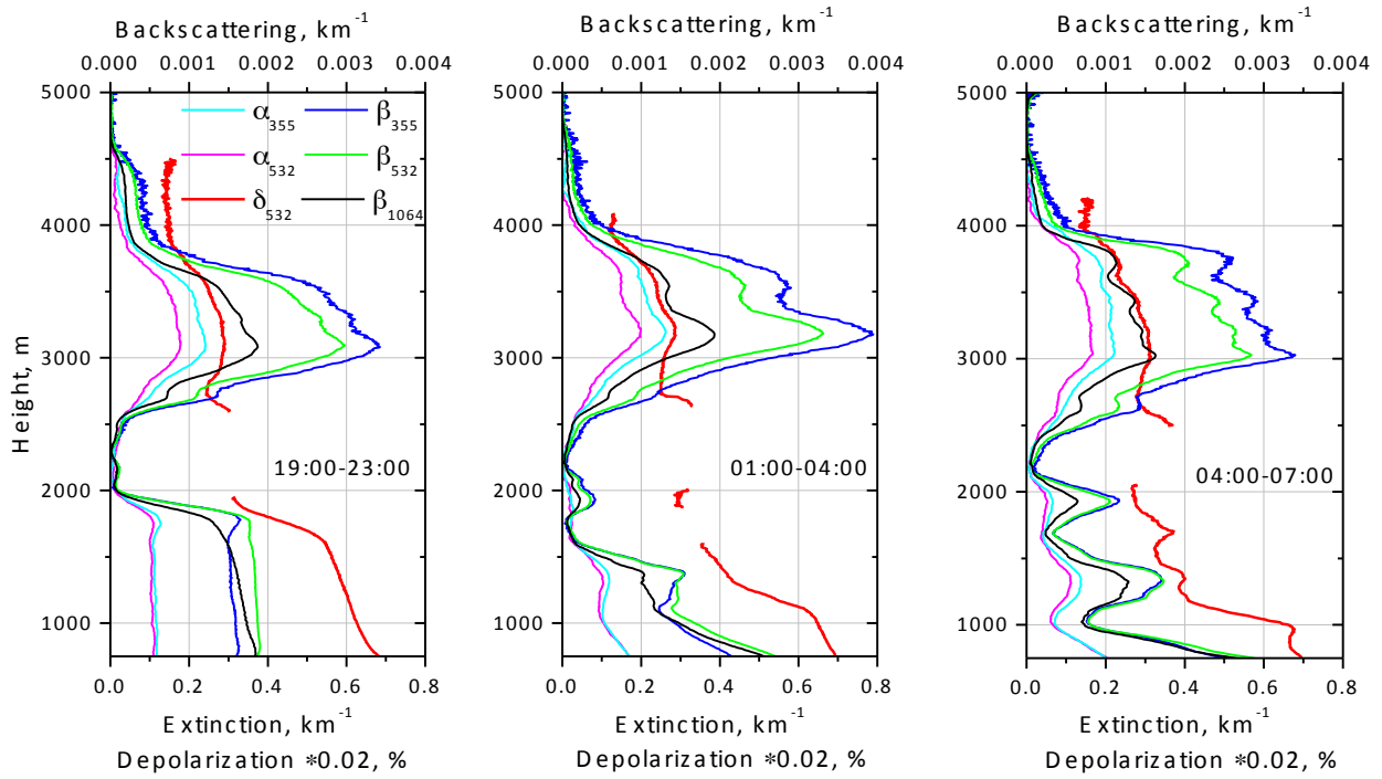
3 Fig.7. Vertical profiles of the aerosol backscattering ( \beta_{355} , \beta_{532} , \beta_{1064} ) and extinction ( \alpha_{355} , 4 \alpha_{532} ) coefficients together with the particle depolarization ratio ( \delta_{532} ) for three temporal 5 intervals: 19:00-23:00, 01:00-04:00 and 04:00-07:00 UTC on 24-25 December 2015. The values 6 of \delta_{532} are multiplied by factor 0.02.
