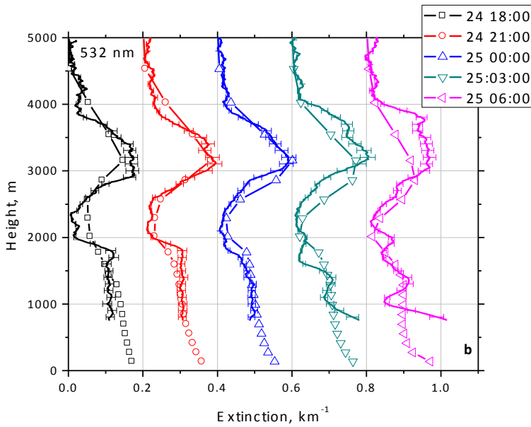
4 Fig.13. Comparison of extinction profiles at (a) 355 nm and (b) 532 nm derived from Raman 5 lidar measurements (line) and modeled by MERRA-2 (line + symbols) on the night 24-25 6 December 2015. Model profiles are provided at 18:00, 21:00, 00:00, 03:00, 06:00 UTC. The 7 lidar measurements are given for temporal intervals centered at: 19:00, 21:00, 00:00, 03:00,
