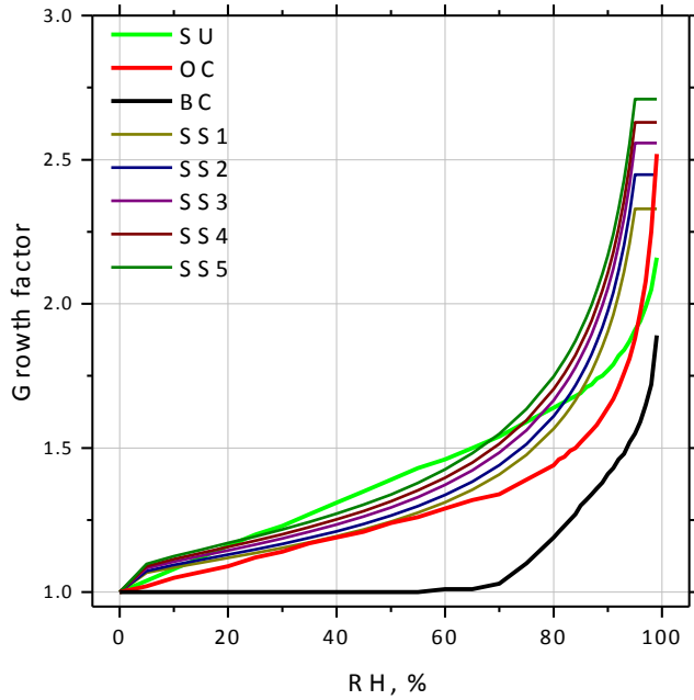
Fig.A1. Dependence of the growth factor of organic carbon, black carbon, sulfates and sea salt on relative humidity (RH) used in MERRA-2. For the sea salt the results are given for five size bins from Table 1. The growth factor increases with increase of bin number.
