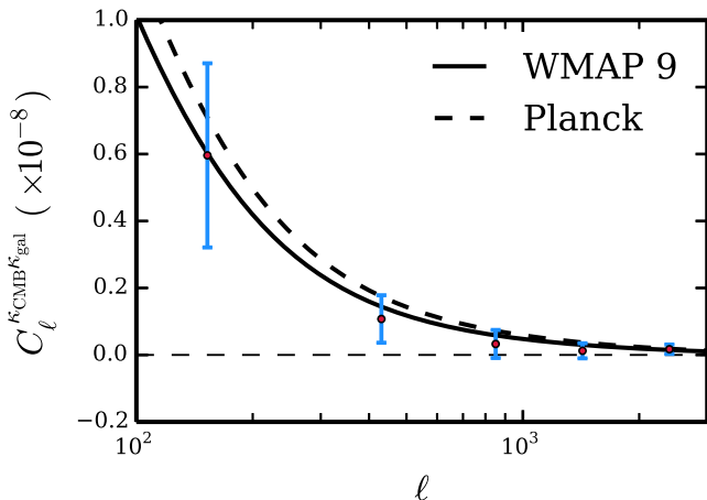
FIG. 4. The CMB lensing - galaxy lensing convergence cross power spectrum (red points), measured using ACT and CS82 data. Error bars are computed using Monte Carlo methods (see text), and the significance of the measurement is 3.2\sigma . The dashed and solid black lines show the expected power spectra assuming the Planck + lensing + WP + highL and WMAP9 + eCMB cosmological models, respectively. The theoretical spectra shown correspond to A = 1 , and relative to these models, the best-fit amplitudes to our data are A^{\text{Planck}} = 0.61 \pm 0.19 and A^{\text{WMAP}} = 0.74 \pm 0.23 .
