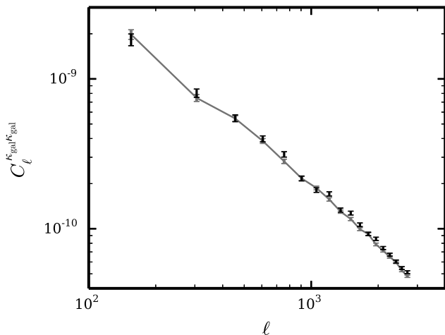
FIG. 3. The auto power spectrum of simulated galaxy lensing convergence maps constructed using source galaxies at z = 0.73 . The gray points connected by the solid line mark the input auto spectrum, while the overlaid black points show the spectrum recovered from the analysis pipeline.
