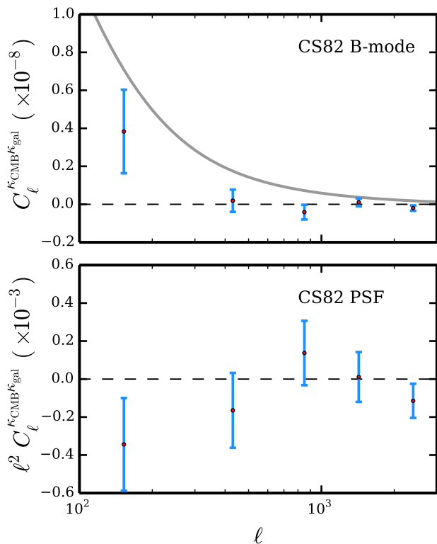
FIG. 6. Two tests of the CS82 lensing data, both consistent with zero. The data points show the correlations between the ACT data and the CS82 B-mode ellipticity data (top) and the PSF ellipticity data (bottom). The probabilities to exceed the measured \chi^2 for these tests are 27% and 46%, respectively. The solid line in the top panel shows the expected CMB lensing - galaxy lensing cross spectrum using Planck parameters (as in Fig. 4) for comparison with the null test data points. Note that the quantity \ell^2 C_\ell is plotted in the bottom panel in order to increase the dynamic range of the plot.
