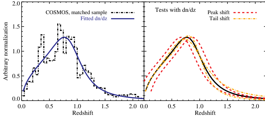
FIG. 2. Redshift distribution of CS82 source galaxies. Left: redshift distribution for a matched sample of galaxies from the COSMOS survey. The blue solid line indicates our fit to the COSMOS matched sample. Right: we test how the amplitude of the theoretical lensing-lensing cross power spectrum changes when we vary the peak of the dn/dz (red, dashed lines) and the high-redshift tail of the distribution (orange, dash-dotted lines). These variations in the dn/dz lead to changes of order 10 – 20% in the amplitude of the theoretical lensing-lensing cross power spectrum. Accurate estimates of dn/dz will be crucial for this kind of cross-correlation in the future.
