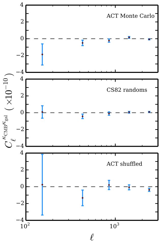
FIG. 5. Three successful null tests, all consistent with zero. Top: the mean correlation between 480 Monte Carlo realizations of simulated CMB lensing maps and the true CS82 lensing data. Middle: the mean correlation between 500 randomized galaxy lensing maps and the true ACT data. Bottom: the mean correlation between the true CS82 data and 58 ACT “shuffled” maps, constructed by shifting the data in intervals of 0.75^\circ along the right ascension direction. The probabilities to exceed the measured \chi^2 for these tests are 7.4%, 39% and 30%, respectively. Note that the scaling of the y -axis here is two orders of magnitude smaller than the y -axis of Fig. 4.
