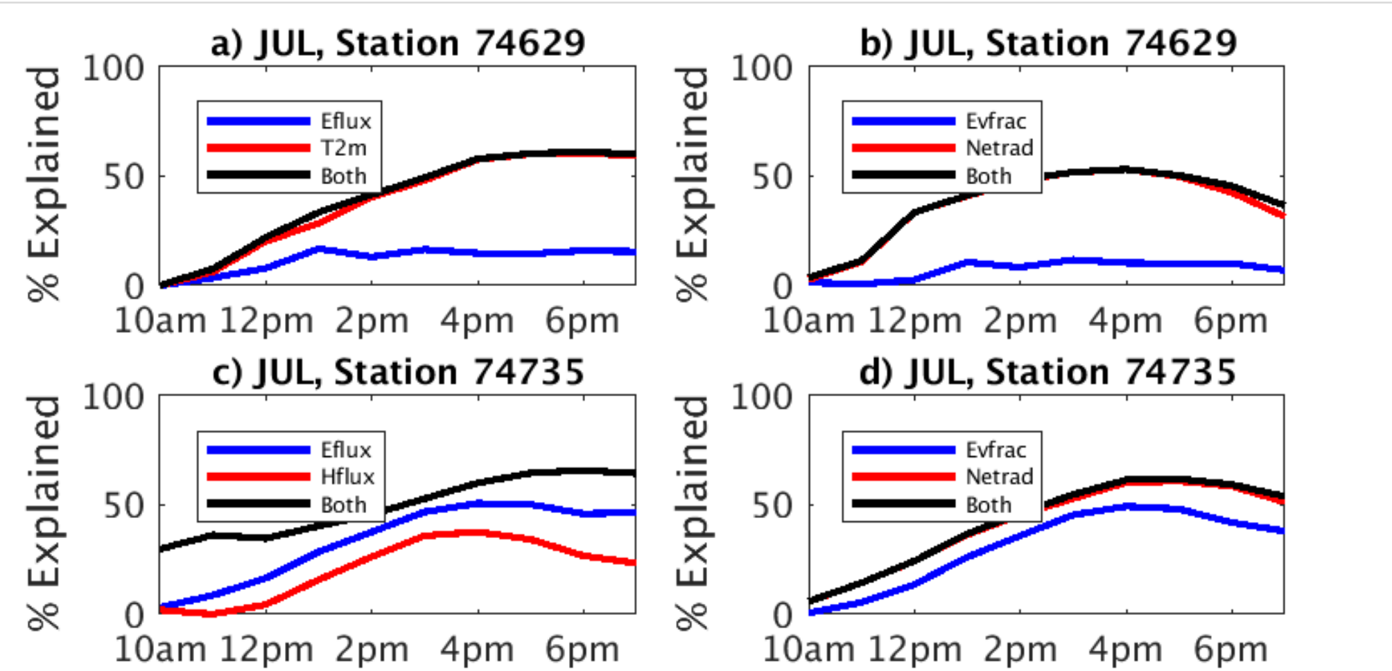
Figure 4 a) Fraction of total PBL height variance explained by latent heat flux, 2-meter temperature, and both at Station 74629 in July, b) fraction explained by evaporative fraction, net surface radiation and both at Station 74629 in July, c) fraction explained by latent heat flux, sensible heat flux and both at Station 74735 in July, d) fraction explained by evaporative fraction, net surface radiation and both at Station 74735 in July.
