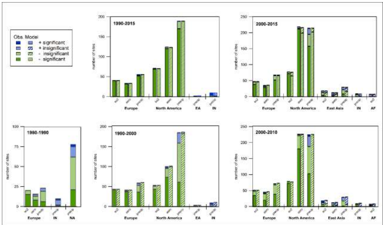
Figure S2. Number of sites with significant and insignificant trends, observed and modeled (EMEP/MSW) for different time periods. NA=North America, EA=East Asia, IN=India, AF=Africa. Note that for the ten year periods the model only have three points (five year interval) and cannot detect significance or not.
