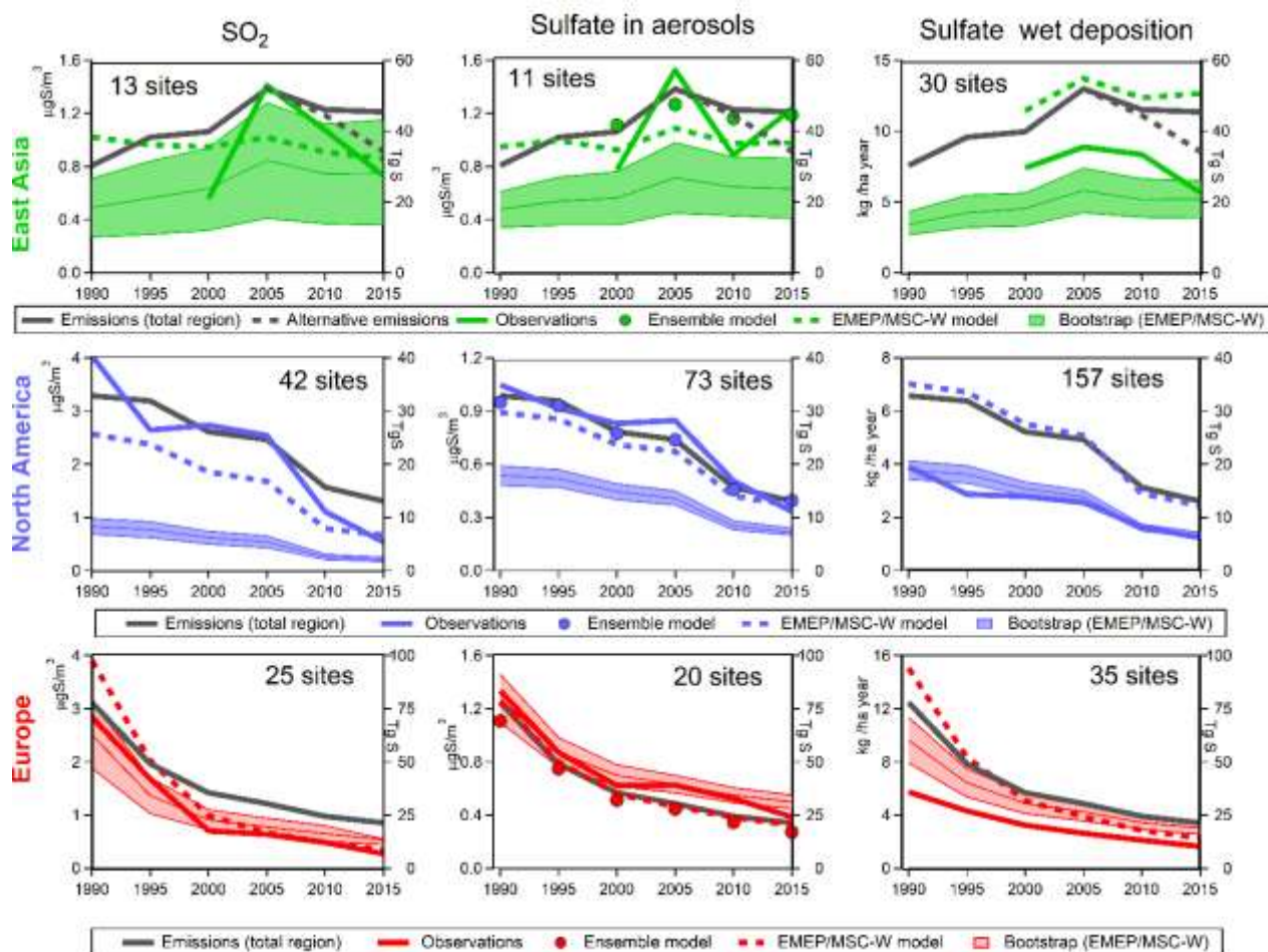
Figure S3. Trends in \text{SO}_2 , sulfate in aerosols and in wet deposition in East Asia, North America and Europe from observations and the EMEP/MSC-W model (and Ensemble model for sulfate in aerosols) at the selected number of sites, and the average bootstrap trends and standard deviations from 1000 iterations. Observed and modelled concentrations are given on the y-axis on the left, while emissions on the right. For East Asia an alternative emission development the last ten years are included, based on more recent inventories 7,8 .
