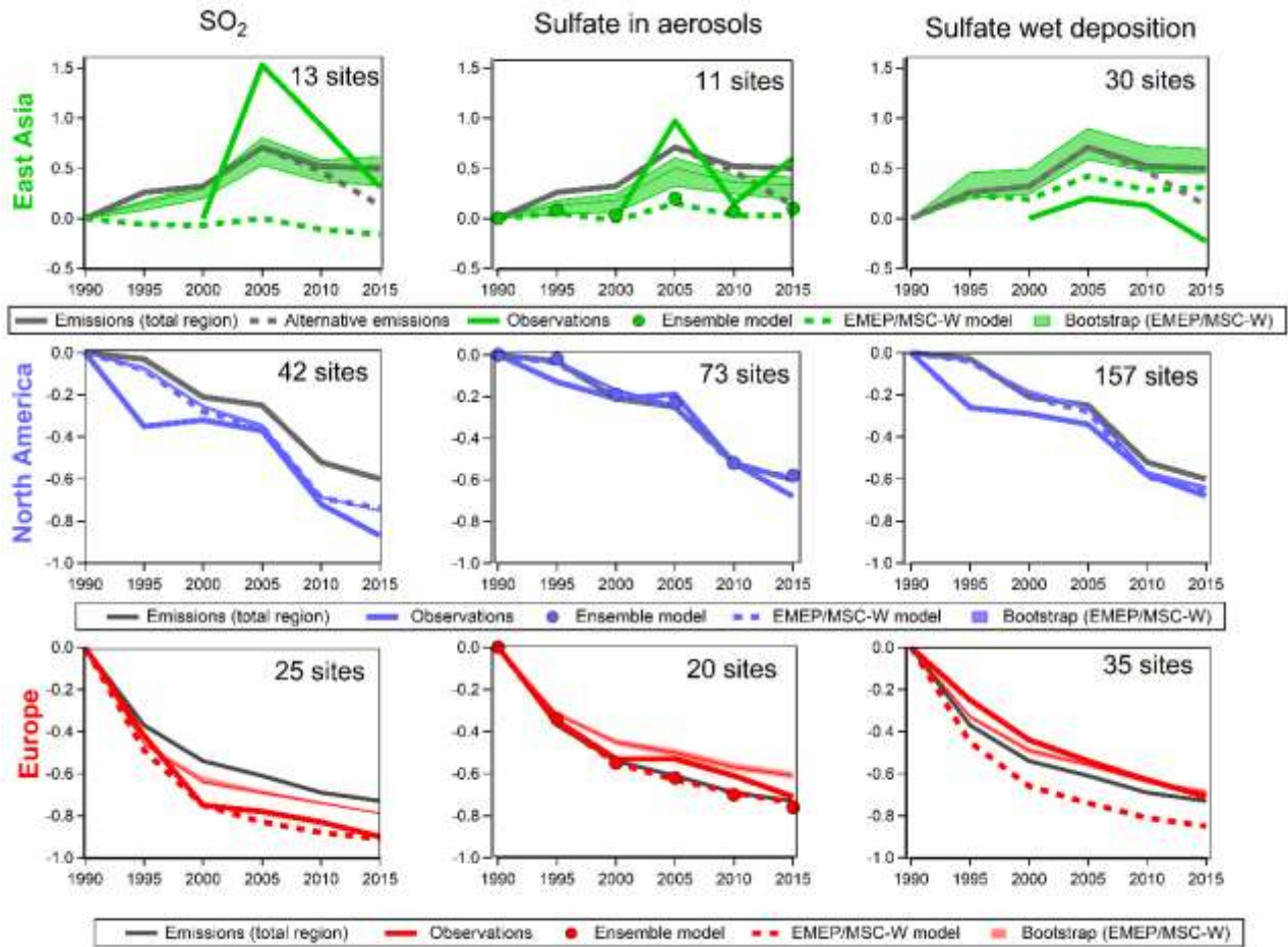
Figure S4. Normalised trends of SO_2 , sulfate in aerosols and in wet deposition in East Asia, North America and Europe in observation and EMEP/MSC-W model (and Ensemble model mean for sulfate in aerosols) at the selected number of sites, and the average bootstrap trends and standard deviations from 1000 iterations. For East Asia an alternative emission development the last ten years are included, based on more recent inventories 7,8 .
