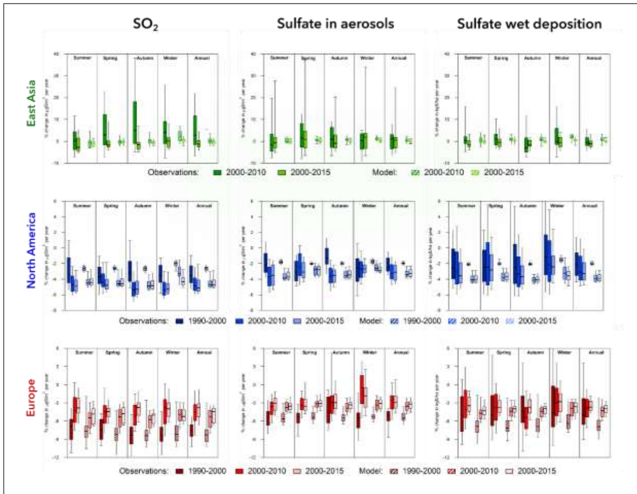
Figure S5. Box plot indicating 10, 25, 50, 75 and 90 percentiles of the seasonal and annual observed and modelled trends (EMEP/MSC-W model for SO 2 and wet deposition of sulfate; ensemble models for sulfate in aerosols) for different time periods.
