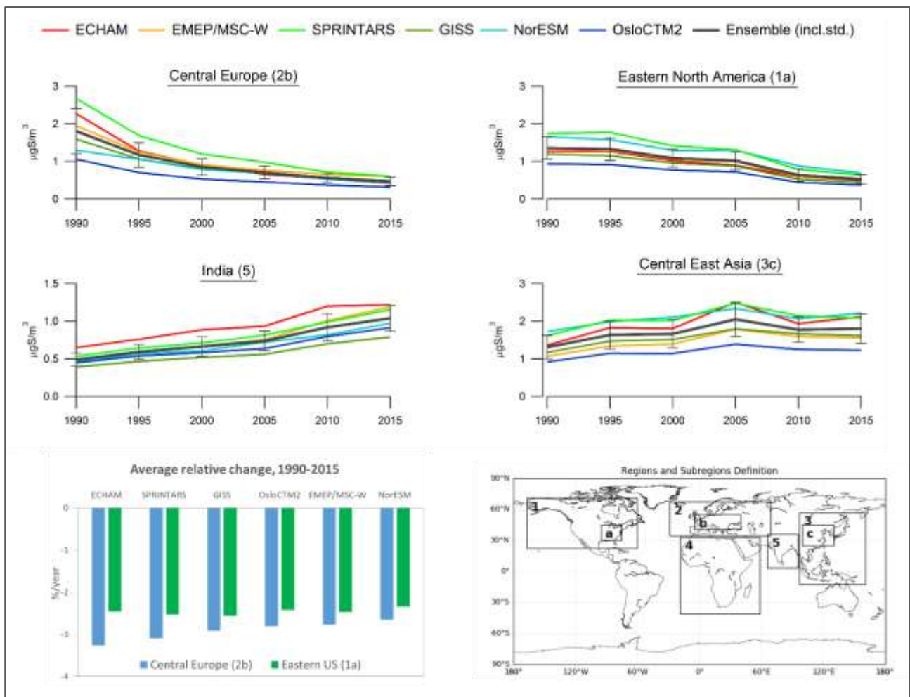
Figure S6. Comparison of the average concentrations and total relative change of modelled sulfate concentrations in aerosols for the period 1990-2015, calculated by the different global models for the different (sub)regions indicated in the bottom right map
