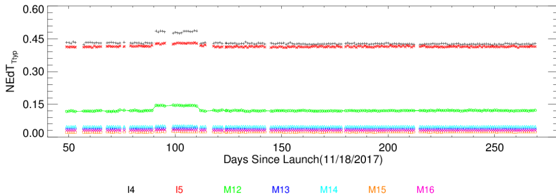
Figure 6. Long-term trending of the NEdT_{Typ} .
