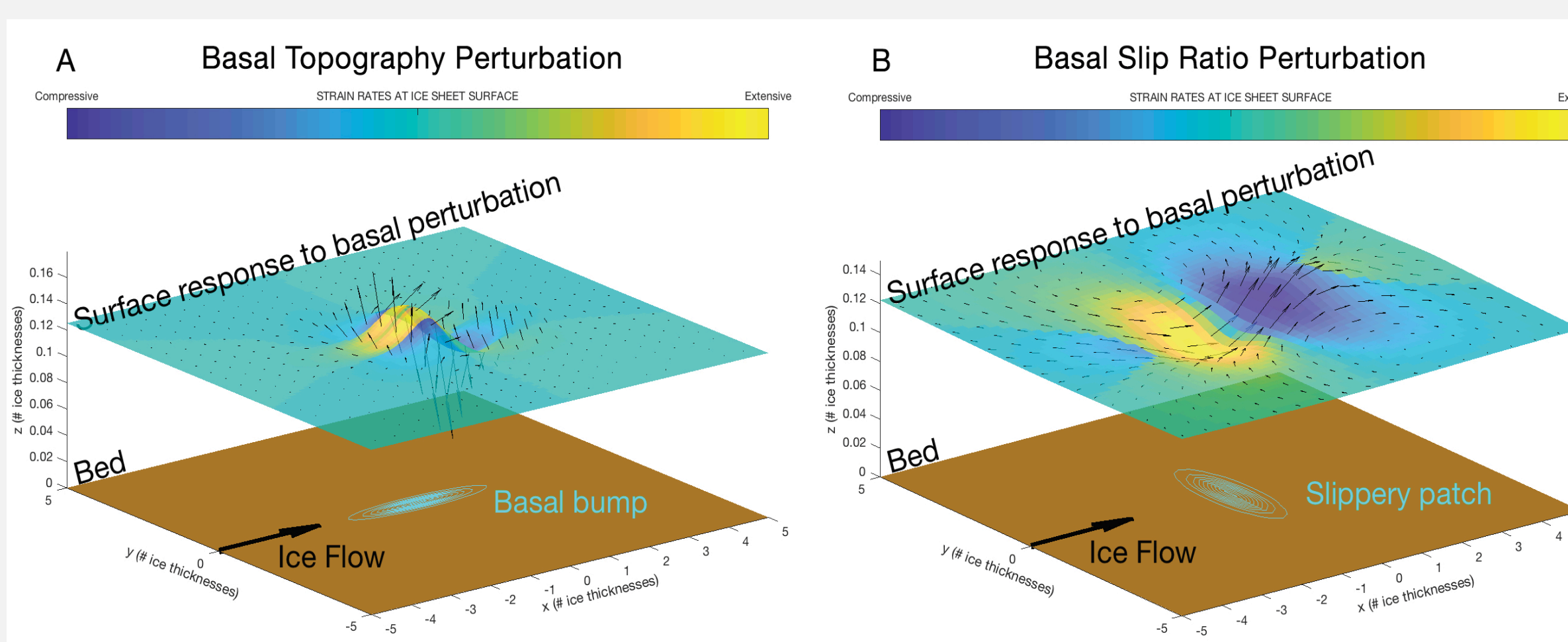
Illustration of the analytic model for the ice-sheet surface response (top surface) to a basal slipperiness perturbation. Ice flow is from left to right. Ice flow is extensive upstream of the slippery patch; this region may seed crevasses.
