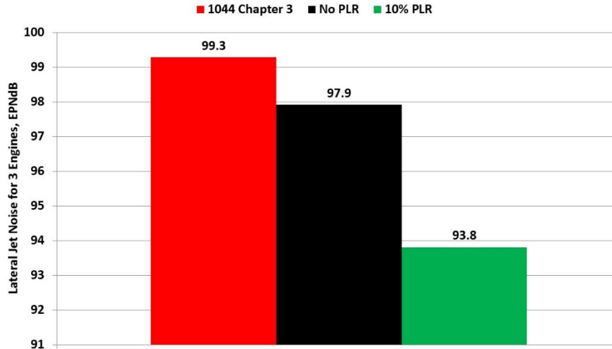
Figure 14.—Effective perceived jet noise levels, three engines on 1044-like aircraft for offset nozzles, NPR_c = 1.8 , NPR_b = 1.8 , NPR_t = 1.6 , NTR_c = 3.0 , and A_b/A_c = 2.5 .
