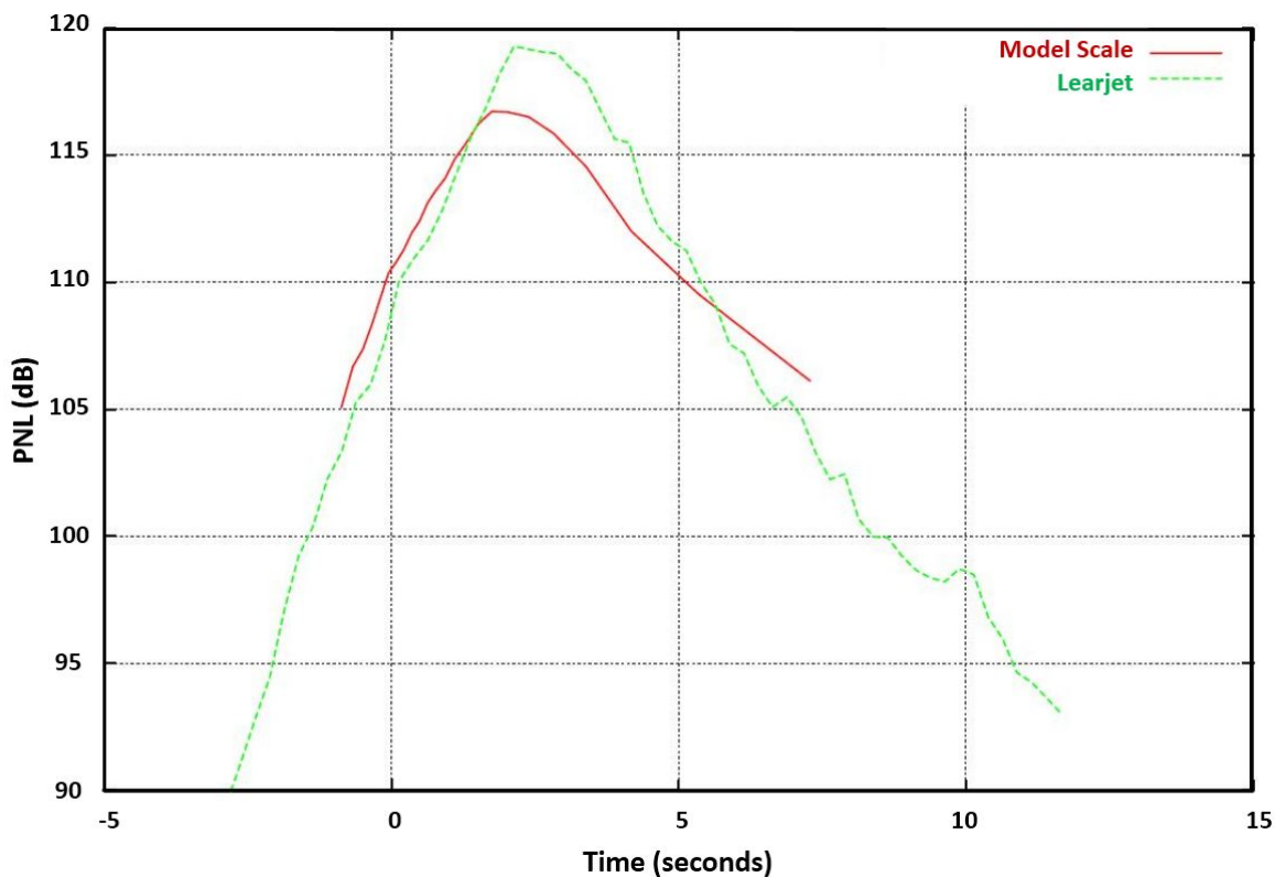
Figure 9.—Perceived noise levels for model scale nozzles tested in NATR and flight tests measurements on a Learjet.
