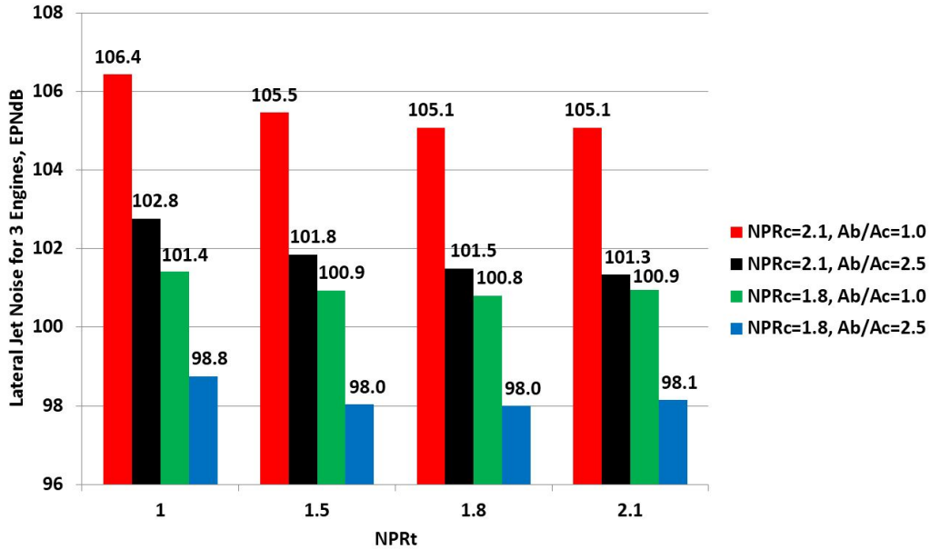
Figure 12.—Perceived noise levels for 3 engines with offset nozzles on a 1044-like aircraft for selected values of NPR c , NPR t , and Ab/Ac.
