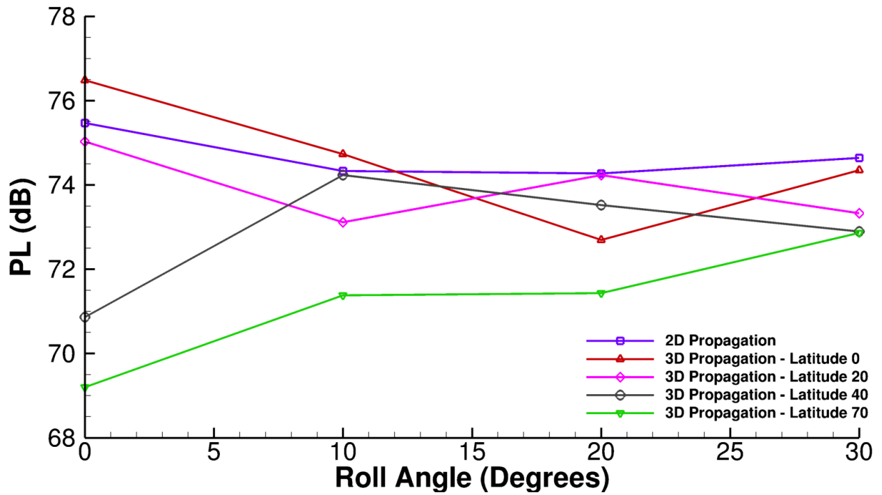
Fig. 8 Impact of ellipsoidal Earth effects on perceived loudness under arbitrary winds
