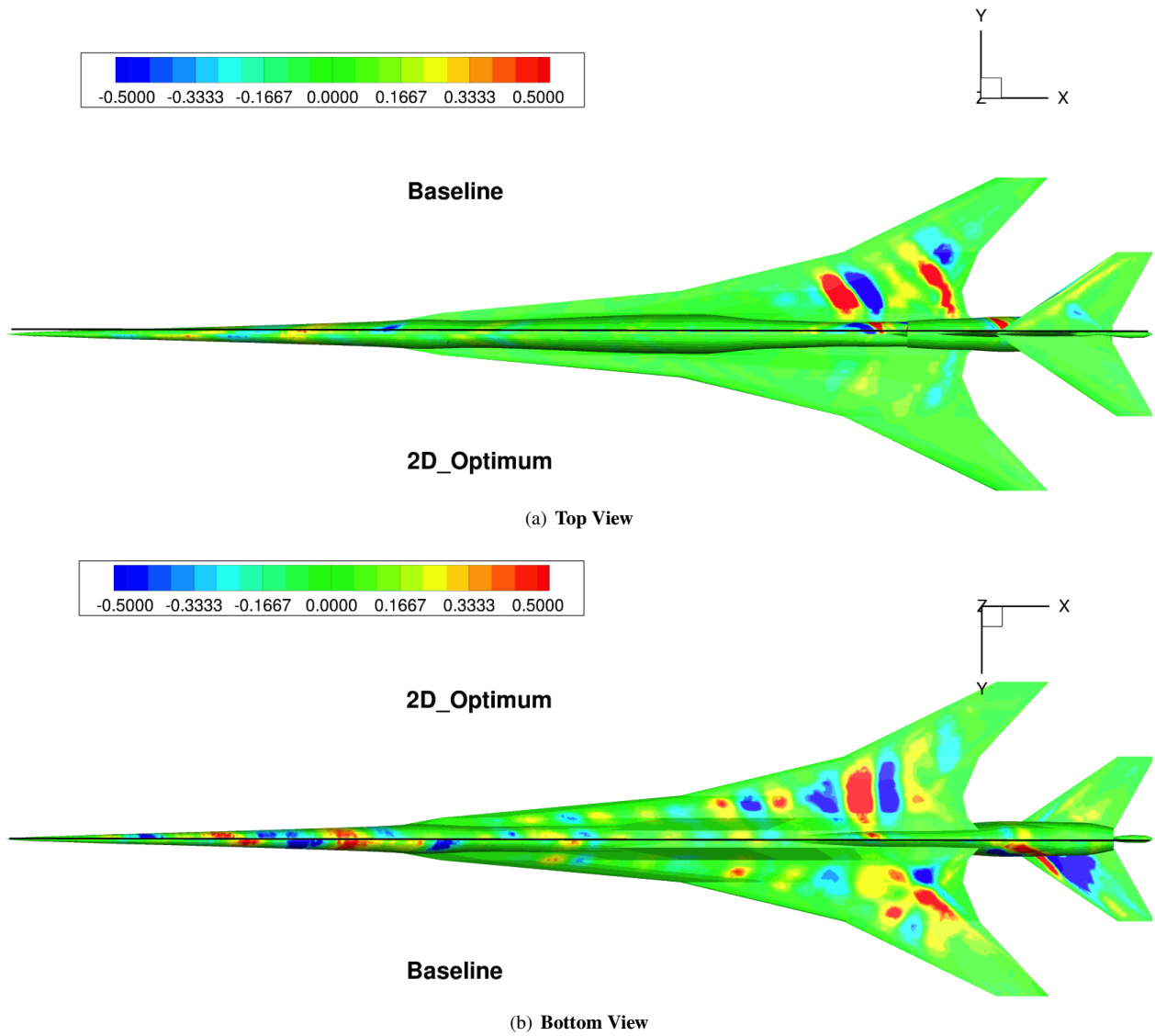
Fig. 17 Optimum loudness sensitivity [d(ASEL)/dn, dB/feet] contours assuming flat Earth
