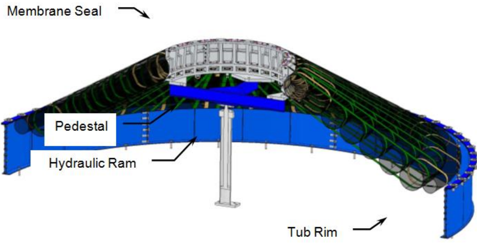
Figure 1- Cutaway view of the 6m HIAD static load test fixture
