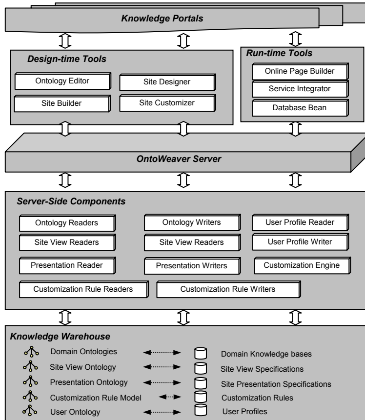
Fig.6. The OntoWeaver-S Architecture
