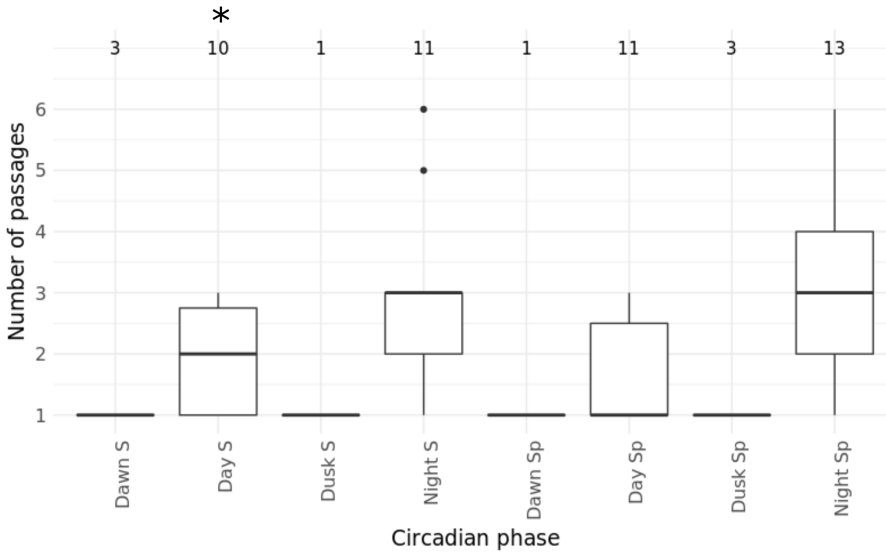
Figure 7.7: The number of shipping lock passages during the four different circadian phases (dawn, day, dusk and night) for the movement classes S and S_p . The number of eels taken into account is indicated above the boxplots. The asterisk indicates a significant difference ( p < 0.05 ) between diurnal and nocturnal passages for S-eels.
