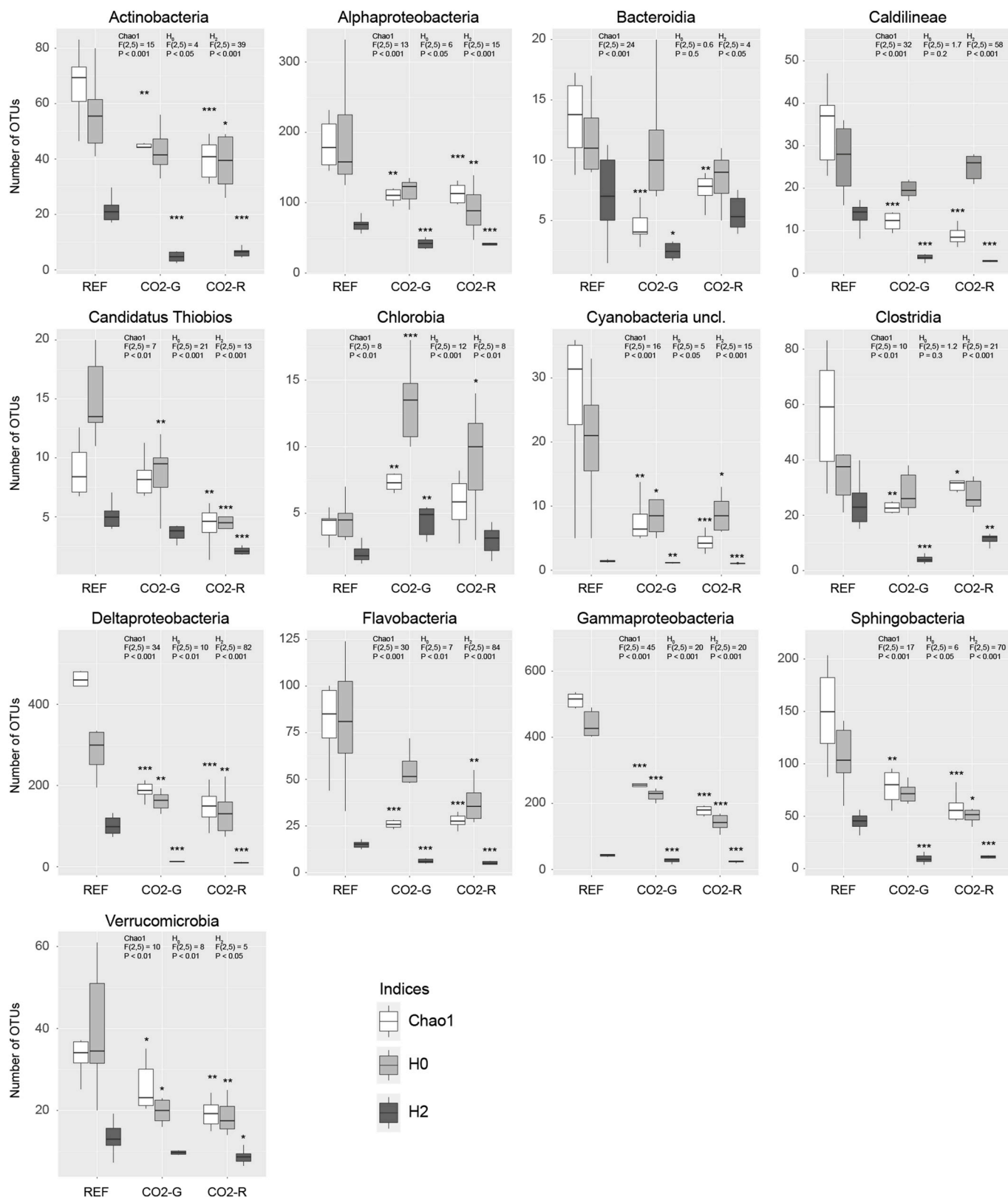
Fig. A.4. Alpha Diversity as described by estimated richness (Chao1) and Hills numbers (H0 and H2) for dominant bacterial classes, based on 454-MPTS data (OTU 0.003 > 0.1%; n = 6; 0–2 cm 4–6 cm layer were combined). Significant difference between the vent sites and the REF are indicated with an asterisk according to pairwise comparison adjusted P values (* < 0.05, ** < 0.01, *** < 0.001). In the plot statistic F-ratio (F), with subscript numbers reporting the degrees of freedom between groups and within groups, respectively, and probability level (P) for total ANOVA model are also reported. Chao1 was calculated based on repeated random subsampling of the 454-MPTS data sets for each class: Actinobacteria = 175 sequences; Alphaproteobacteria = 132 sequences; Bacteroidia = 11 sequences; Caldilineae = 32 sequences; Candidatus Thiobios = 19 sequences; Chlorobia = 15 sequences; Cyanobacteria unclassified (uncl.) = 122 sequences; Clostridia = 32 sequences; Deltaproteobacteria = 470 sequences; Flavobacteria = 185 sequences; Gammaproteobacteria = 860 sequences; Sphingobacteria = 187 sequences;
