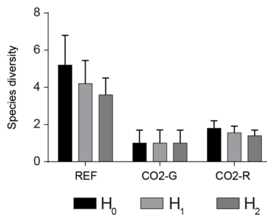
Fig. A.3. Alpha diversity of Polychaeta species (n = 5) expressed in Hill's numbers (H 0 , H 1 , H 2 ) for each study site (REF, CO2-G, CO2-R).
