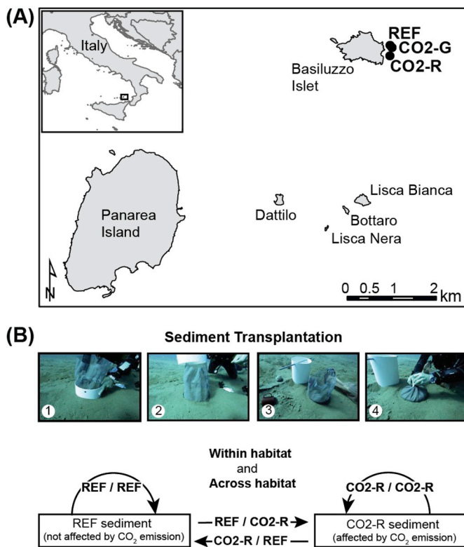
Fig. 1. A) Location of the study area near Basiluzzo Islet (Panarea, Italy), adapted from Guilini et al. (2017b), and B) a scheme illustrating the experimental design of the transplantation experiment. The pictures show (1) how a mesh bag (1.8 mm × 1.6 mm mesh) containing 30 L of sediment was inserted in a TUBO device that was first pushed into the sediments (15 cm depth) and emptied, (2–3) the removal of TUBO and the plastic bag, and (4) the closure of the mesh bags.
