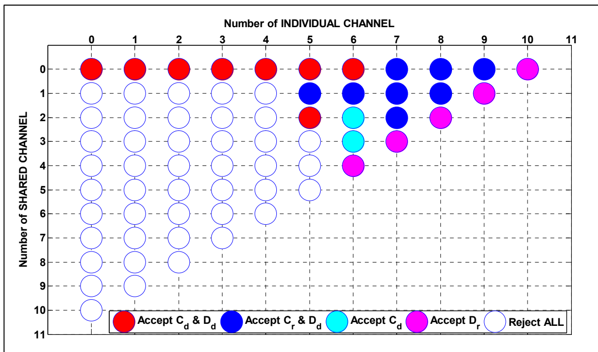
Figure 2.7 Optimal policy for case 3
