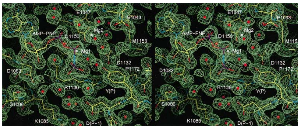
Fig. 1. Electron density map of the active site of IRK3P. Stereo view of a 2F_o - F_c map computed at 1.9 Å resolution and contoured at 1.2 \sigma . Superimposed is the refined atomic model. Carbon atoms are yellow, oxygen atoms red, nitrogen atoms blue, phosphate atoms purple, and sulfur atoms green. The red spheres represent water molecules and the white spheres represent Mg^{2+} ions. Figure prepared with SETOR (Evans, 1993).
