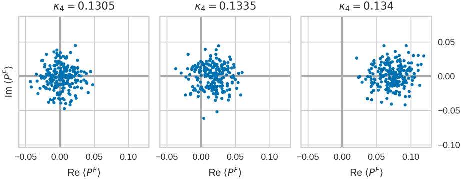
Figure 1. Fundamental Polyakov loops in the complex plane for three different 12^3 \times 6 ensembles on a slice across the transition varying \kappa_4 at constant (\beta, \kappa_6) = (7.4, 0.1285) . Each point is the volume-averaged P^F for one configuration. In the left figure, the points are scattered around 0 and \langle P^F \rangle = 0 . This corresponds to a confined ensemble. The right figure where the points are scattered around a central value on the real axis corresponds to a deconfined ensemble. The ensemble shown in the central panel sits almost directly on top of the confinement transition.
