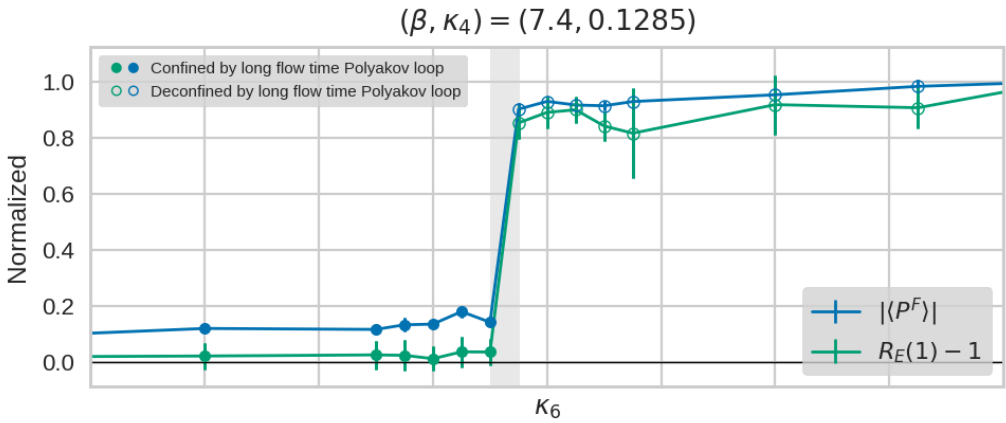
Figure 6. This figure compares the three phase diagnostics used in our study, for the fundamental representation. The diagnostics are plotted as a function of the coupling \kappa_6 for \beta = 7.4 and \kappa_4 = 0.1285 for a 12^3 \times 6 lattice. First: the blue curve denotes the standard Polyakov loop diagnostic. Second: the green curve denotes the “flow anisotropy” diagnostic. Third: the open (closed) circles denote ensembles that are determined to be deconfined (confined) using the “long flow time Polyakov loop” diagnostic. The shaded region denotes the confinement transition. It is clear that the three diagnostics are consistent.
