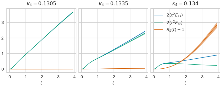
Figure 2. Evolution under Wilson flow of the split flow observables \langle t^2 E_{ss} \rangle and \langle t^2 E_{st} \rangle , depicted for three different 12^3 \times 6 ensembles on a slice at constant (\beta, \kappa_6) = (7.4, 0.1285) . Also depicted is the behavior of R_E - 1 , where R_E \equiv \langle E_{ss}(t) \rangle / \langle E_{st}(t) \rangle . The left panel shows typical confined behavior: the split flow observables are degenerate and R_E = 1 , indicating isotropy. The central panel shows some hints of impending deconfinement: the split flow observables separate slightly, and R_E - 1 becomes nonzero. The right panel shows typical deconfined behavior: the split flow observables break apart, and R_E - 1 grows rapidly in flow time, indicating anisotropy.
