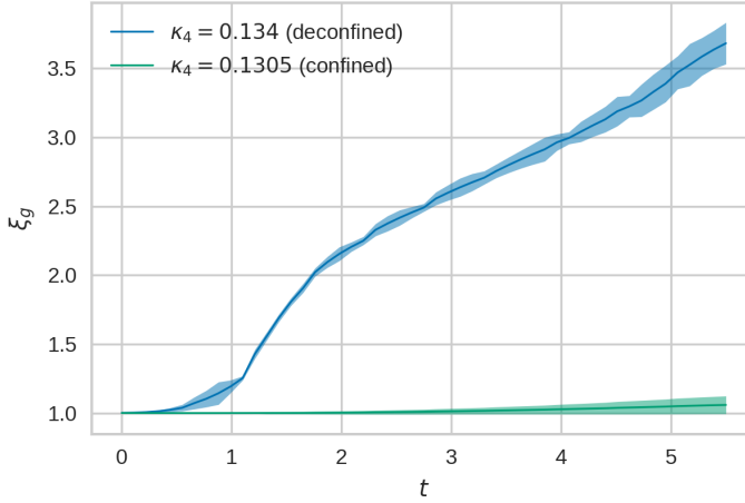
Figure 5. This figure shows a plot of \xi_g = \frac{a_s}{a_t} as a function of flow time t . The blue curve represents the deconfined ensemble shown in the right plot of Fig. 4. It grows monotonically and quite rapidly with t . In the long flow time limit, this behavior implies a_t \rightarrow 0 , which suggests movement towards infinite temperature. The green curve represents the confined ensemble shown in the left plot of Fig. 4. In this case, there is no move towards infinite temperature, at least for the range of flow times we explore.
