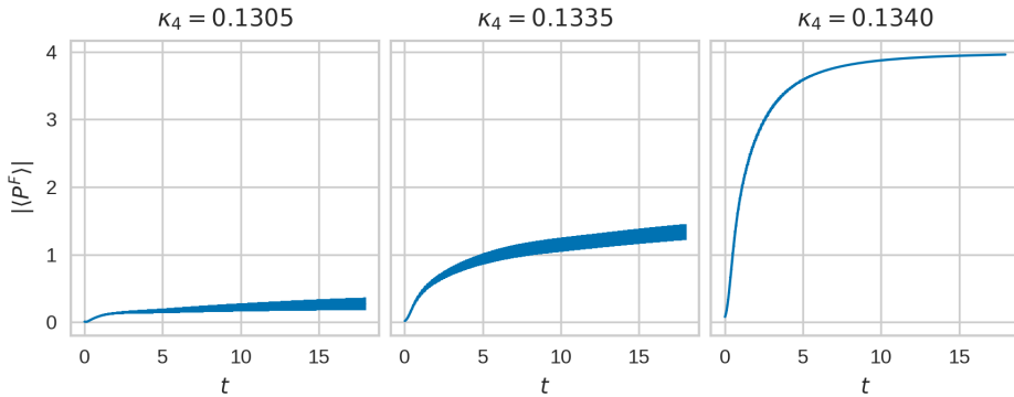
Figure 4. Ensemble-averaged evolution of P^F under Wilson flow, depicted for three different 12^3 \times 6 ensembles on a slice at constant (\beta, \kappa_6) = (7.4, 0.1285) . In the left panel and center panels, we see typical confined behavior: the Polyakov loop either does not increase in magnitude or increases very slowly. In the right panel, we see typical deconfined behavior: the magnitude of Polyakov loop rapidly approaches its maximum value ( \max P^F = d(F) = 4 ). Despite the \kappa_4 values for the centre and right panels being very close, the diagnostic does a very good job of distinguishing the phases.
