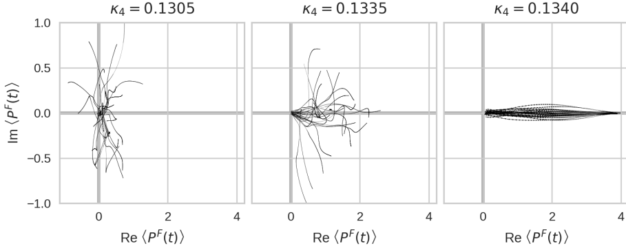
Figure 3. Fundamental Polyakov loops under Wilson flow, depicted for three different 12^3 \times 6 ensembles on a slice at constant (\beta, \kappa_6) = (7.4, 0.1285) . Each panel depicts the complex plane. Each line is the evolution of P^F under Wilson flow on a configuration in the ensemble (i.e., each line is the complex function P^F(t) where t is the flow time). In the two left panels, we see typical confined behavior. In the right panel, we see typical deconfined behavior. The ensemble shown in the central panel sits almost directly on top of the confinement transition.
