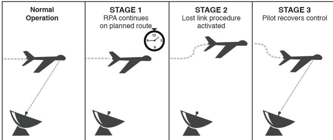
Figure 4. Stages of a lost link event.
