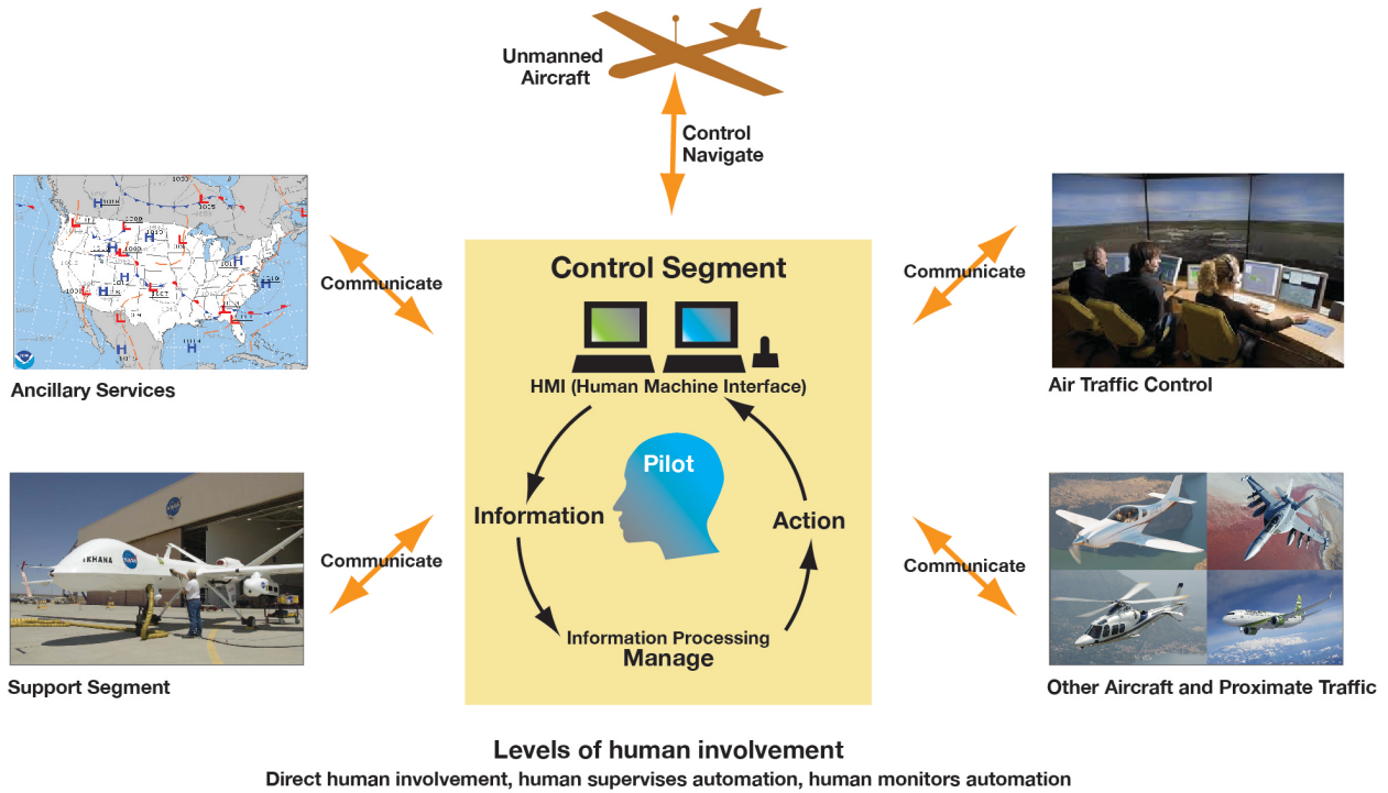
Figure 2. Control and communication responsibilities of a RPAS pilot operating in the NAS.
