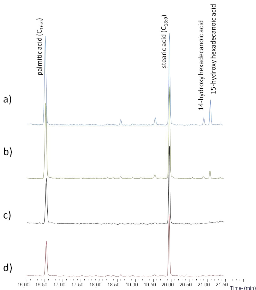
Fig. 4. TIC chromatograms of the aqueous extracted a) R2-np-ua; b) R3-np-ua; c) R4-np-ua; d) R1-np-ua; c) d) without pigment and unaged analysed by GC/MS.
