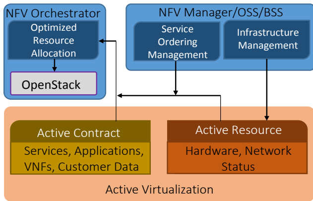
Fig. 2. CloudNFV Architecture
