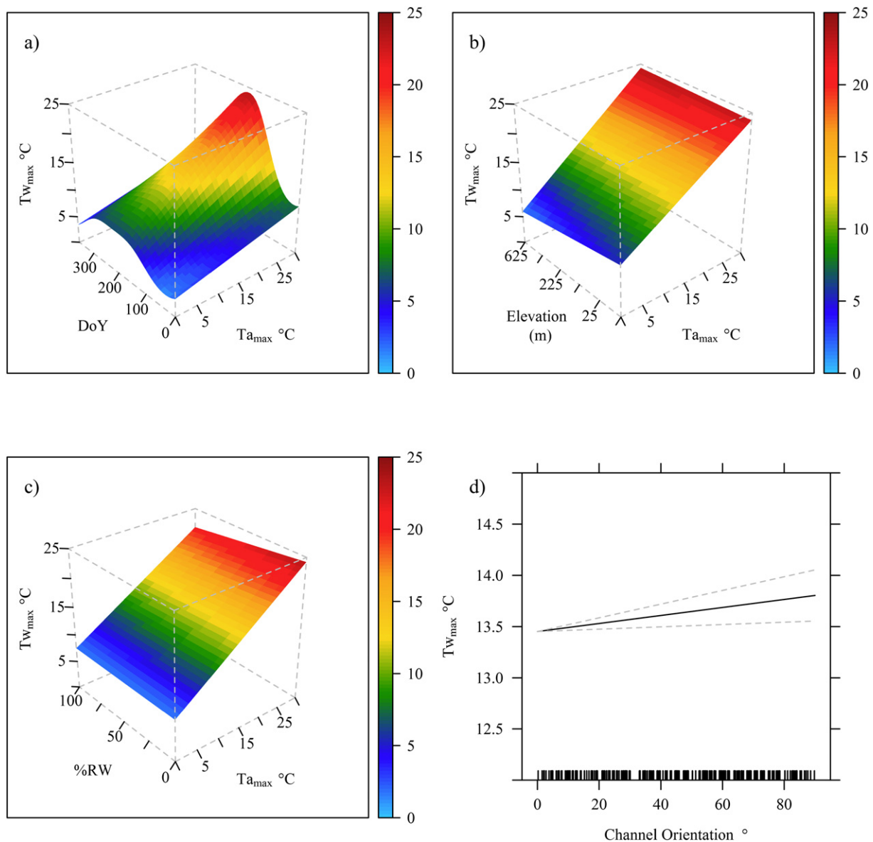
Fig. 3. Joint effects of a) T_{a,max} and DoY, b) T_{a,max} and Elevation, c) T_{a,max} and %RW and the effect of d) Orientation on T_{w,max} . The other covariates are fixed at their median values. Pointwise 95% confidence bands are shown for the Orientation effect. Vertical black lines on the x-axis of the channel orientation plot indicate the presence of data.
