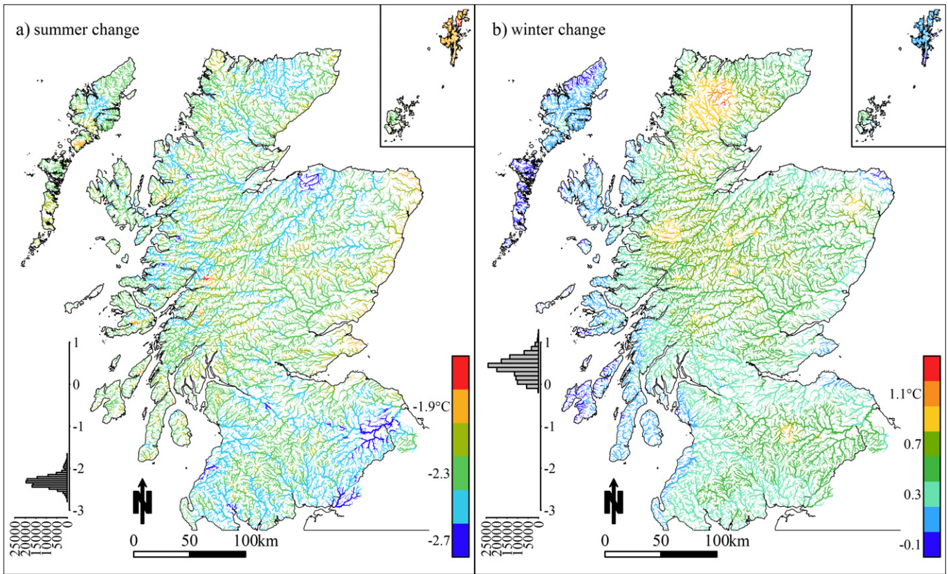
Fig. 8. The predicted change in T_{w,max} when %RW is increased from 0 to 100% in a) summer and b) winter. Plots are conditioned on the hottest and coldest T_{a,max} observed in 2003 and 2010 respectively and the DoY that give the highest and lowest predictions of T_{w,max} (174 and 16 respectively).
