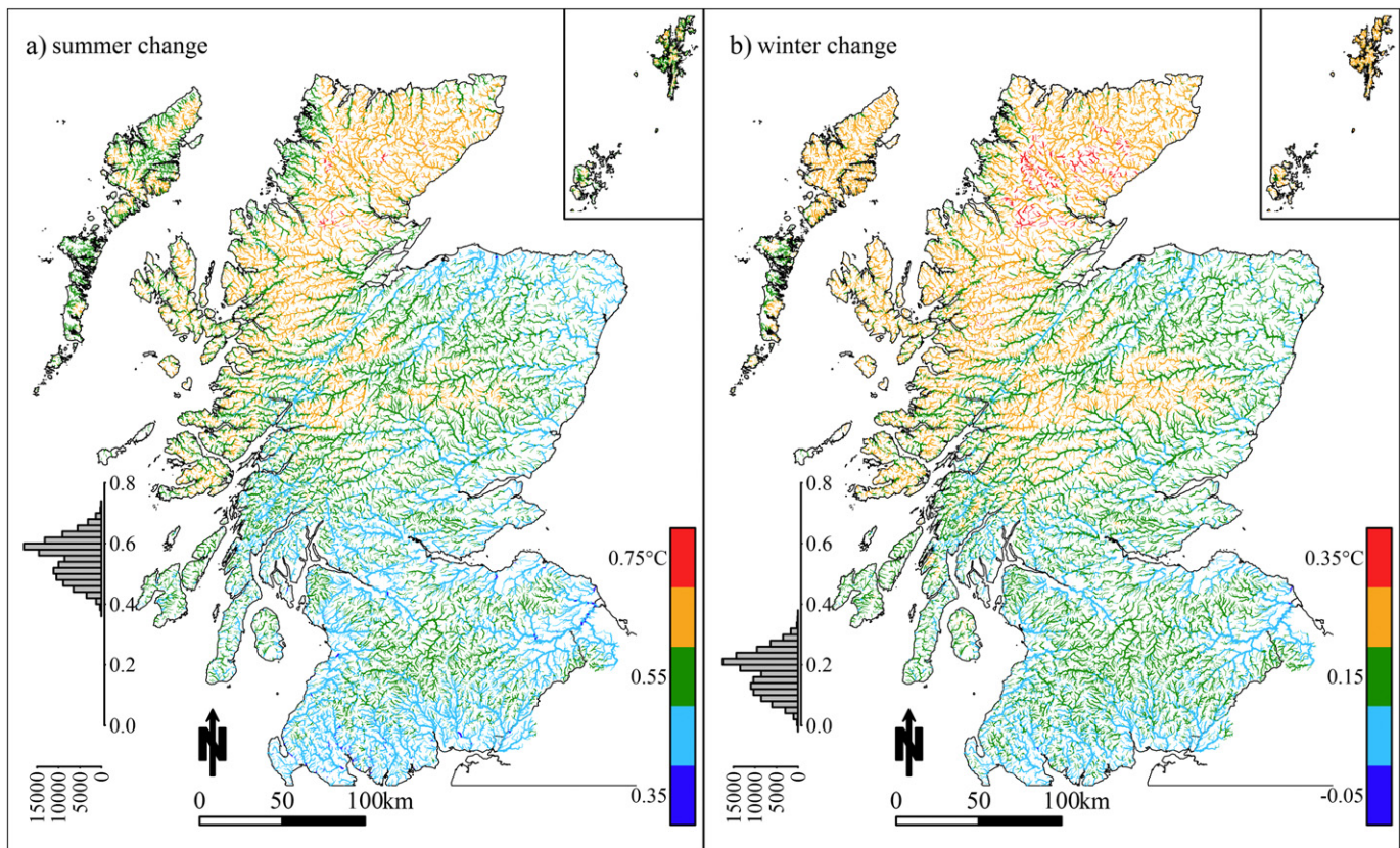
Fig. 7. Sensitivity of rivers to climate change. Maps show the predicted change in T_{w_{max}} for a 1^\circ\text{C} change in T_{a_{max}} in a) summer (DoY 169) and b) winter (DoY 350). The DoYs maximise and minimise the slope of the T_{w_{max}}-T_{a_{max}} relationship respectively.
