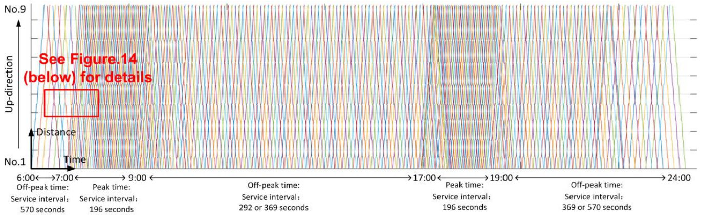
Figure 13. Train running diagram using optimal timetable.
