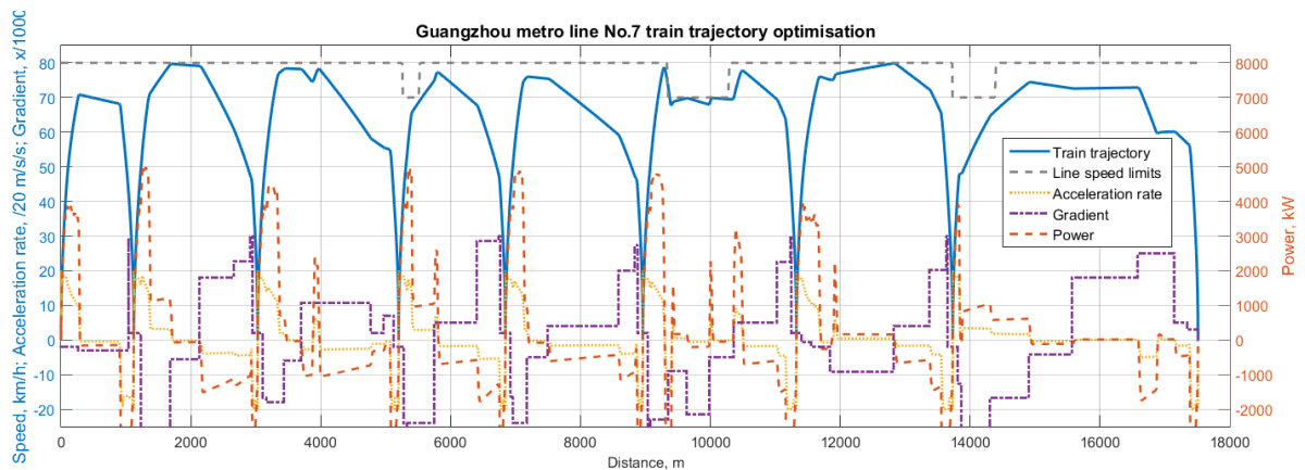
Figure 11. Optimal train trajectory.
