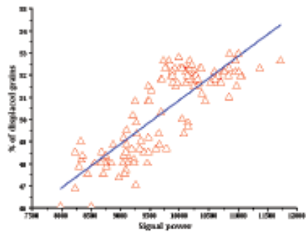
Figure 14 Relation between signal power and percentage of displaced grains (39)
