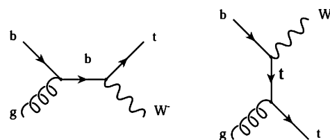
Fig. 1. Leading-order Feynman diagrams for associated production of a single top-quark and a W boson.
