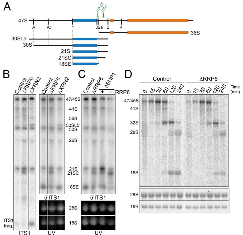
Figure 2. RRP6 is required for ITS1 processing. (A) Schematic representation of the 47S pre-rRNA intermediate and relevant pre-rRNAs. The relative positions of Northern blot probes are indicated. (B and C) RNA was extracted from HeLa cells depleted of RRP6, XRN2, or ENP1 by RNAi or control cells and analyzed by ethidium bromide staining (UV) and Northern hybridization using probes specific to the 5' end and middle of ITS1 as indicated. Positions of the various intermediates detected are indicated. (D) HeLa cells depleted of RRP6, or control cells, were pulse labeled with ^3\text{H} methyl-methionine followed by incubation in normal media for varying lengths of time (indicated above each lane). RNA was recovered from the cells, separated using glyoxal/agarose gel electrophoresis, and visualized using a phosphorimager and ethidium bromide staining (UV). The control data are repeated in Fig. 6 E. Black lines in B indicate intervening lanes that have been removed.
