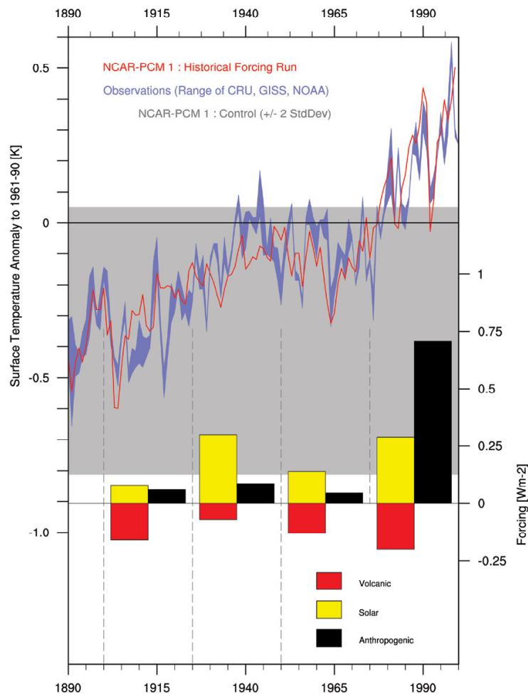
Figure 2.2 A modelled global surface temperature (red line) from 1890-2000 compared to observations (blue area, the width denotes the precision). The averaged volcanic, solar and anthropogenic climate forcings are indicated by the underlying histogram.
