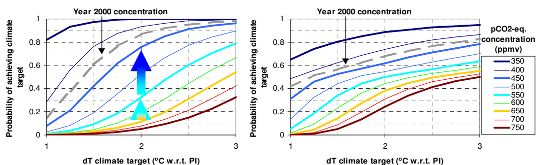
Figure 5.5 Probability of achieving a temperature target for a range of \text{CO}_2 -eq. stabilization levels.
